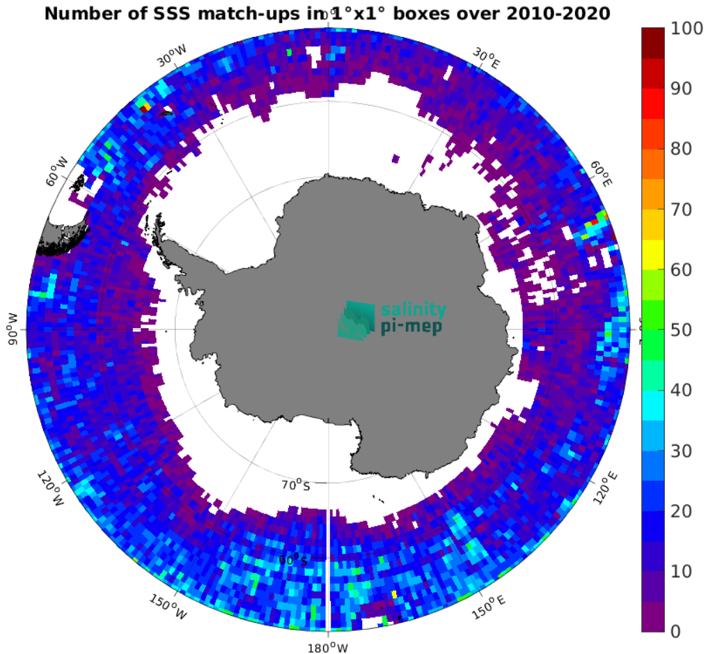
Figure 4: Number of SSS match-ups between Argo SSS and the CCI SSS L4 Merged-OI v3.2 - 7-day running (ESA) SSS product for the Southern Ocean Pi-MEP region over 1^\circ \times 1^\circ boxes and for the full satellite product period.
