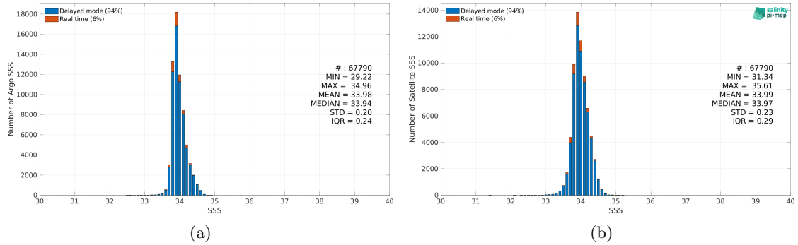
Figure 2: Histograms of SSS from Argo (a) and CCI SSS L4 Merged-OI v3.2 - 7-day running (ESA) (b) considering all match-up pairs per bins of 0.1 over the Southern Ocean Pi-MEP region and for the full satellite product period.
