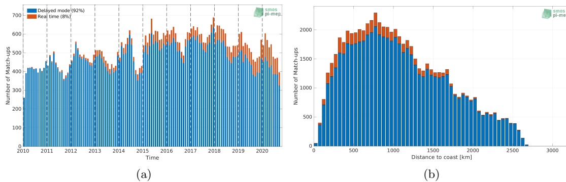
Figure 1: Number of match-ups between Argo and CCI SSS L4 Merged-OI v3.2 - 7-day running (ESA) SSS as a function of time (a) and as function of the distance to coast (b) over the Southern Ocean Pi-MEP region and for the full satellite product period.
