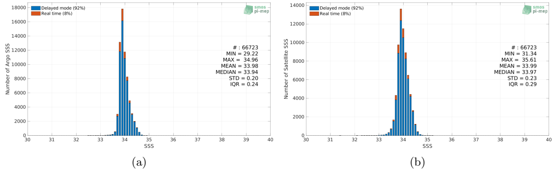
Figure 2: Histograms of SSS from Argo (a) and CCI SSS L4 Merged-OI v3.2 - 7-day running (ESA) (b) considering all match-up pairs per bins of 0.1 over the Southern Ocean Pi-MEP region and for the full satellite product period.
