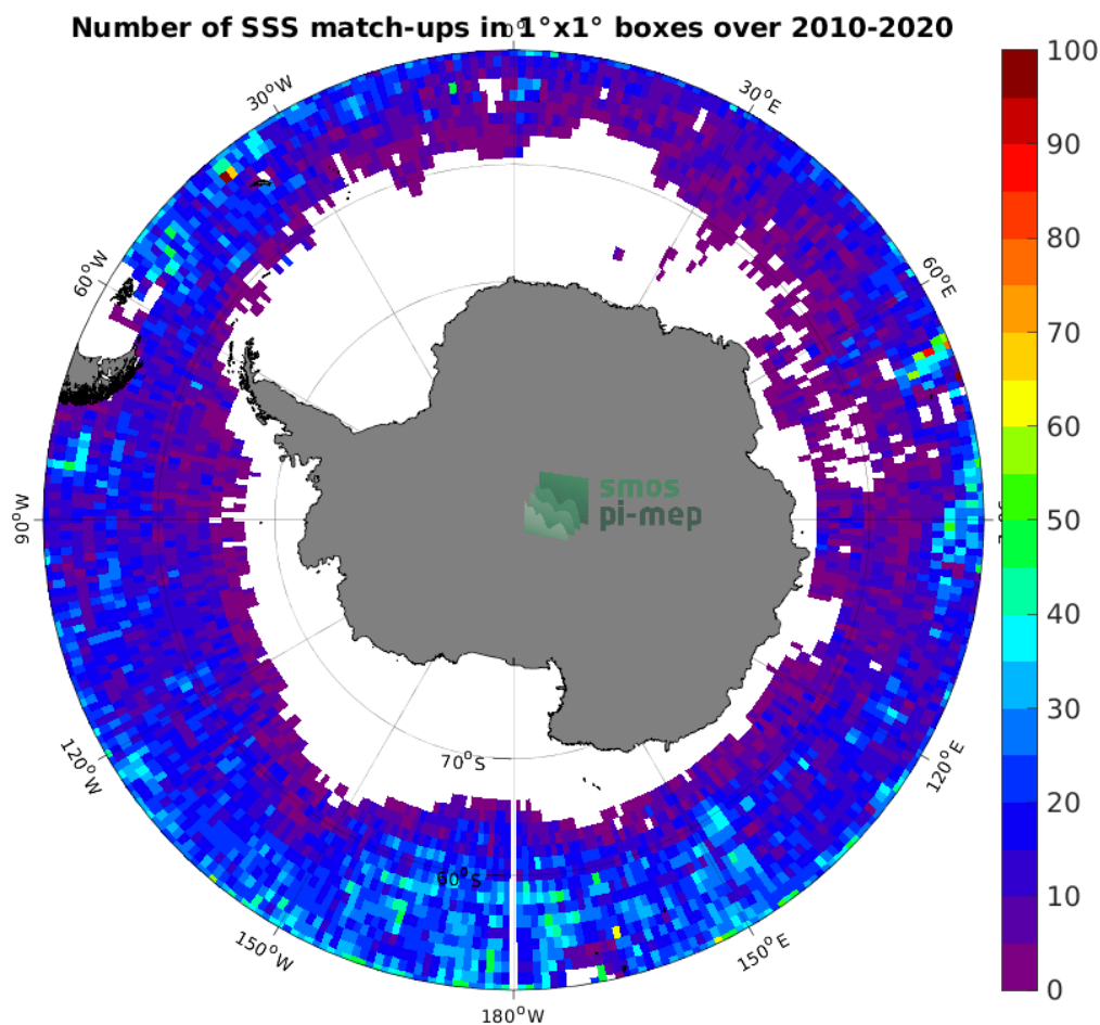
Figure 4: Number of SSS match-ups between Argo SSS and the CCI SSS L4 Merged-OI v3.2 - 7-day running (ESA) SSS product for the Southern Ocean Pi-MEP region over 1^\circ \times 1^\circ boxes and for the full satellite product period.
