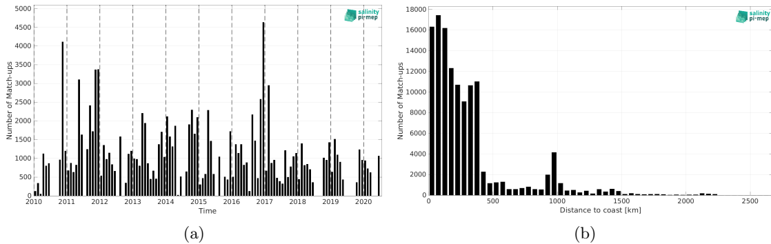
Figure 1: Number of match-ups between TSG (SAMOS) and CCI SSS L4 Merged-OI v3.2 - 30-day running (ESA) SSS as a function of time (a) and as function of the distance to coast (b) over the Southern Ocean Pi-MEP region and for the full satellite product period.
