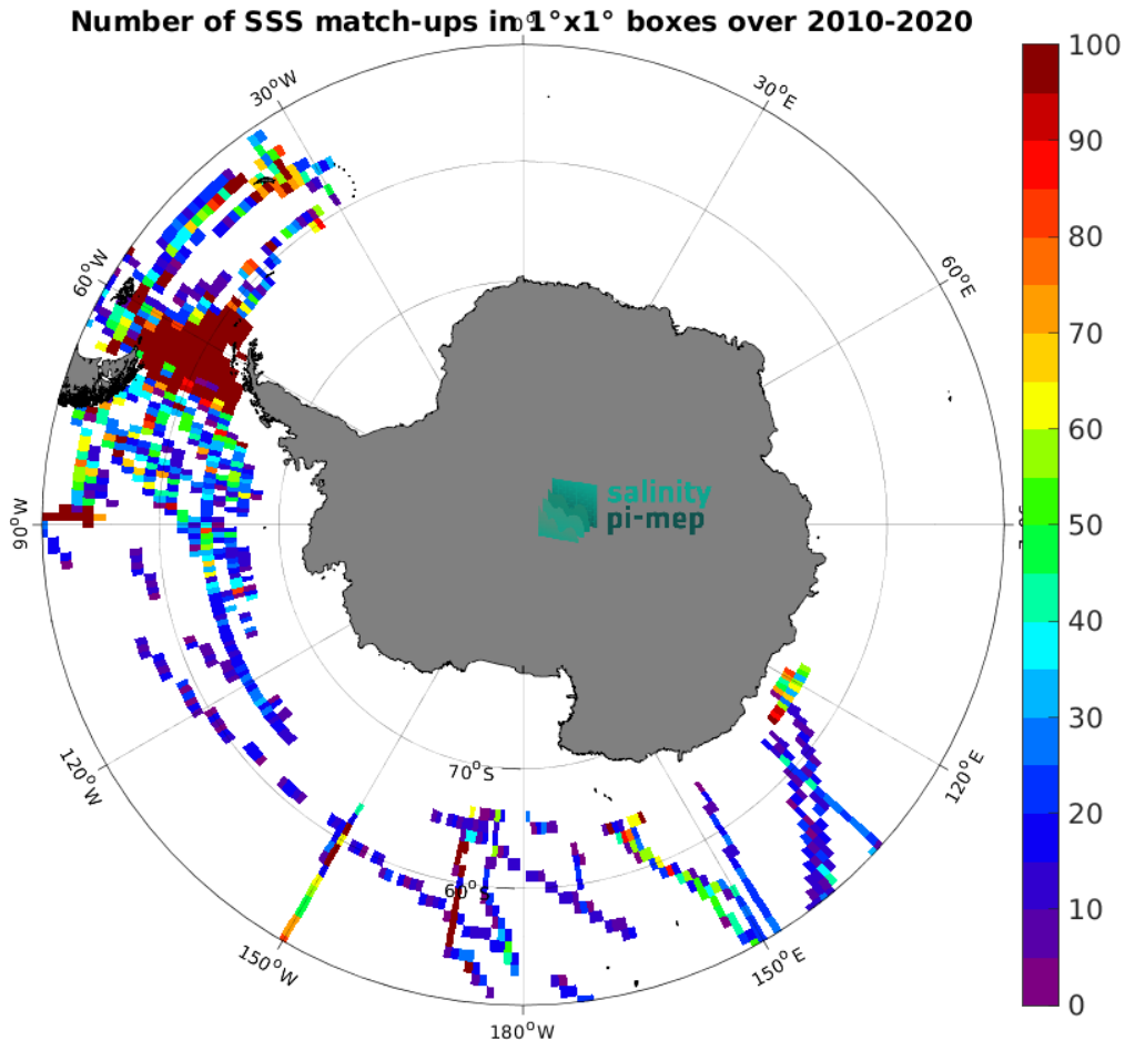
Figure 4: Number of SSS match-ups between TSG (SAMOS) SSS and the CCI SSS L4 Merged-OI v3.2 - 30-day running (ESA) SSS product for the Southern Ocean Pi-MEP region over 1^\circ \times 1^\circ boxes and for the full satellite product period.
