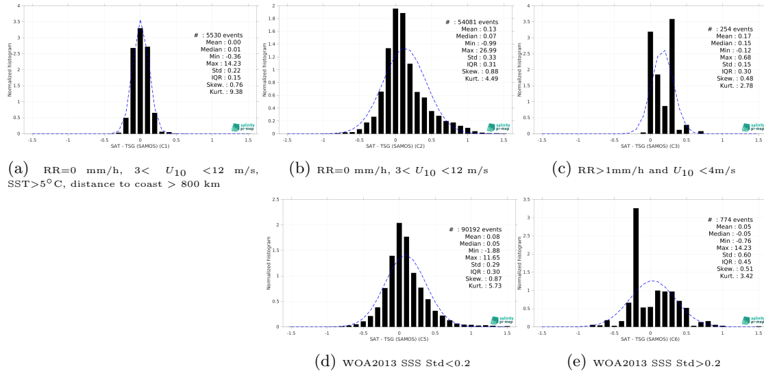
Figure 13: Normalized histogram of \Delta\text{SSS} (CCI SSS L4 Merged-OI v3.2 - 30-day running (ESA) - TSG (SAMOS)) for 5 different subdatasets corresponding to: RR=0 mm/h, 3 < U_{10} < 12 m/s, SST>5°C, distance to coast > 800 km (a), RR=0 mm/h, 3 < U_{10} < 12 m/s (b), RR>1mm/h and U_{10} < 4 m/s (c), WOA2013 SSS Std<0.2 (d), WOA2013 SSS Std>0.2 (e).
