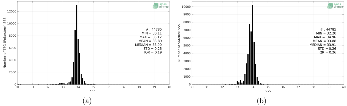
Figure 2: Histograms of SSS from TSG (Polarstern) (a) and CCI SSS L4 Merged-OI v3.2 - 30-day running (ESA) (b) considering all match-up pairs per bins of 0.1 over the Southern Ocean Pi-MEP region and for the full satellite product period.
