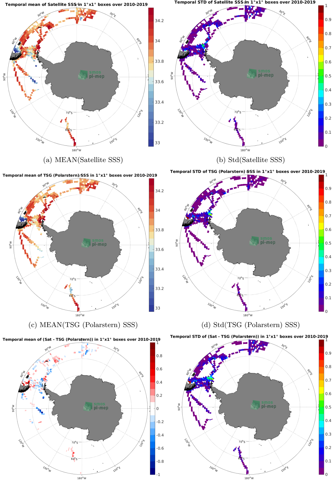
Figure 6: Temporal mean (left) and Std (right) of SSS from CCI SSS L4 Merged-OI v3.2 - 30-day running (ESA) (top), TSG (Polarstern) (middle), and of \Delta SSS (Satellite - TSG (Polarstern)). Only match-up pairs are used to generate these maps.
