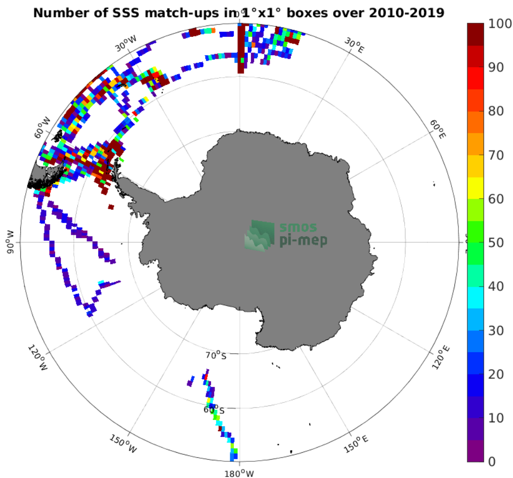
Figure 4: Number of SSS match-ups between TSG (Polarstern) SSS and the CCI SSS L4 Merged-OI v3.2 - 30-day running (ESA) SSS product for the Southern Ocean Pi-MEP region over 1^\circ \times 1^\circ boxes and for the full satellite product period.
