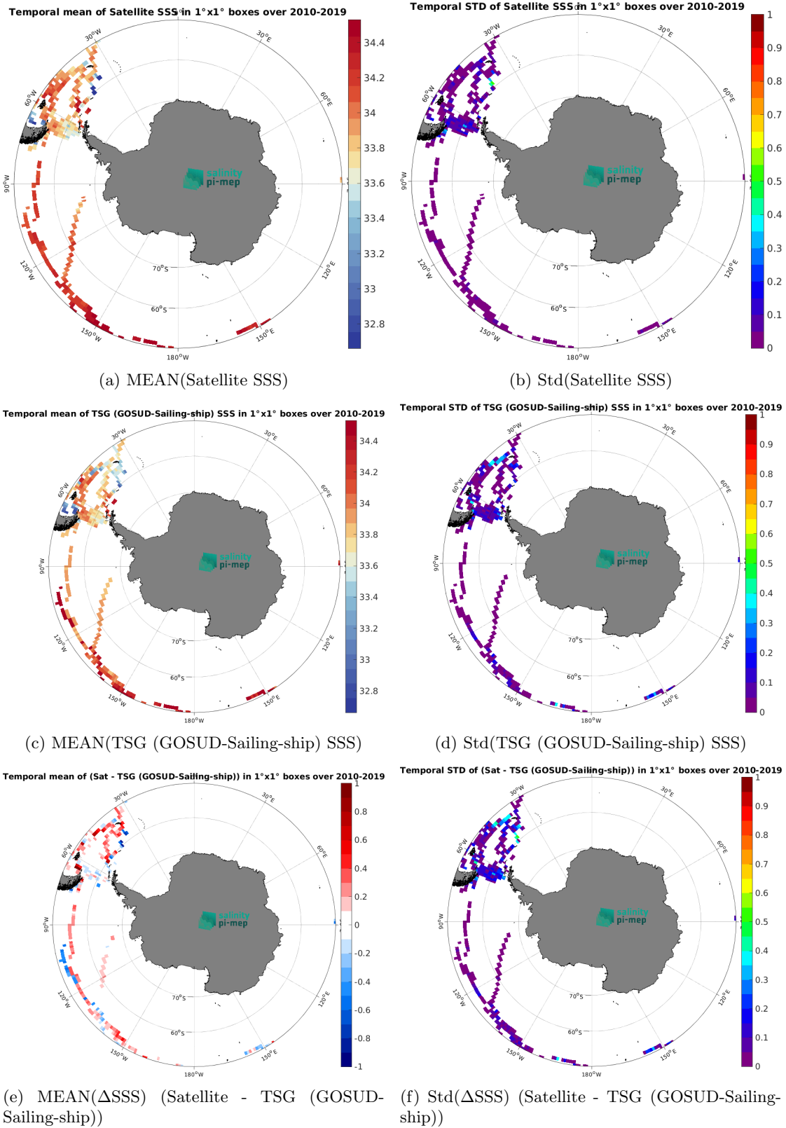
Figure 6: Temporal mean (left) and Std (right) of SSS from CCI SSS L4 Merged-OI v3.2 - 30-day running (ESA) (top), TSG (GOSUD-Sailing-ship) (middle), and of \Delta SSS (Satellite - TSG (GOSUD-Sailing-ship)). Only match-up pairs are used to generate these maps.
