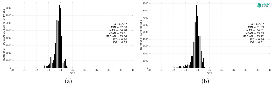
Figure 2: Histograms of SSS from TSG (GOSUD-Sailing-ship) (a) and CCI SSS L4 Merged-OI v3.2 - 30-day running (ESA) (b) considering all match-up pairs per bins of 0.1 over the Southern Ocean Pi-MEP region and for the full satellite product period.
