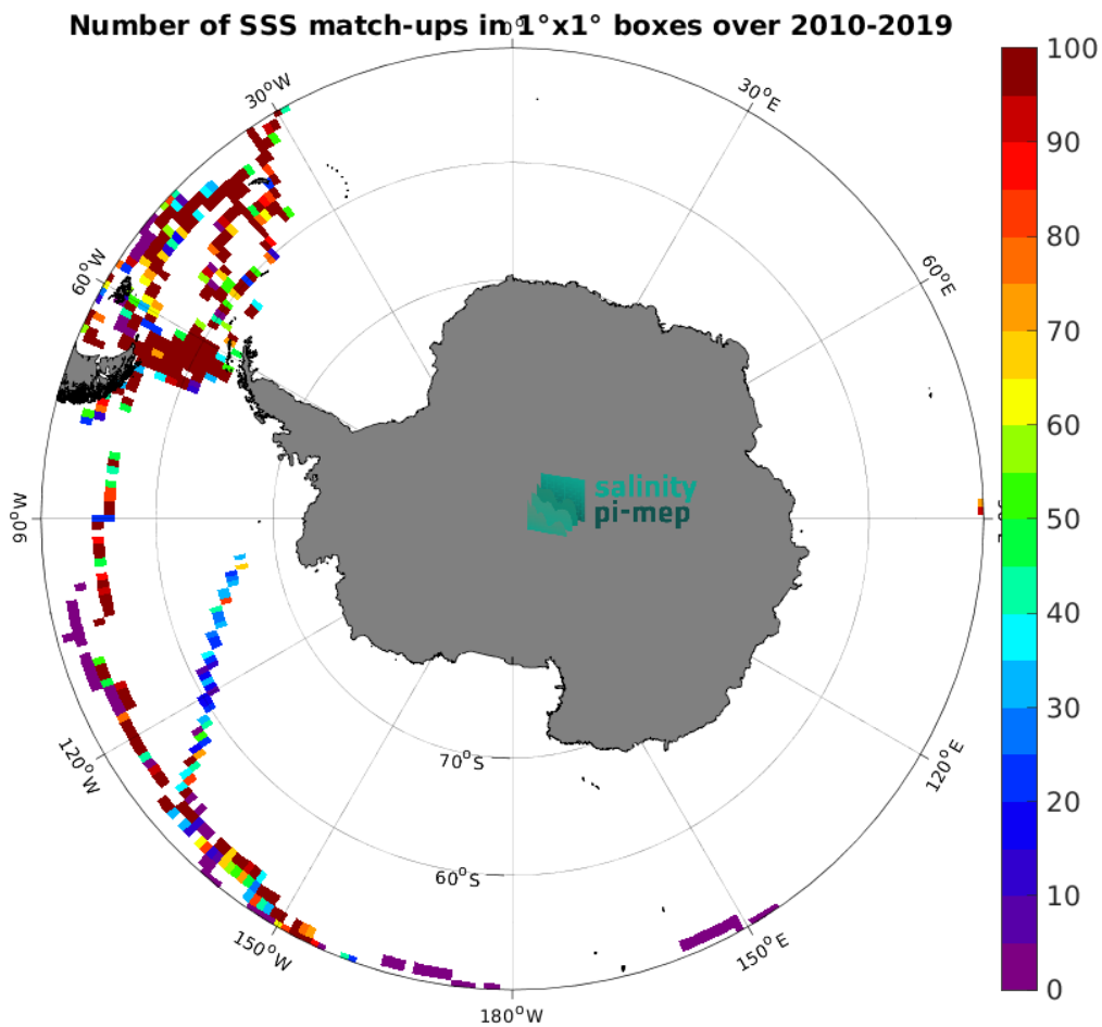
Figure 4: Number of SSS match-ups between TSG (GOSUD-Sailing-ship) SSS and the CCI SSS L4 Merged-OI v3.2 - 30-day running (ESA) SSS product for the Southern Ocean Pi-MEP region over 1^\circ \times 1^\circ boxes and for the full satellite product period.
