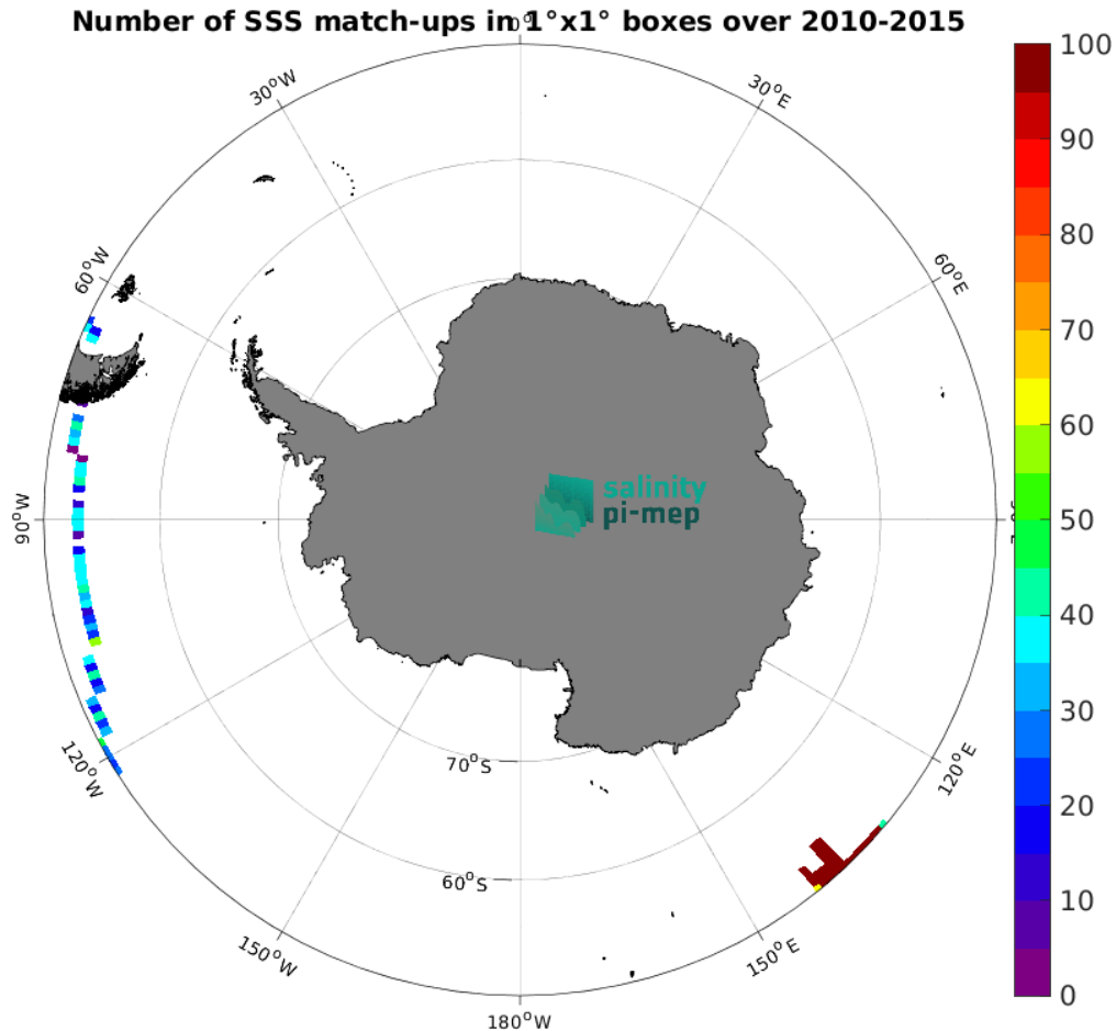
Figure 4: Number of SSS match-ups between TSG (GOSUD-Research-vessel) SSS and the CCI SSS L4 Merged-OI v3.2 - 30-day running (ESA) SSS product for the Southern Ocean Pi-MEP region over 1^\circ \times 1^\circ boxes and for the full satellite product period.
