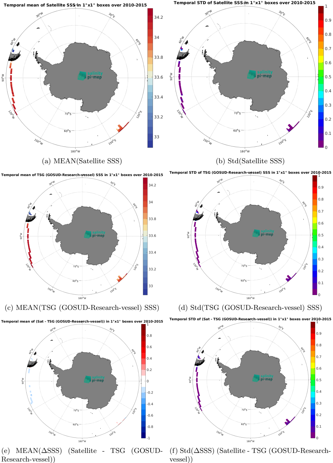
Figure 6: Temporal mean (left) and Std (right) of SSS from CCI SSS L4 Merged-OI v3.2 - 30-day running (ESA) (top), TSG (GOSUD-Research-vessel) (middle), and of \Delta SSS (Satellite - TSG (GOSUD-Research-vessel)). Only match-up pairs are used to generate these maps.
