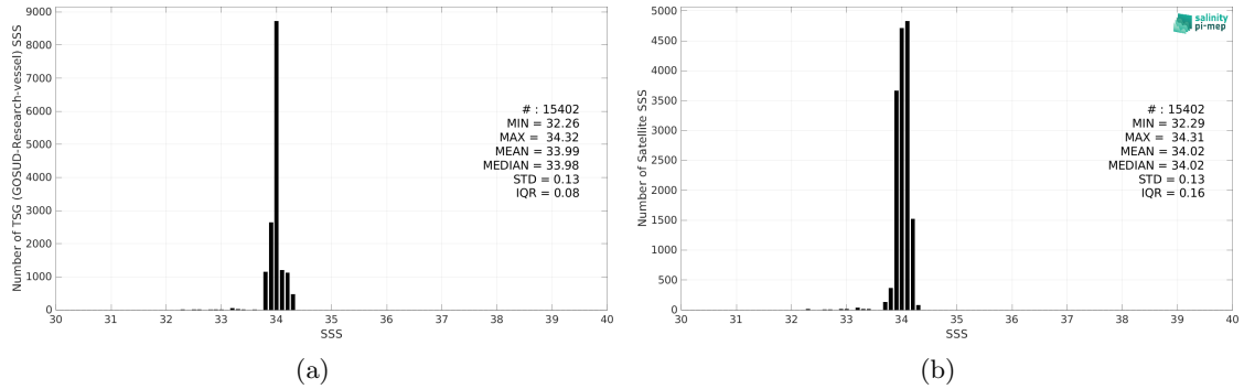
Figure 2: Histograms of SSS from TSG (GOSUD-Research-vessel) (a) and CCI SSS L4 Merged-OI v3.2 - 30-day running (ESA) (b) considering all match-up pairs per bins of 0.1 over the Southern Ocean Pi-MEP region and for the full satellite product period.
