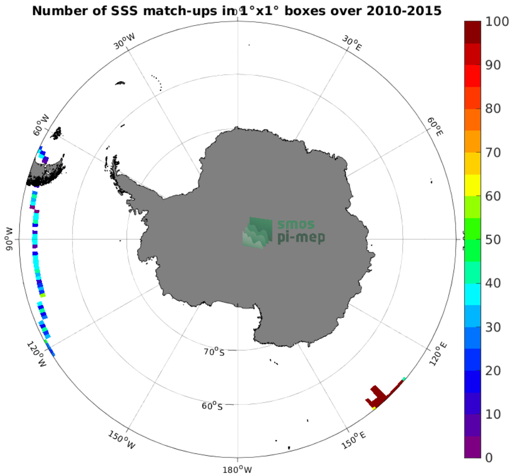
Figure 4: Number of SSS match-ups between TSG (GOSUD-Research-vessel) SSS and the CCI SSS L4 Merged-OI v3.2 - 30-day running (ESA) SSS product for the Southern Ocean Pi-MEP region over 1^\circ \times 1^\circ boxes and for the full satellite product period.
