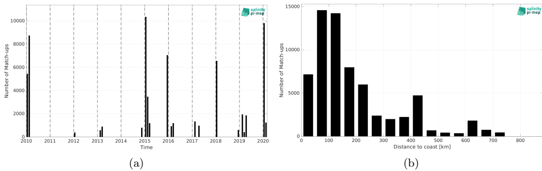
Figure 1: Number of match-ups between TSG (CSIC-UTM) and CCI SSS L4 Merged-OI v3.2 - 30-day running (ESA) SSS as a function of time (a) and as function of the distance to coast (b) over the Southern Ocean Pi-MEP region and for the full satellite product period.
