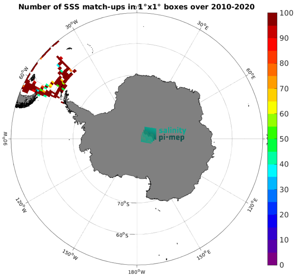
Figure 4: Number of SSS match-ups between TSG (CSIC-UTM) SSS and the CCI SSS L4 Merged-OI v3.2 - 30-day running (ESA) SSS product for the Southern Ocean Pi-MEP region over 1^\circ \times 1^\circ boxes and for the full satellite product period.
