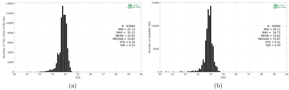
Figure 2: Histograms of SSS from TSG (CSIC-UTM) (a) and CCI SSS L4 Merged-OI v3.2 - 30-day running (ESA) (b) considering all match-up pairs per bins of 0.1 over the Southern Ocean Pi-MEP region and for the full satellite product period.
