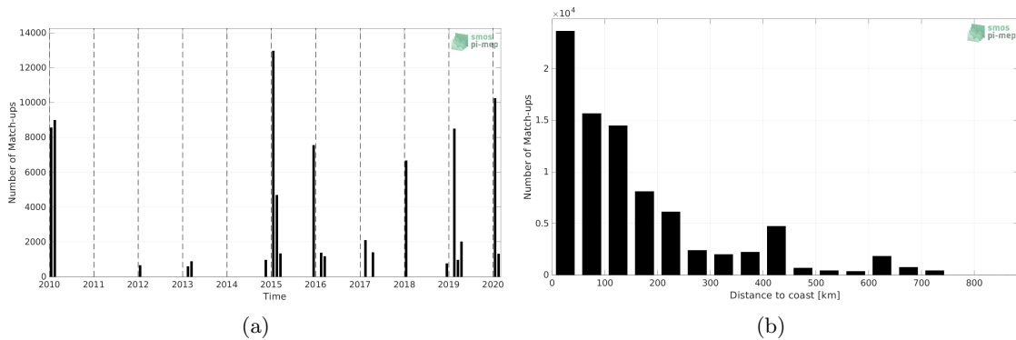
Figure 1: Number of match-ups between TSG (CSIC-UTM) and CCI SSS L4 Merged-OI v3.2 - 30-day running (ESA) SSS as a function of time (a) and as function of the distance to coast (b) over the Southern Ocean Pi-MEP region and for the full satellite product period.
