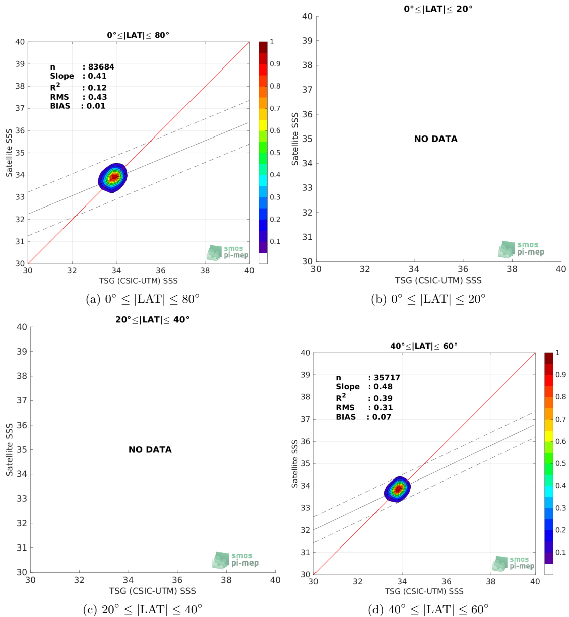
Figure 9: Contour maps of the concentration of CCI SSS L4 Merged-OI v3.2 - 30-day running (ESA) SSS (y-axis) versus TSG (CSIC-UTM) SSS (x-axis) at match-up pairs for different latitude bands. For each plot, the red line shows x=y . The black thin and dashed lines indicate a linear fit through the data cloud and the \pm 95\% confidence levels, respectively. The number match-up pairs n , the slope and R^2 coefficient of the linear fit, the root mean square (RMS) and the mean bias between satellite and in situ data are indicated for each latitude band in each plots.
