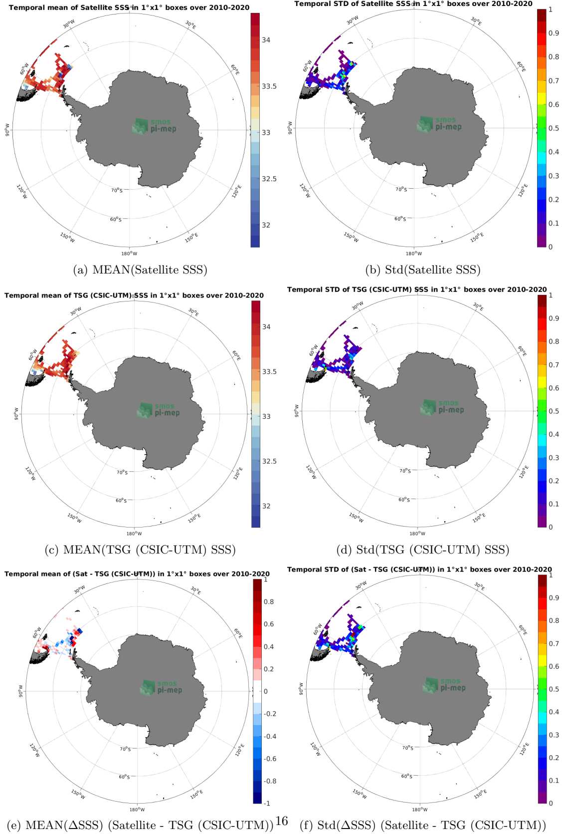
Figure 6: Temporal mean (left) and Std (right) of SSS from CCI SSS L4 Merged-OI v3.2 - 30-day running (ESA) (top), TSG (CSIC-UTM) (middle), and of \Delta SSS (Satellite - TSG (CSIC-UTM)). Only match-up pairs are used to generate these maps.
