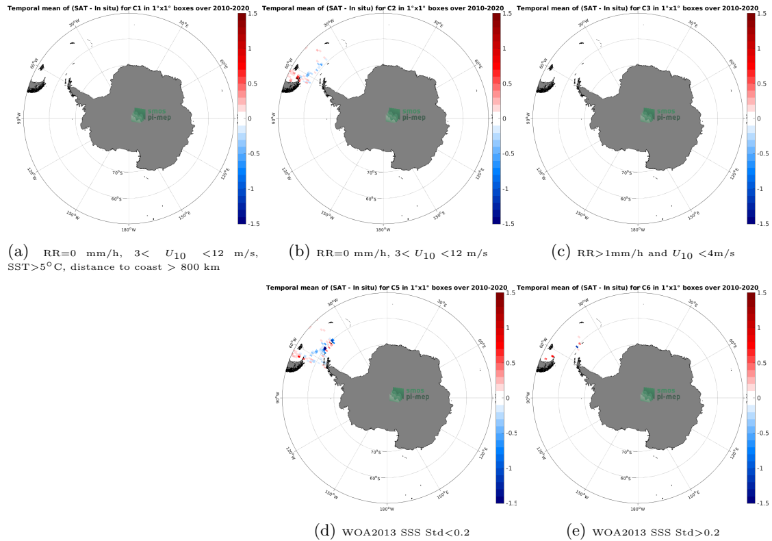
Figure 12: Temporal mean gridded over spatial boxes of size 1^{\circ}\times 1^{\circ} of \Delta\text{SSS} (CCI SSS L4 Merged-OI v3.2 - 30-day running (ESA) - TSG (CSIC-UTM)) for 5 different subdatasets corresponding to:RR=0 mm/h, 3 < U_{10} < 12 m/s, SST >5^{\circ}\text{C} , distance to coast > 800 km (a), RR=0 mm/h, 3 < U_{10} < 12 m/s (b), RR >1 mm/h and U_{10} < 4 m/s (c), WOA2013 SSS Std <0.2 (d), WOA2013 SSS Std >0.2 (e).
