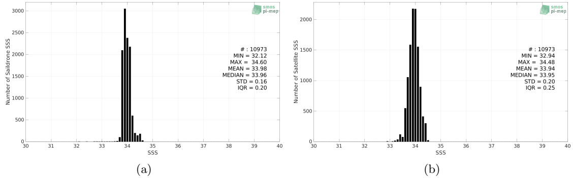
Figure 2: Histograms of SSS from Saildrone (a) and CCI SSS L4 Merged-OI v3.2 - 30-day running (ESA) (b) considering all match-up pairs per bins of 0.1 over the Southern Ocean Pi-MEP region and for the full satellite product period.
