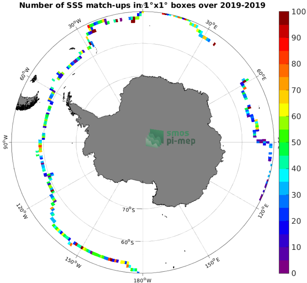
Figure 4: Number of SSS match-ups between Saildrone SSS and the CCI SSS L4 Merged-OI v3.2 - 30-day running (ESA) SSS product for the Southern Ocean Pi-MEP region over 1^\circ \times 1^\circ boxes and for the full satellite product period.
