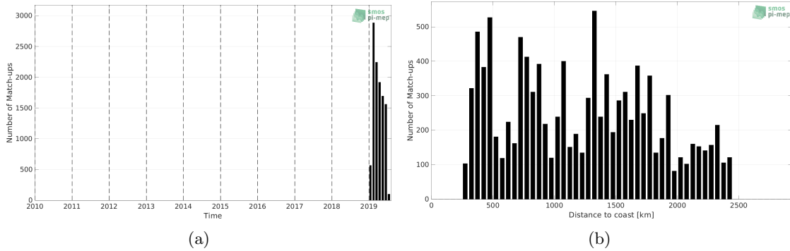
Figure 1: Number of match-ups between Saildrone and CCI SSS L4 Merged-OI v3.2 - 30-day running (ESA) SSS as a function of time (a) and as function of the distance to coast (b) over the Southern Ocean Pi-MEP region and for the full satellite product period.
