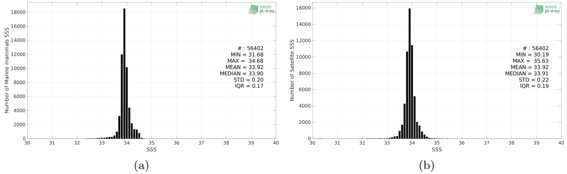
Figure 2: Histograms of SSS from Marine mammals (a) and CCI SSS L4 Merged-OI v3.2 - 30-day running (ESA) (b) considering all match-up pairs per bins of 0.1 over the Southern Ocean Pi-MEP region and for the full satellite product period.
