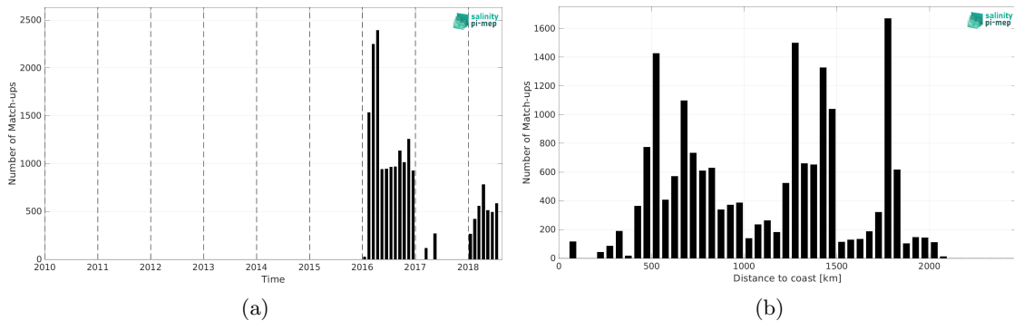
Figure 1: Number of match-ups between Surface drifters and CCI SSS L4 Merged-OI v3.2 - 30-day running (ESA) SSS as a function of time (a) and as function of the distance to coast (b) over the Southern Ocean Pi-MEP region and for the full satellite product period.
