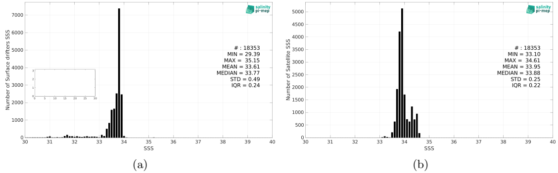
Figure 2: Histograms of SSS from Surface drifters (a) and CCI SSS L4 Merged-OI v3.2 - 30-day running (ESA) (b) considering all match-up pairs per bins of 0.1 over the Southern Ocean Pi-MEP region and for the full satellite product period.
