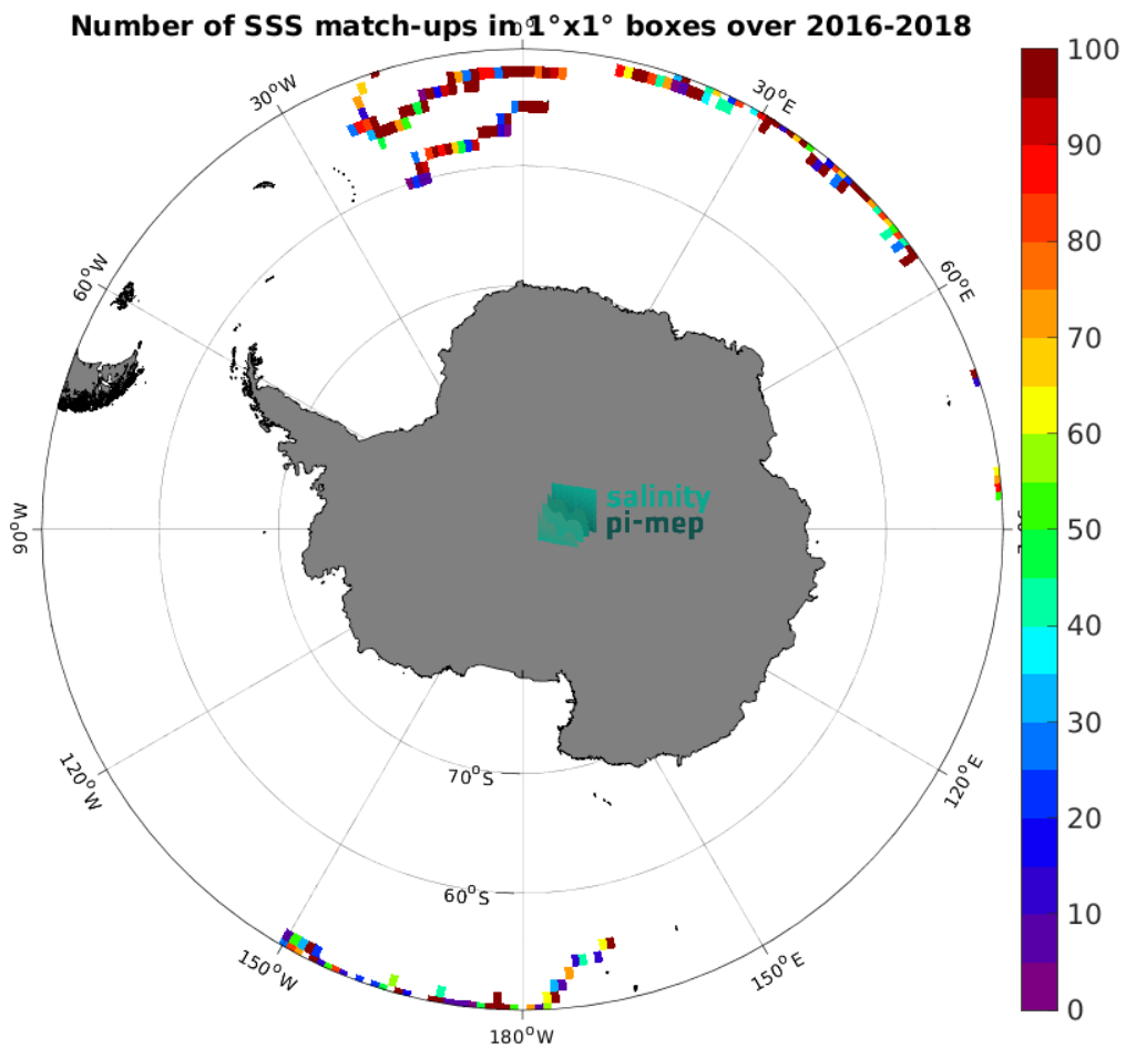
Figure 3: Number of SSS match-ups between Surface drifters SSS and the CCI SSS L4 Merged-OI v3.2 - 30-day running (ESA) SSS product for the Southern Ocean Pi-MEP region over 1^\circ \times 1^\circ boxes and for the full satellite product period.
