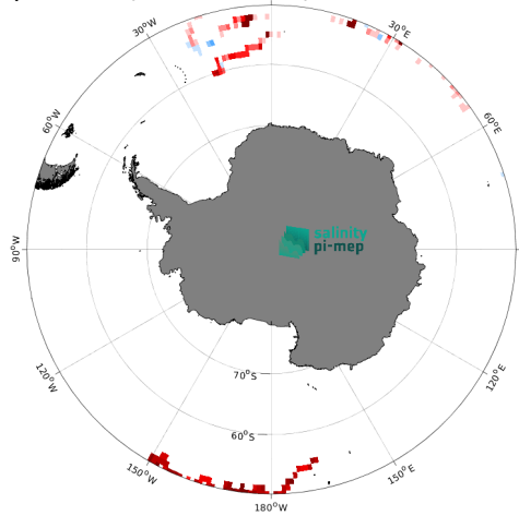
(e) MEAN( \Delta SSS) (Satellite - Surface drifters) 15
