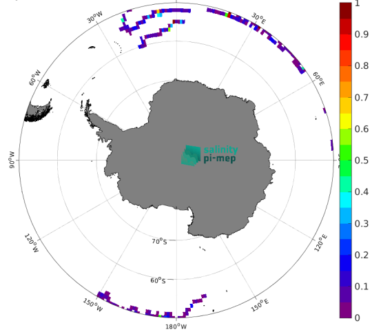
(e) MEAN( \Delta SSS) (Satellite - Surface drifters) 15
