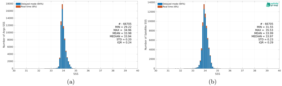
Figure 2: Histograms of SSS from Argo (a) and CCI SSS L4 Merged-OI v3.2 - 30-day running (ESA) (b) considering all match-up pairs per bins of 0.1 over the Southern Ocean Pi-MEP region and for the full satellite product period.
