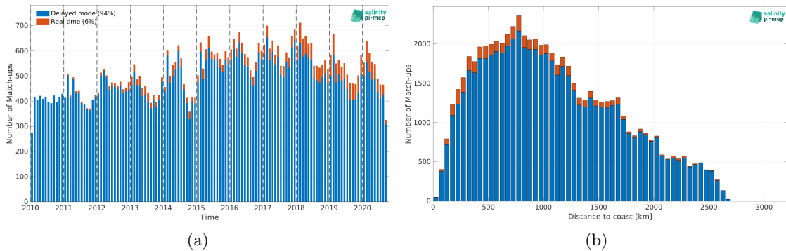
Figure 1: Number of match-ups between Argo and CCI SSS L4 Merged-OI v3.2 - 30-day running (ESA) SSS as a function of time (a) and as function of the distance to coast (b) over the Southern Ocean Pi-MEP region and for the full satellite product period.
