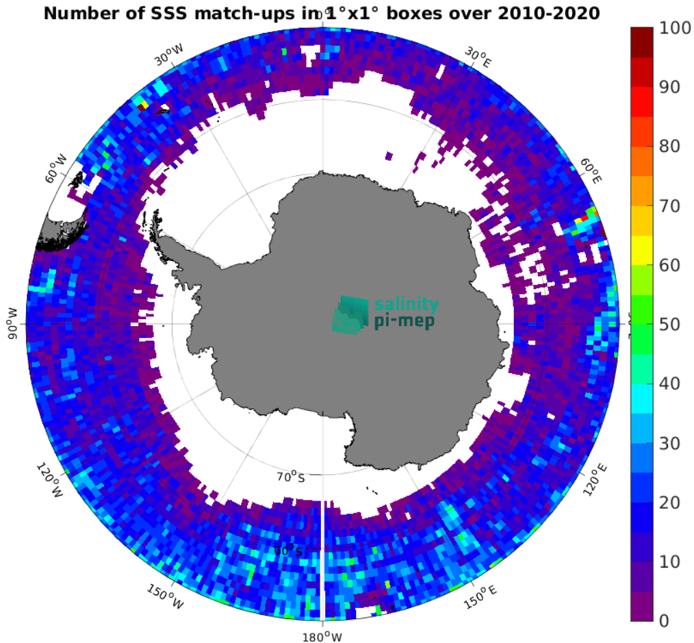
Figure 4: Number of SSS match-ups between Argo SSS and the CCI SSS L4 Merged-OI v3.2 - 30-day running (ESA) SSS product for the Southern Ocean Pi-MEP region over 1^\circ \times 1^\circ boxes and for the full satellite product period.
