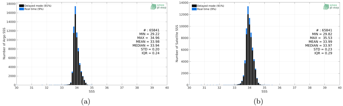
Figure 2: Histograms of SSS from Argo (a) and CCI SSS L4 Merged-OI v3.2 - 30-day running (ESA) (b) considering all match-up pairs per bins of 0.1 over the Southern Ocean Pi-MEP region and for the full satellite product period.
