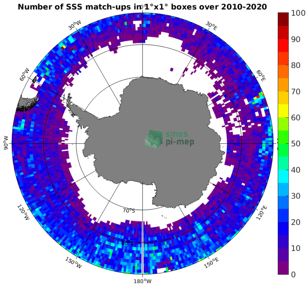
Figure 4: Number of SSS match-ups between Argo SSS and the CCI SSS L4 Merged-OI v3.2 - 30-day running (ESA) SSS product for the Southern Ocean Pi-MEP region over 1^\circ \times 1^\circ boxes and for the full satellite product period.
