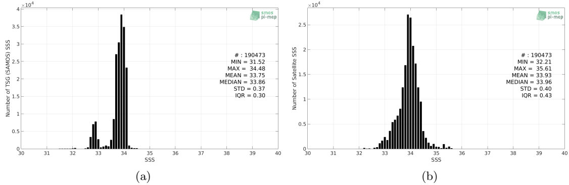
Figure 2: Histograms of SSS from TSG (SAMOS) (a) and CCI SSS L4 Merged-OI v2.31 - 30-day running (ESA) (b) considering all match-up pairs per bins of 0.1 over the Southern Ocean Pi-MEP region and for the full satellite product period.
