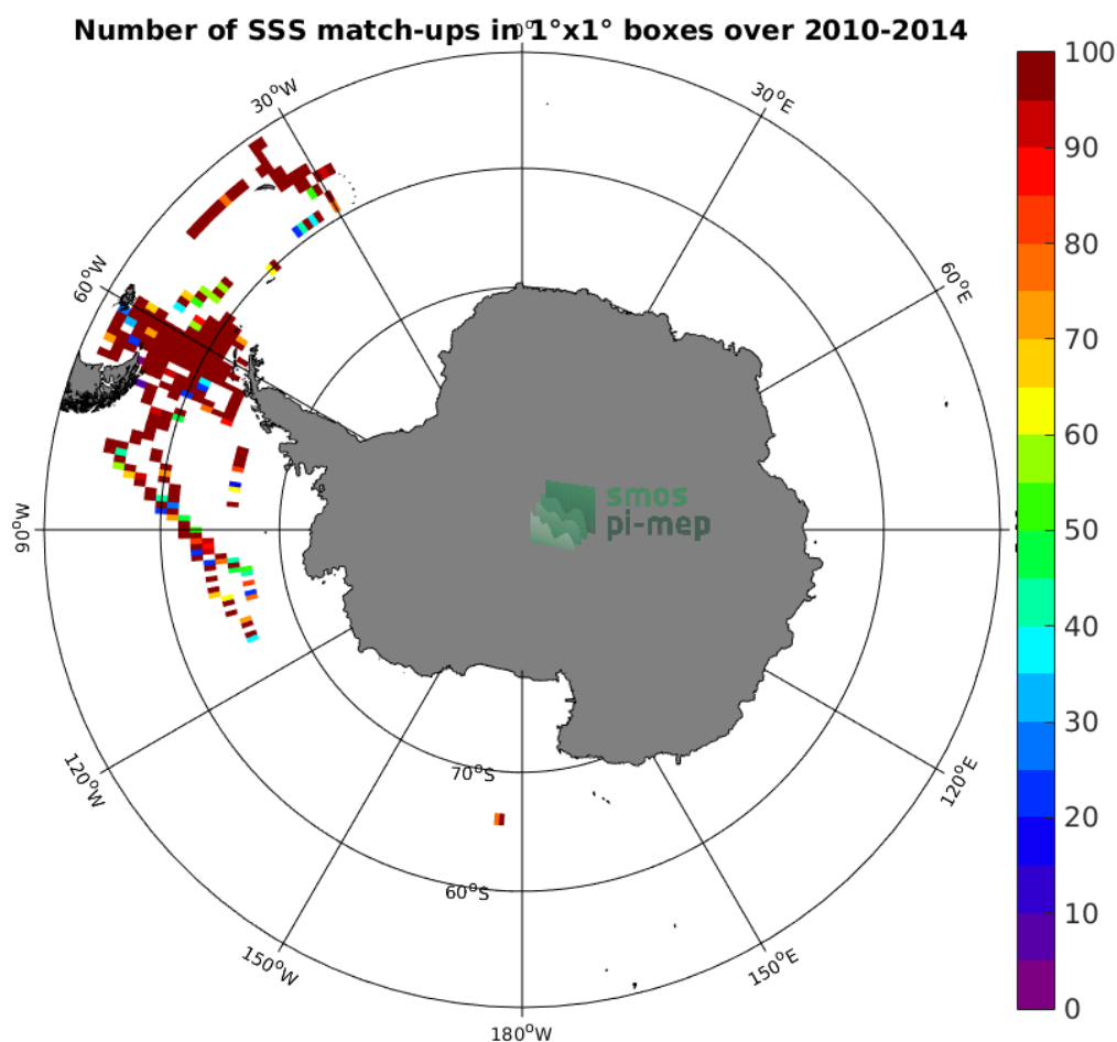
Figure 4: Number of SSS match-ups between TSG (SAMOS) SSS and the CCI SSS L4 Merged-OI v2.31 - 30-day running (ESA) SSS product for the Southern Ocean Pi-MEP region over 1^\circ \times 1^\circ boxes and for the full satellite product period.
