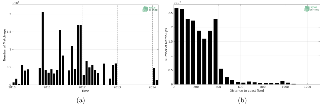
Figure 1: Number of match-ups between TSG (SAMOS) and CCI SSS L4 Merged-OI v2.31 - 30-day running (ESA) SSS as a function of time (a) and as function of the distance to coast (b) over the Southern Ocean Pi-MEP region and for the full satellite product period.
