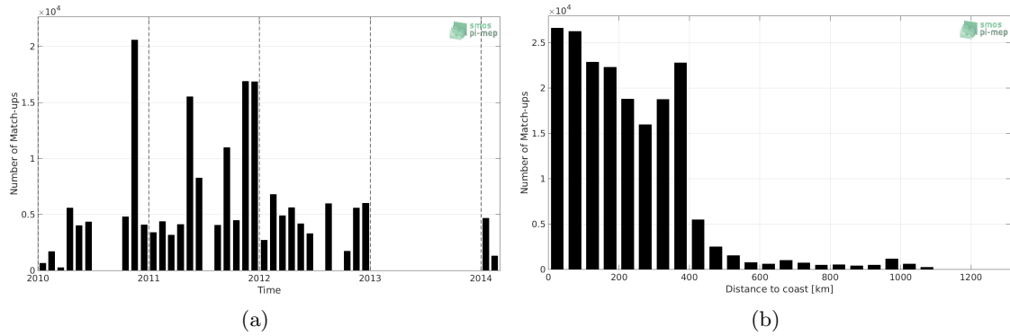
Figure 1: Number of match-ups between TSG (SAMOS) and CCI L4 Merged-OI v2.31 - 30-day running (ESA) SSS as a function of time (a) and as function of the distance to coast (b) over the Southern Ocean Pi-MEP region and for the full satellite product period.
