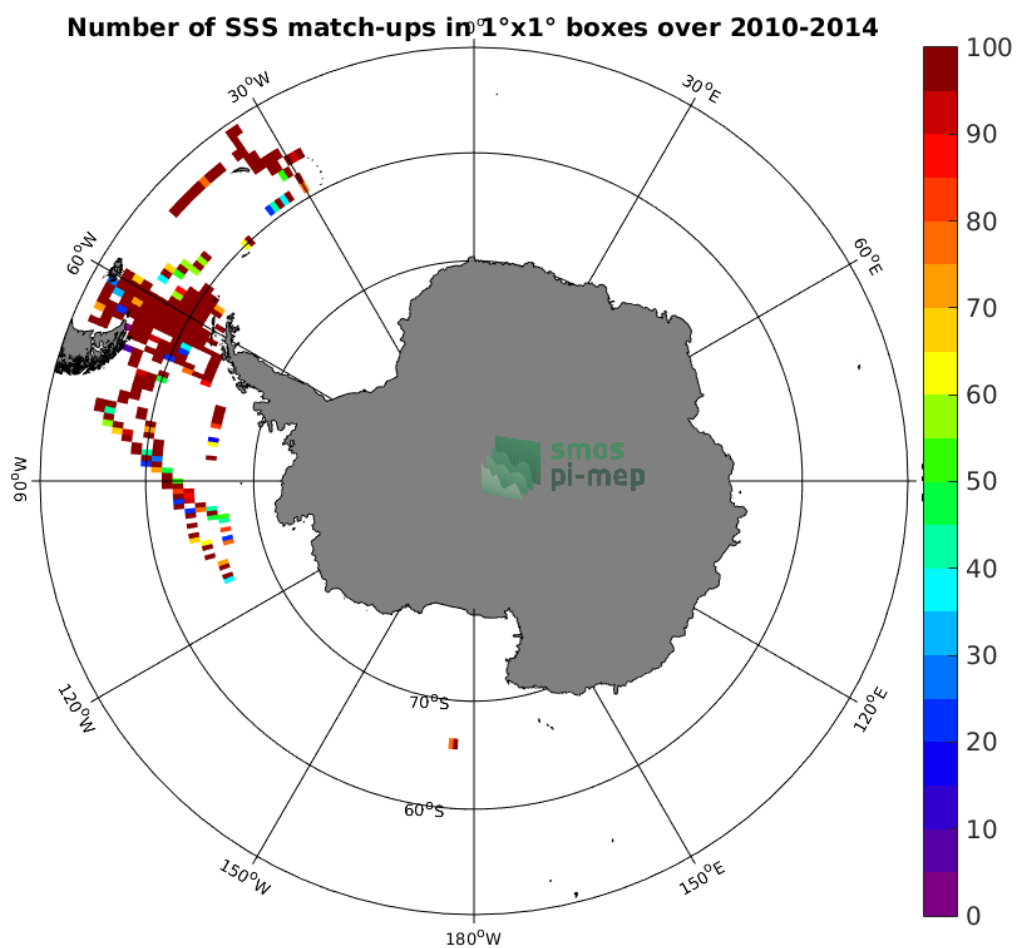
Figure 4: Number of SSS match-ups between TSG (SAMOS) SSS and the CCI L4 Merged-OI v2.31 - 30-day running (ESA) SSS product for the Southern Ocean Pi-MEP region over 1^\circ \times 1^\circ boxes and for the full satellite product period.
