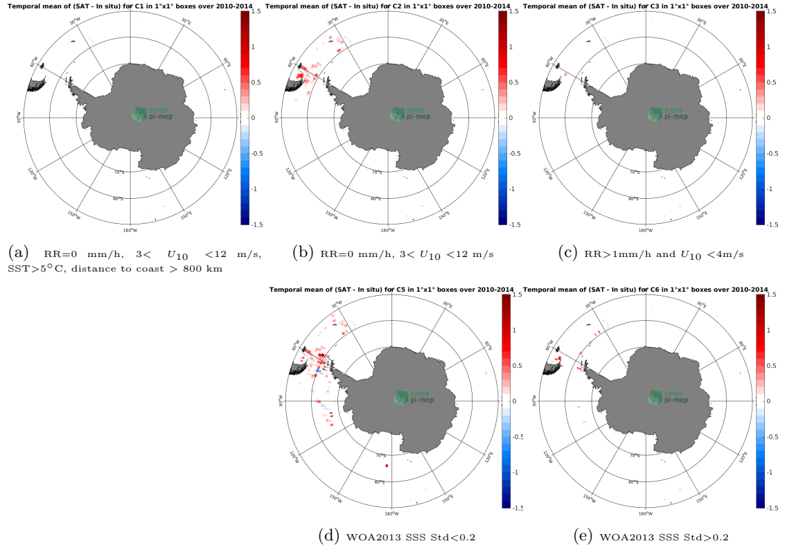
Figure 12: Temporal mean gridded over spatial boxes of size 1^{\circ}\times 1^{\circ} of \Delta\text{SSS} (CCI L4 Merged-OI v2.31 - 30-day running (ESA) - TSG (SAMOS)) for 5 different subdatasets corresponding to: RR=0 mm/h, 3 < U_{10} < 12 m/s, SST >5^{\circ}\text{C} , distance to coast > 800 km (a), RR=0 mm/h, 3 < U_{10} < 12 m/s (b), RR >1 mm/h and U_{10} <4 m/s (c), WOA2013 SSS Std <0.2 (d), WOA2013 SSS Std >0.2 (e).
