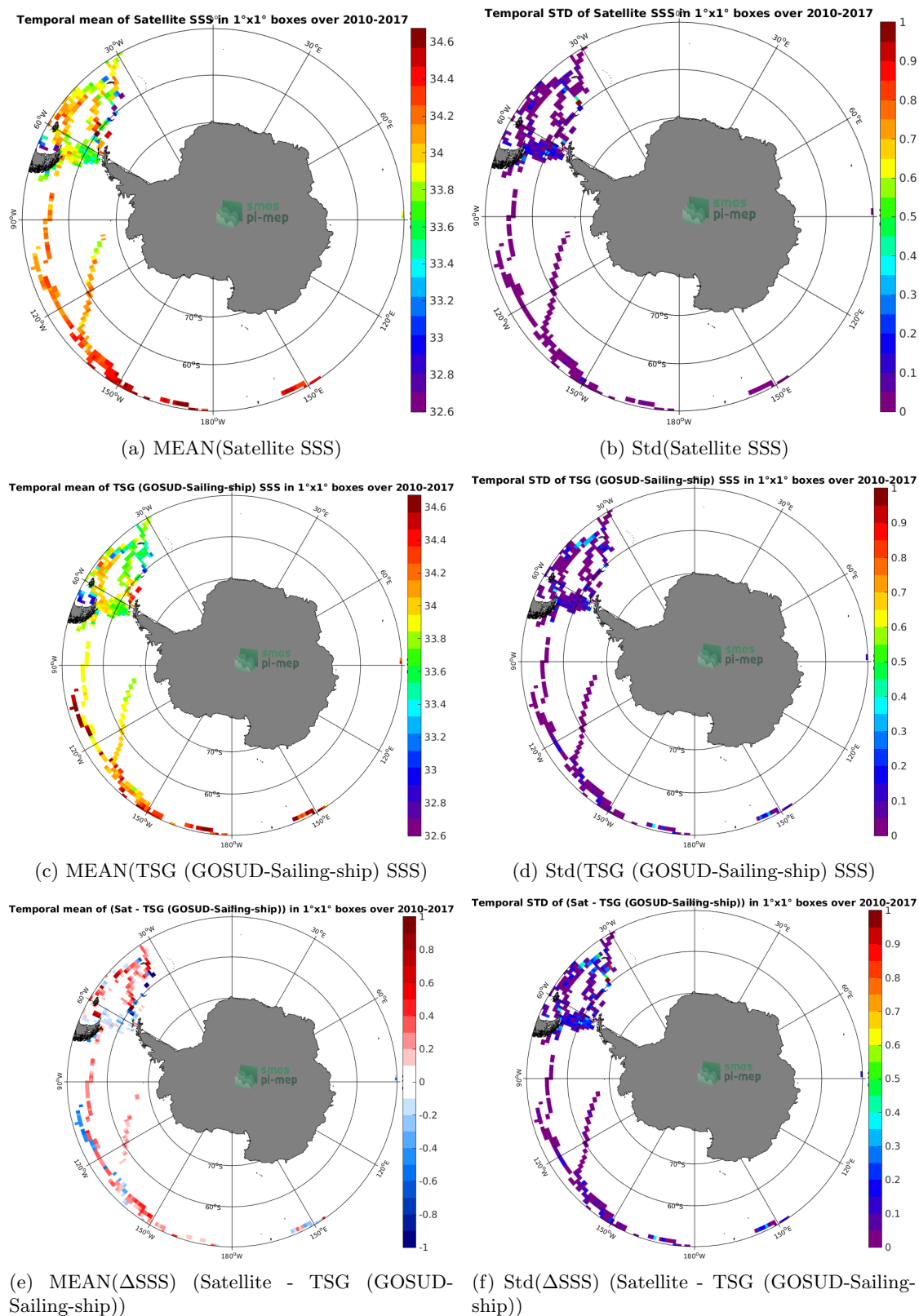
Figure 6: Temporal mean (left) and Std (right) of SSS from CCI SSS L4 Merged-OI v2.31 - 30-day running (ESA) (top), TSG (GOSUD-Sailing-ship) (middle), and of \Delta SSS (Satellite - TSG (GOSUD-Sailing-ship)). Only match-up pairs are used to generate these maps.
