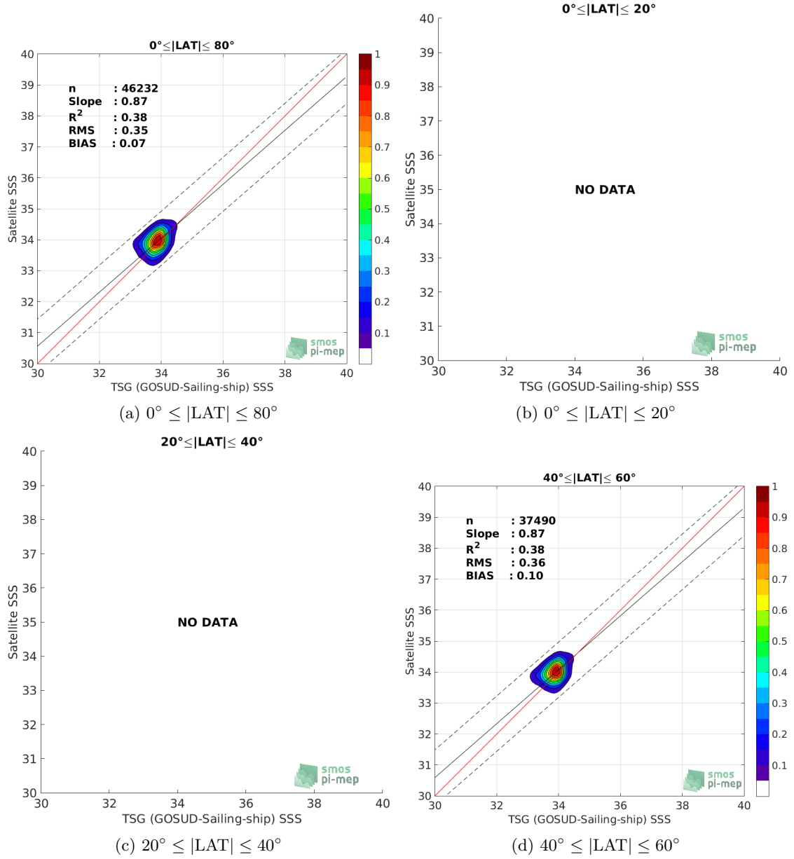
Figure 9: Contour maps of the concentration of CCI SSS L4 Merged-OI v2.31 - 30-day running (ESA) SSS (y-axis) versus TSG (GOSUD-Sailing-ship) SSS (x-axis) at match-up pairs for different latitude bands. For each plot, the red line shows x=y . The black thin and dashed lines indicate a linear fit through the data cloud and the \pm 95\% confidence levels, respectively. The number match-up pairs n , the slope and R^2 coefficient of the linear fit, the root mean square (RMS) and the mean bias between satellite and in situ data are indicated for each latitude band in each plots.
