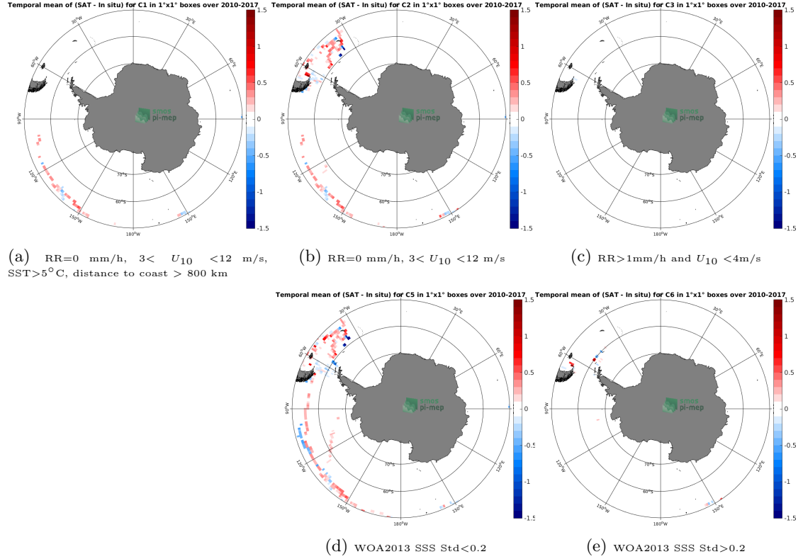
Figure 12: Temporal mean gridded over spatial boxes of size 1^{\circ} \times 1^{\circ} of \Delta\text{SSS} (CCI SSS L4 Merged-OI v2.31 - 30-day running (ESA) - TSG (GOSUD-Sailing-ship)) for 5 different subdatasets corresponding to: RR=0 mm/h, 3 < U_{10} < 12 m/s, SST > 5^{\circ}\text{C} , distance to coast > 800 km (a), RR=0 mm/h, 3 < U_{10} < 12 m/s (b), RR > 1 mm/h and U_{10} < 4 m/s (c), WOA2013 SSS Std < 0.2 (d), WOA2013 SSS Std > 0.2 (e).
