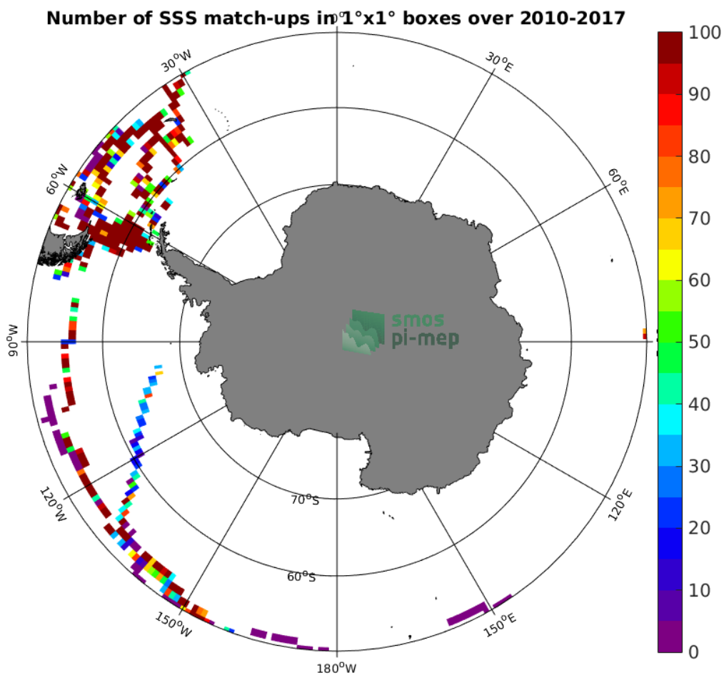
Figure 4: Number of SSS match-ups between TSG (GOSUD-Sailing-ship) SSS and the CCI SSS L4 Merged-OI v2.31 - 30-day running (ESA) SSS product for the Southern Ocean Pi-MEP region over 1^\circ \times 1^\circ boxes and for the full satellite product period.
