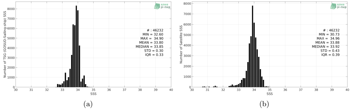
Figure 2: Histograms of SSS from TSG (GOSUD-Sailing-ship) (a) and CCI SSS L4 Merged-OI v2.31 - 30-day running (ESA) (b) considering all match-up pairs per bins of 0.1 over the Southern Ocean Pi-MEP region and for the full satellite product period.
