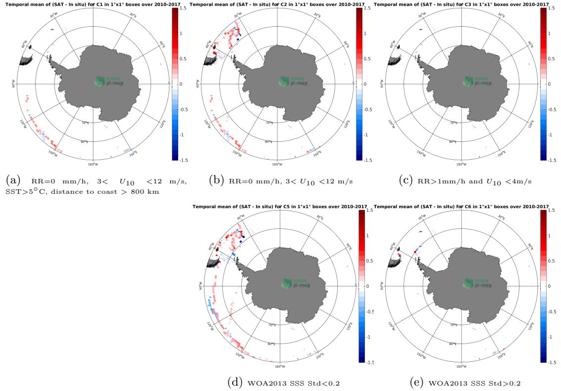
Figure 12: Temporal mean gridded over spatial boxes of size 1°x1° of \Delta\text{SSS} (CCI L4 Merged-OI v2.31 - 30-day running (ESA) - TSG (GOSUD-Sailing-ship)) for 5 different subdatasets corresponding to: RR=0 mm/h, 3 < U_{10} < 12 m/s, SST > 5^\circ\text{C} , distance to coast > 800 km (a), RR=0 mm/h, 3 < U_{10} < 12 m/s (b), RR > 1 mm/h and U_{10} < 4 m/s (c), WOA2013 SSS Std < 0.2 (d), WOA2013 SSS Std > 0.2 (e).
