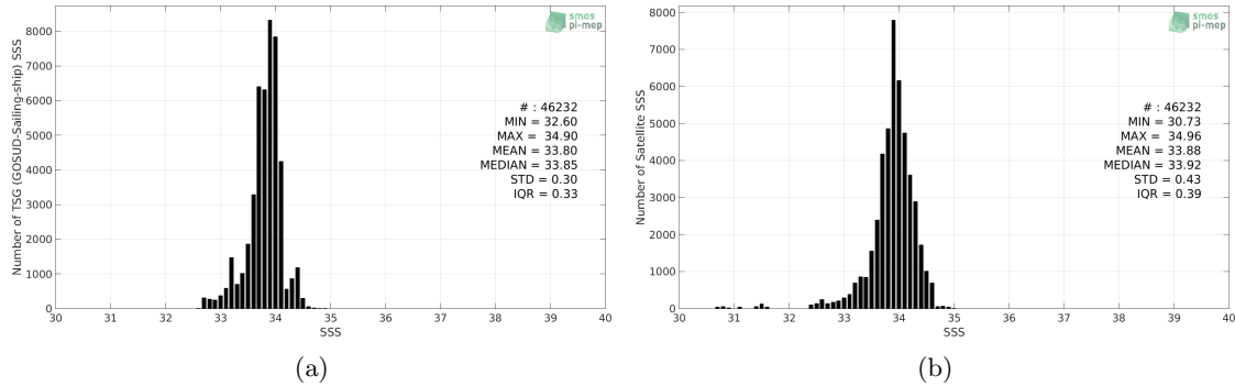
Figure 2: Histograms of SSS from TSG (GOSUD-Sailing-ship) (a) and CCI L4 Merged-OI v2.31 - 30-day running (ESA) (b) considering all match-up pairs per bins of 0.1 over the Southern Ocean Pi-MEP region and for the full satellite product period.
