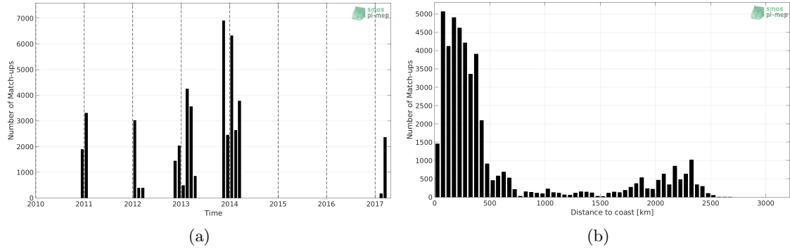
Figure 1: Number of match-ups between TSG (GOSUD-Sailing-ship) and CCI L4 Merged-OI v2.31 - 30-day running (ESA) SSS as a function of time (a) and as function of the distance to coast (b) over the Southern Ocean Pi-MEP region and for the full satellite product period.
