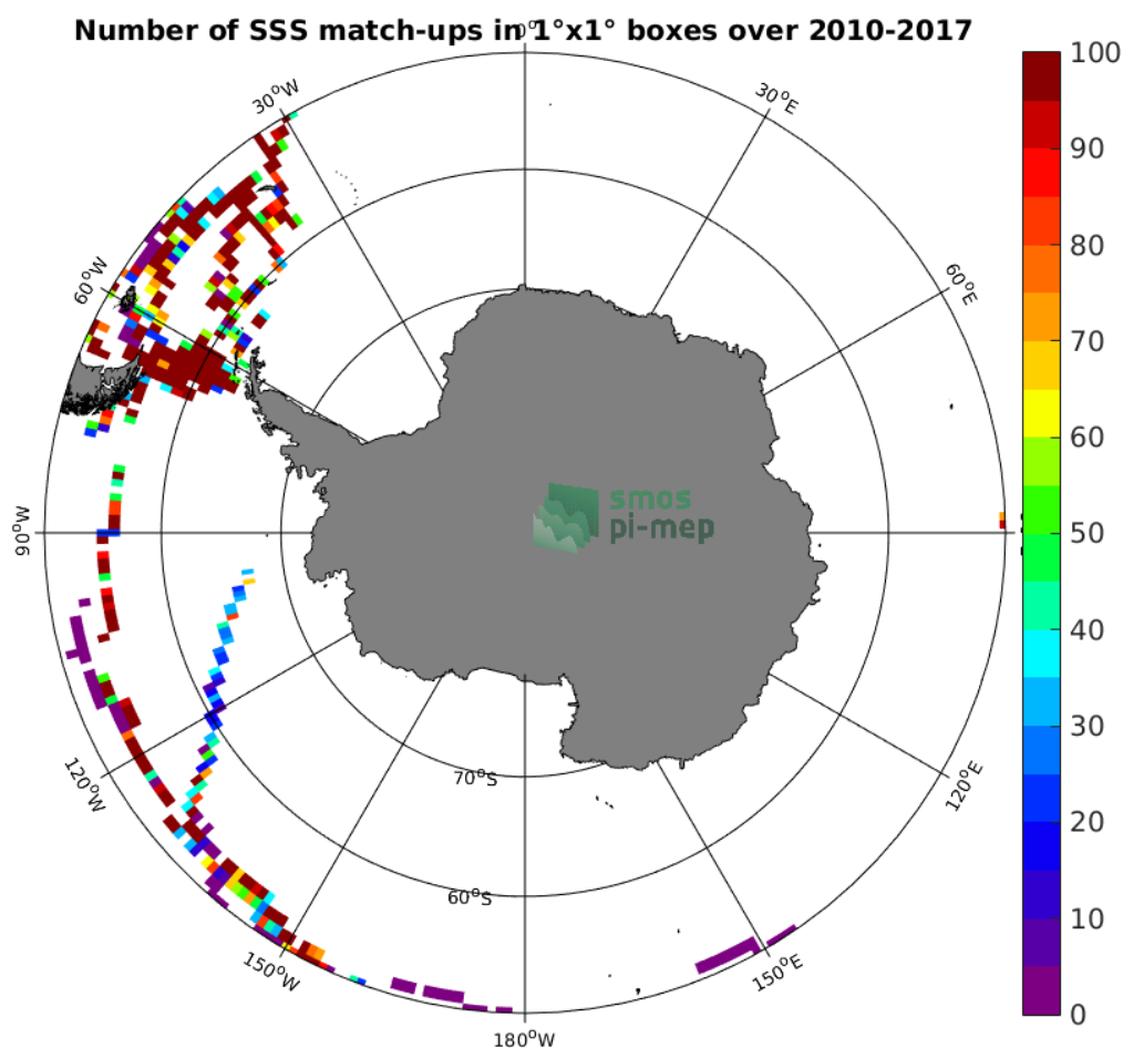
Figure 4: Number of SSS match-ups between TSG (GOSUD-Sailing-ship) SSS and the CCI L4 Merged-OI v2.31 - 30-day running (ESA) SSS product for the Southern Ocean Pi-MEP region over 1^\circ \times 1^\circ boxes and for the full satellite product period.
