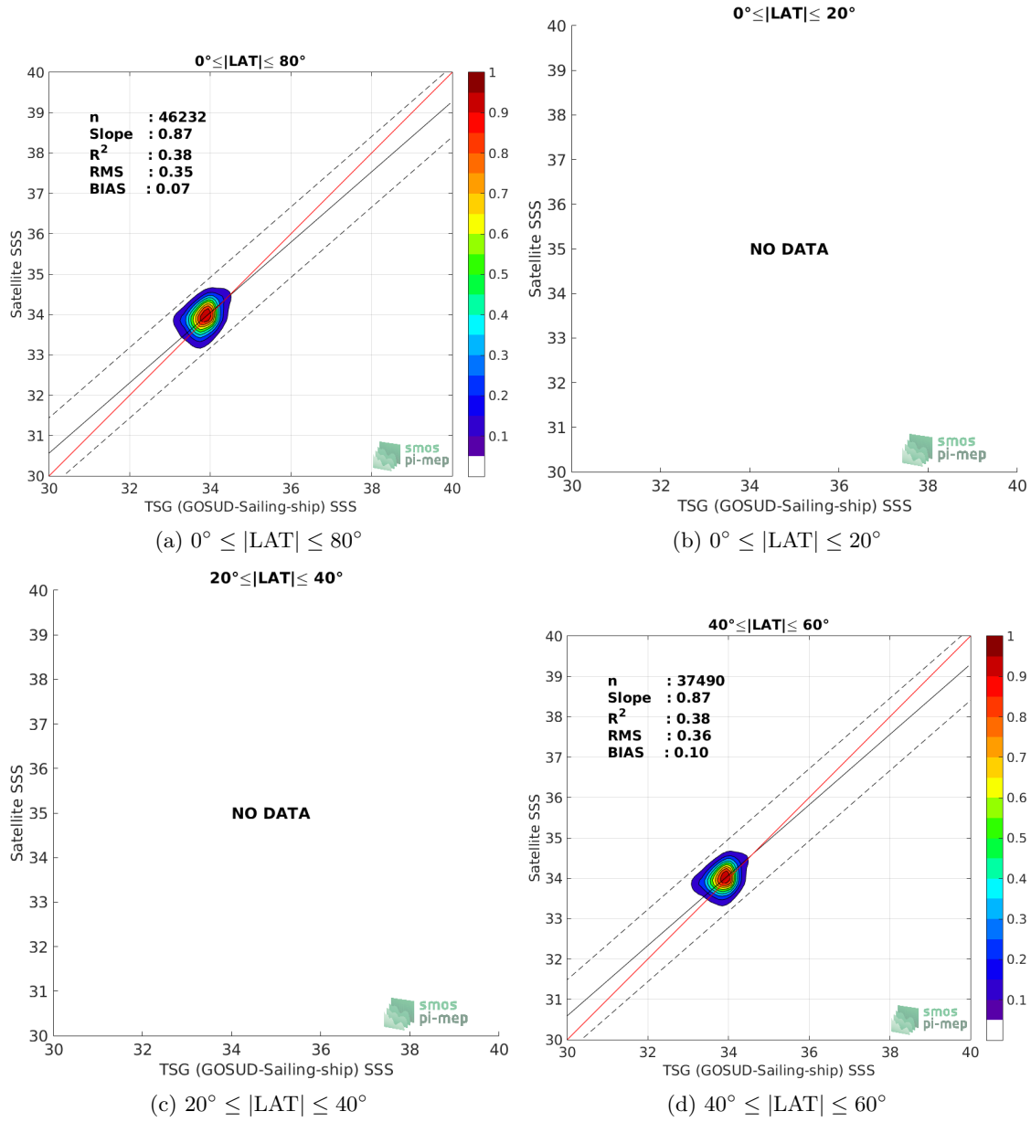
Figure 9: Contour maps of the concentration of CCI L4 Merged-OI v2.31 - 30-day running (ESA) SSS (y-axis) versus TSG (GOSUD-Sailing-ship) SSS (x-axis) at match-up pairs for different latitude bands. For each plot, the red line shows x=y . The black thin and dashed lines indicate a linear fit through the data cloud and the \pm 95\% confidence levels, respectively. The number match-up pairs n , the slope and R^2 coefficient of the linear fit, the root mean square (RMS) and the mean bias between satellite and in situ data are indicated for each latitude band in each plots.
