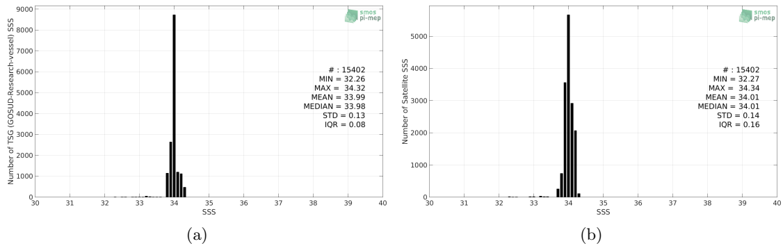
Figure 2: Histograms of SSS from TSG (GOSUD-Research-vessel) (a) and CCI L4 Merged-OI v2.31 - 30-day running (ESA) (b) considering all match-up pairs per bins of 0.1 over the Southern Ocean Pi-MEP region and for the full satellite product period.
