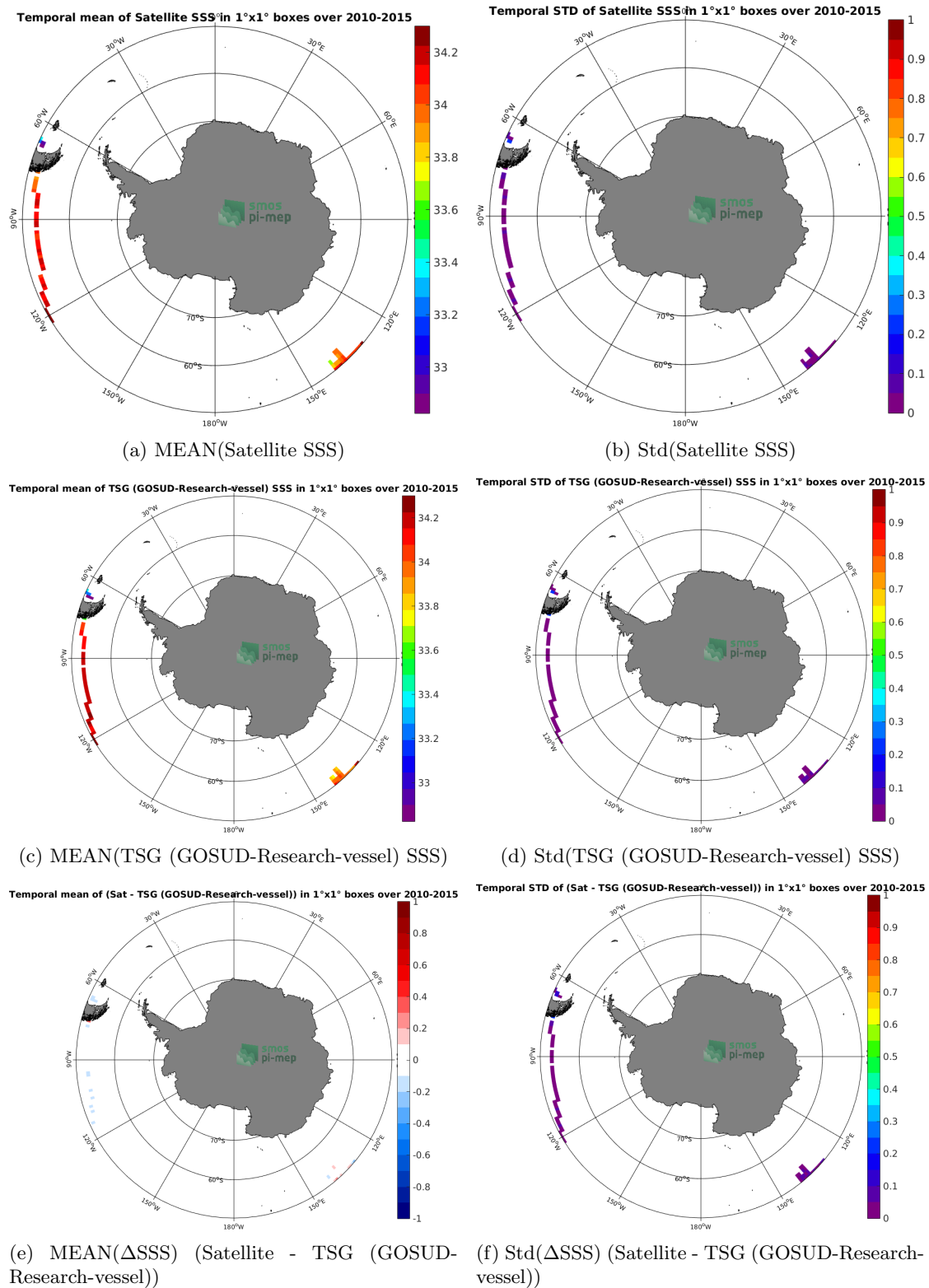
Figure 6: Temporal mean (left) and Std (right) of SSS from CCI L4 Merged-OI v2.31 - 30-day running (ESA) (top), TSG (GOSUD-Research-vessel) (middle), and of \Delta SSS (Satellite - TSG (GOSUD-Research-vessel)). Only match-up pairs are used to generate these maps.
