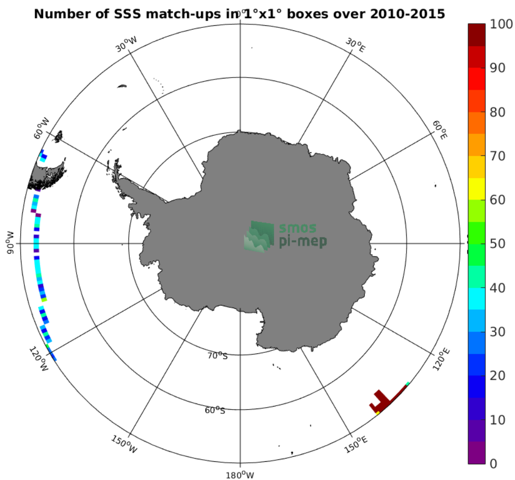
Figure 4: Number of SSS match-ups between TSG (GOSUD-Research-vessel) SSS and the CCI L4 Merged-OI v2.31 - 30-day running (ESA) SSS product for the Southern Ocean Pi-MEP region over 1^\circ \times 1^\circ boxes and for the full satellite product period.
