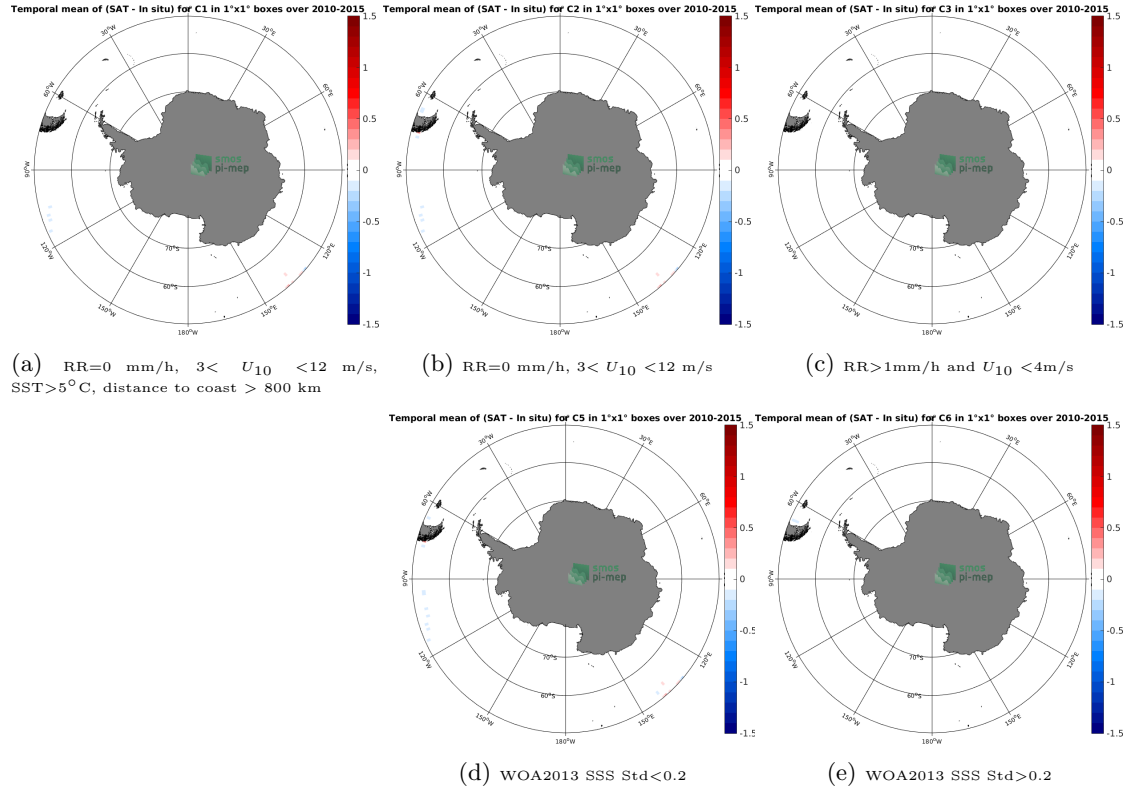
Figure 12: Temporal mean gridded over spatial boxes of size 1°x1° of \Delta SSS (CCI L4 Merged-OI v2.31 - 30-day running (ESA) - TSG (GOSUD-Research-vessel)) for 5 different subdatasets corresponding to:RR=0 mm/h, 3 < U_{10} < 12 m/s, SST>5°C, distance to coast > 800 km (a), RR=0 mm/h, 3 < U_{10} < 12 m/s (b), RR>1mm/h and U_{10} < 4 m/s (c), WOA2013 SSS Std<0.2 (d), WOA2013 SSS Std>0.2 (e).
