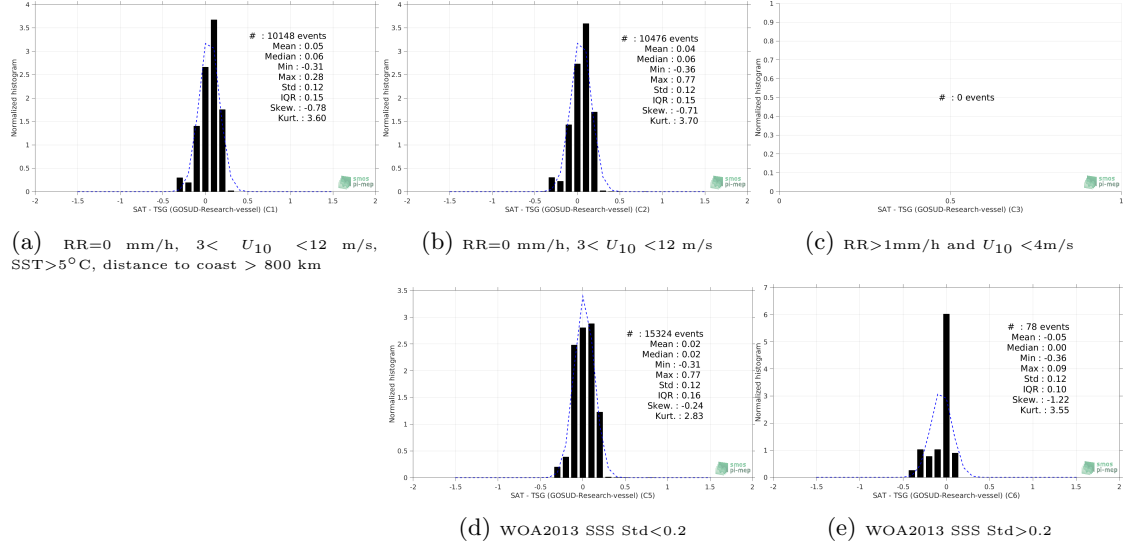
Figure 13: Normalized histogram of \Delta SSS (CCI L4 Merged-OI v2.31 - 30-day running (ESA) - TSG (GOSUD-Research-vessel)) for 5 different subdatasets corresponding to: RR=0 mm/h, 3 < U_{10} < 12 m/s, SST>5°C, distance to coast > 800 km (a), RR=0 mm/h, 3 < U_{10} < 12 m/s (b), RR>1mm/h and U_{10} < 4 m/s (c), WOA2013 SSS Std<0.2 (d), WOA2013 SSS Std>0.2 (e).
