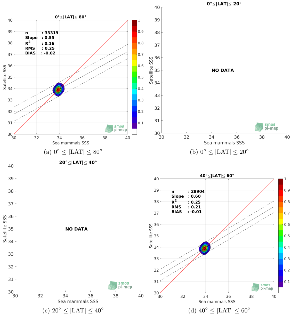
Figure 9: Contour maps of the concentration of CCI L4 Merged-OI v2.31 - 30-day running (ESA) SSS (y-axis) versus Sea mammals SSS (x-axis) at match-up pairs for different latitude bands. For each plot, the red line shows x=y . The black thin and dashed lines indicate a linear fit through the data cloud and the \pm 95\% confidence levels, respectively. The number match-up pairs n , the slope and R^2 coefficient of the linear fit, the root mean square (RMS) and the mean bias between satellite and in situ data are indicated for each latitude band in each plots.
