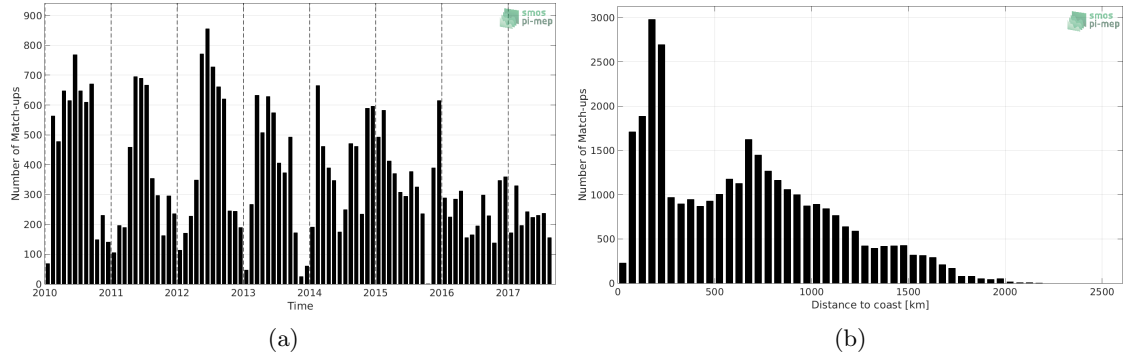
Figure 1: Number of match-ups between Sea mammals and CCI L4 Merged-OI v2.31 - 30-day running (ESA) SSS as a function of time (a) and as function of the distance to coast (b) over the Southern Ocean Pi-MEP region and for the full satellite product period.
