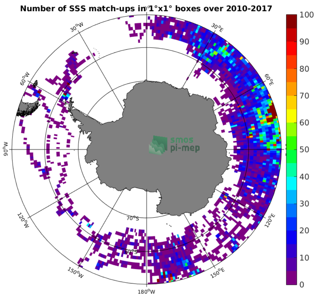
Figure 4: Number of SSS match-ups between Sea mammals SSS and the CCI L4 Merged-OI v2.31 - 30-day running (ESA) SSS product for the Southern Ocean Pi-MEP region over 1^\circ \times 1^\circ boxes and for the full satellite product period.
