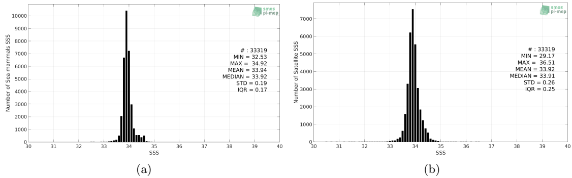
Figure 2: Histograms of SSS from Sea mammals (a) and CCI L4 Merged-OI v2.31 - 30-day running (ESA) (b) considering all match-up pairs per bins of 0.1 over the Southern Ocean Pi-MEP region and for the full satellite product period.
