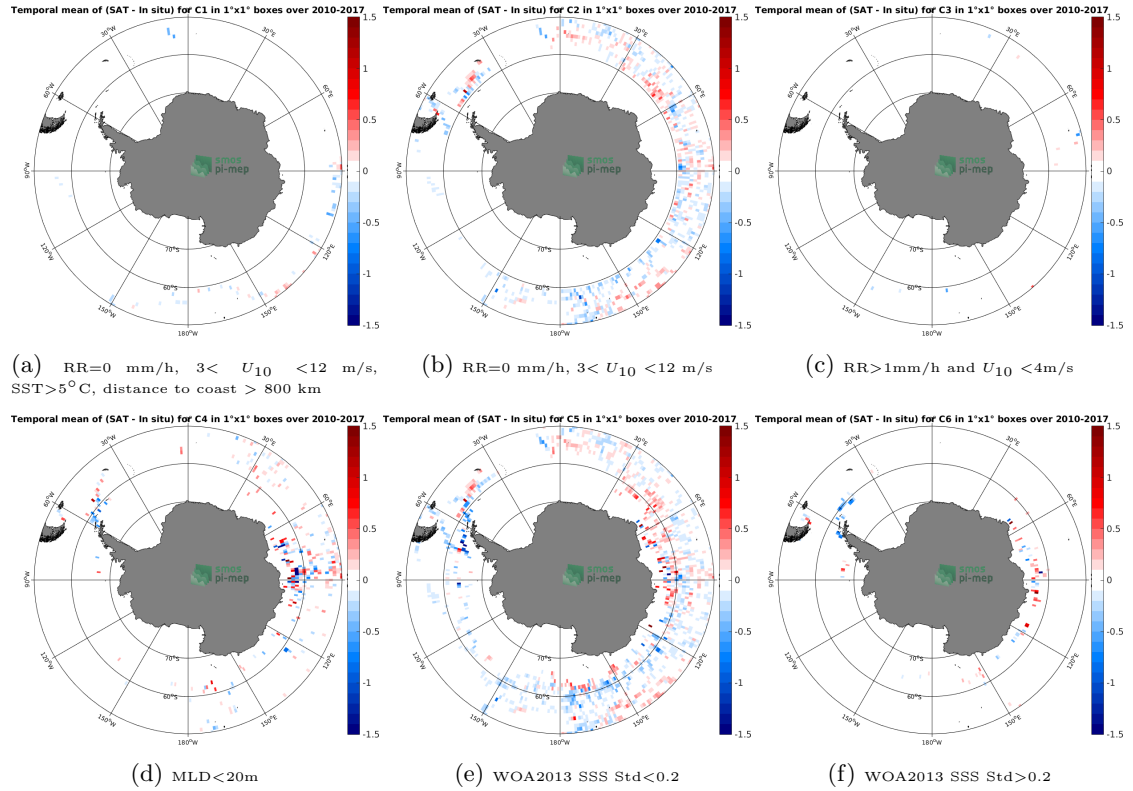
Figure 12: Temporal mean gridded over spatial boxes of size 1^{\circ}\times 1^{\circ} of \Delta\text{SSS} (CCI L4 Merged-OI v2.31 - 30-day running (ESA) - Sea mammals) for 6 different subdatasets corresponding to:RR=0 mm/h, 3 < U_{10} < 12 m/s, SST >5^{\circ}\text{C} , distance to coast > 800 km (a), RR=0 mm/h, 3 < U_{10} < 12 m/s (b), RR >1 mm/h and U_{10} < 4 m/s (c),MLD <20 m (d),WOA2013 SSS Std <0.2 (e),WOA2013 SSS Std >0.2 (f).
