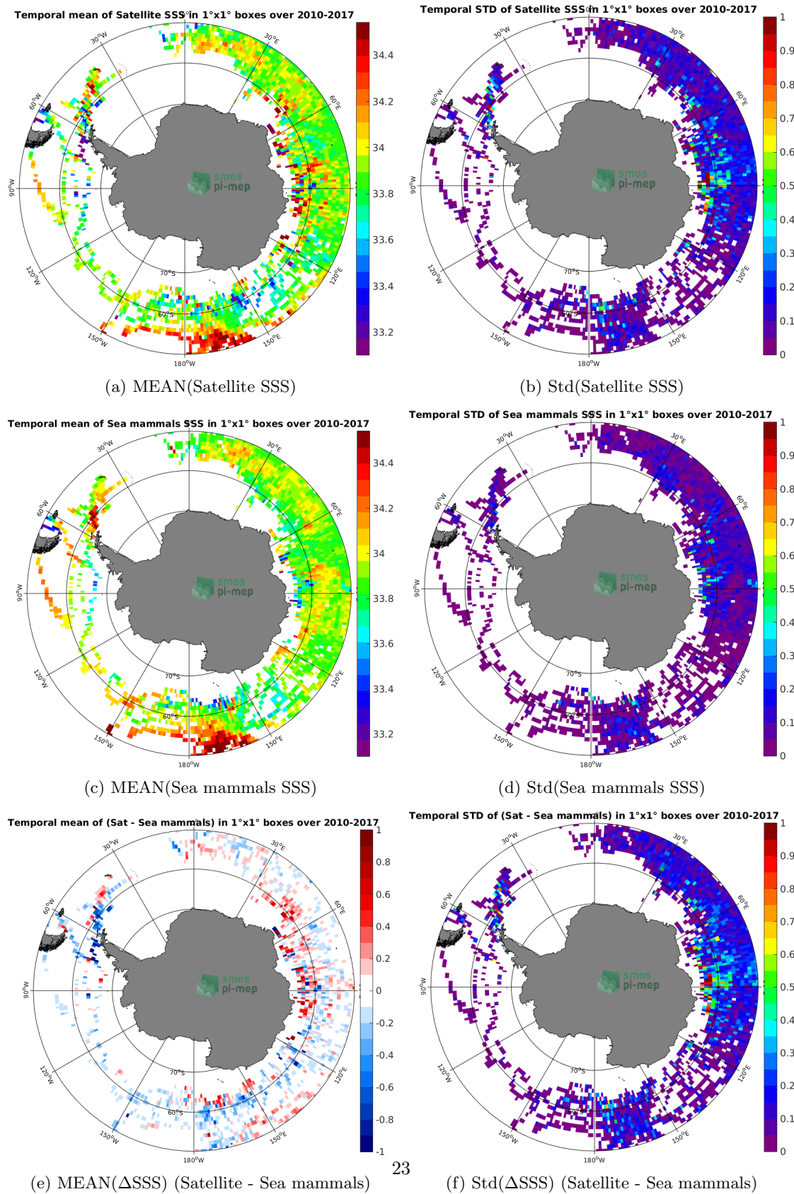
Figure 6: Temporal mean (left) and Std (right) of SSS from CCI L4 Merged-OI v2.31 - 30-day running (ESA) (top), Sea mammals (middle), and of \Delta SSS (Satellite - Sea mammals). Only match-up pairs are used to generate these maps.
