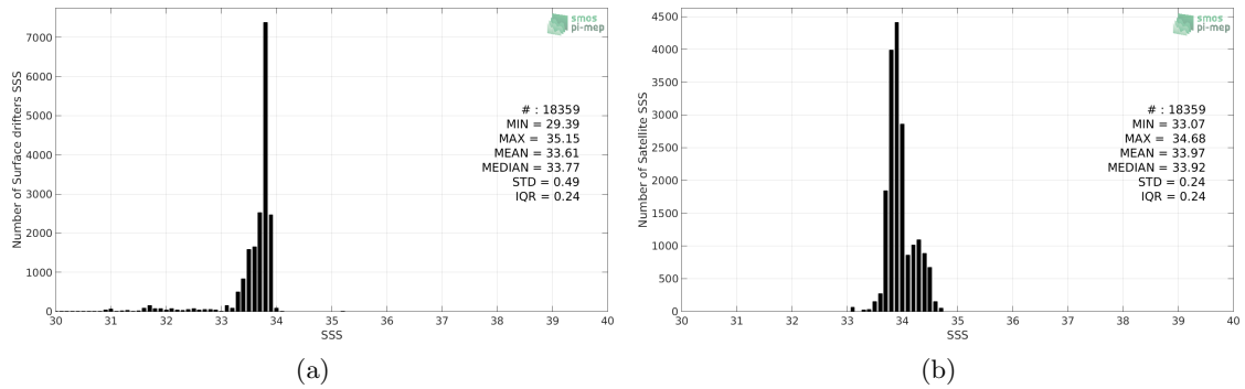
Figure 2: Histograms of SSS from Surface drifters (a) and CCI SSS L4 Merged-OI v2.31 - 30-day running (ESA) (b) considering all match-up pairs per bins of 0.1 over the Southern Ocean Pi-MEP region and for the full satellite product period.
