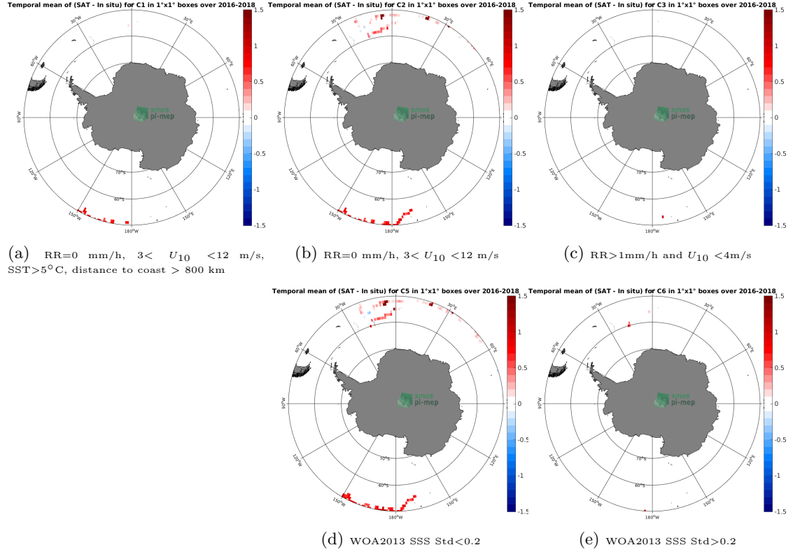
Figure 11: Temporal mean gridded over spatial boxes of size 1^{\circ}\times 1^{\circ} of \Delta\text{SSS} (CCI SSS L4 Merged-OI v2.31 - 30-day running (ESA) - Surface drifters) for 5 different subdatasets corresponding to: \text{RR}=0 mm/h, 3 < U_{10} < 12 m/s, \text{SST}>5^{\circ}\text{C} , distance to coast > 800 km (a), \text{RR}=0 mm/h, 3 < U_{10} < 12 m/s (b), \text{RR}>1\text{mm/h} and U_{10} <4\text{m/s} (c), WOA2013 SSS Std <0.2 (d), WOA2013 SSS Std >0.2 (e).
