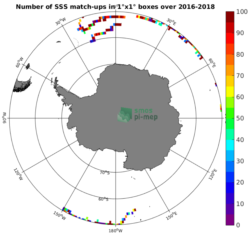
Figure 3: Number of SSS match-ups between Surface drifters SSS and the CCI SSS L4 Merged-OI v2.31 - 30-day running (ESA) SSS product for the Southern Ocean Pi-MEP region over 1^\circ \times 1^\circ boxes and for the full satellite product period.
