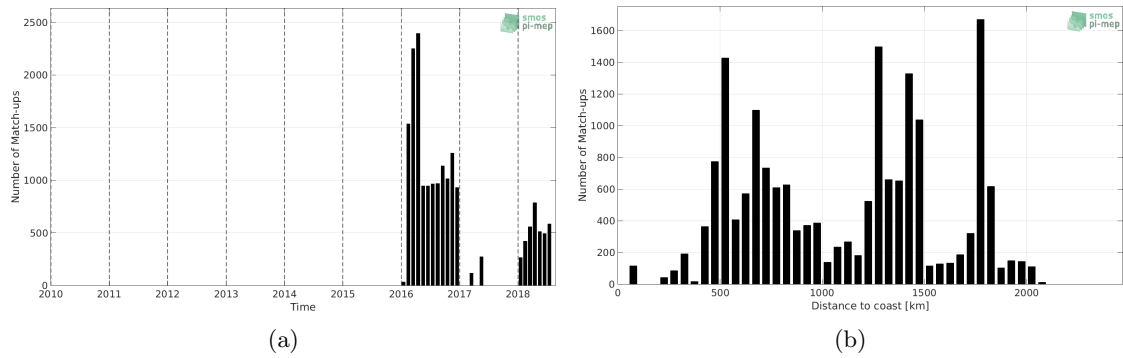
Figure 1: Number of match-ups between Surface drifters and CCI SSS L4 Merged-OI v2.31 - 30-day running (ESA) SSS as a function of time (a) and as function of the distance to coast (b) over the Southern Ocean Pi-MEP region and for the full satellite product period.
