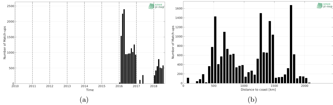
Figure 1: Number of match-ups between Surface drifters and CCI L4 Merged-OI v2.31 - 30-day running (ESA) SSS as a function of time (a) and as function of the distance to coast (b) over the Southern Ocean Pi-MEP region and for the full satellite product period.
