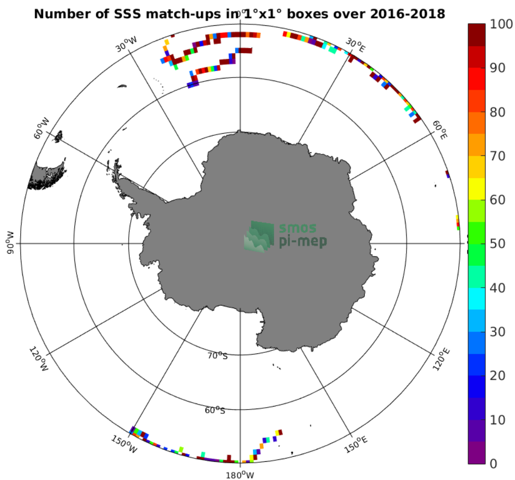
Figure 3: Number of SSS match-ups between Surface drifters SSS and the CCI L4 Merged-OI v2.31 - 30-day running (ESA) SSS product for the Southern Ocean Pi-MEP region over 1^\circ \times 1^\circ boxes and for the full satellite product period.
