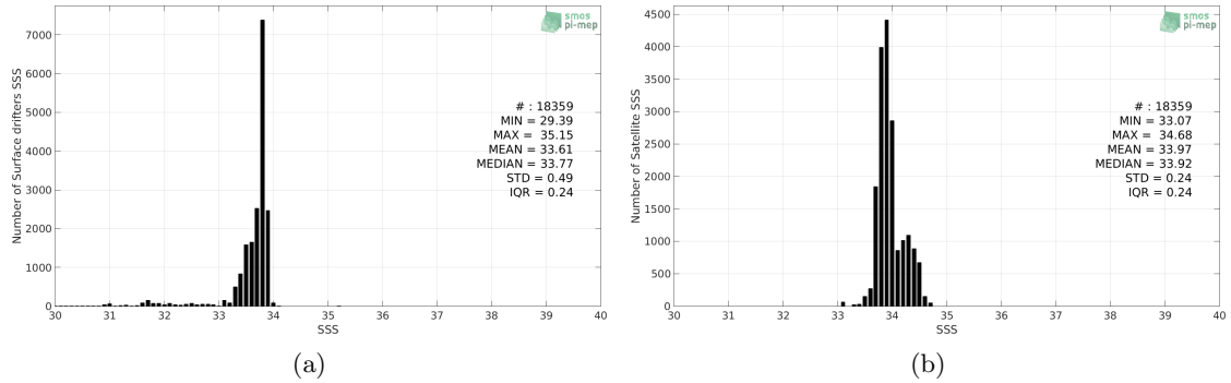
Figure 2: Histograms of SSS from Surface drifters (a) and CCI L4 Merged-OI v2.31 - 30-day running (ESA) (b) considering all match-up pairs per bins of 0.1 over the Southern Ocean Pi-MEP region and for the full satellite product period.
