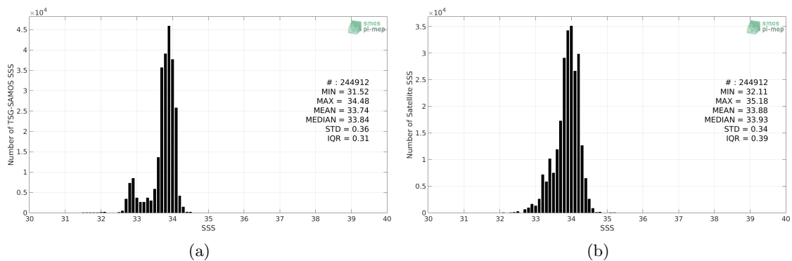
Figure 2: Histograms of SSS from TSG-SAMOS (a) and CCI L4 Merged-OI v1.8 - 30-day running (ESA) (b) considering all match-up pairs per bins of 0.1 over the Southern Ocean Pi-MEP region and for the full satellite product period.
