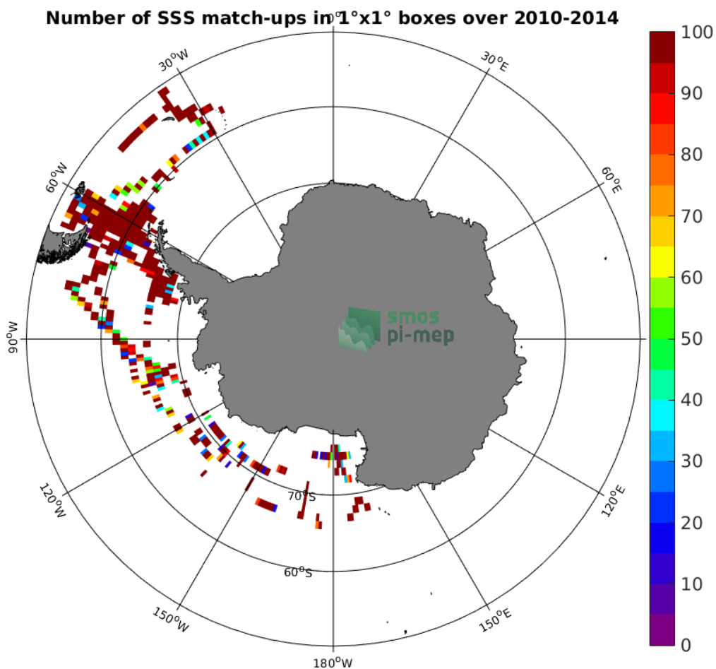
Figure 4: Number of SSS match-ups between TSG-SAMOS SSS and the CCI L4 Merged-OI v1.8 - 30-day running (ESA) SSS product for the Southern Ocean Pi-MEP region over 1^\circ \times 1^\circ boxes and for the full satellite product period.
