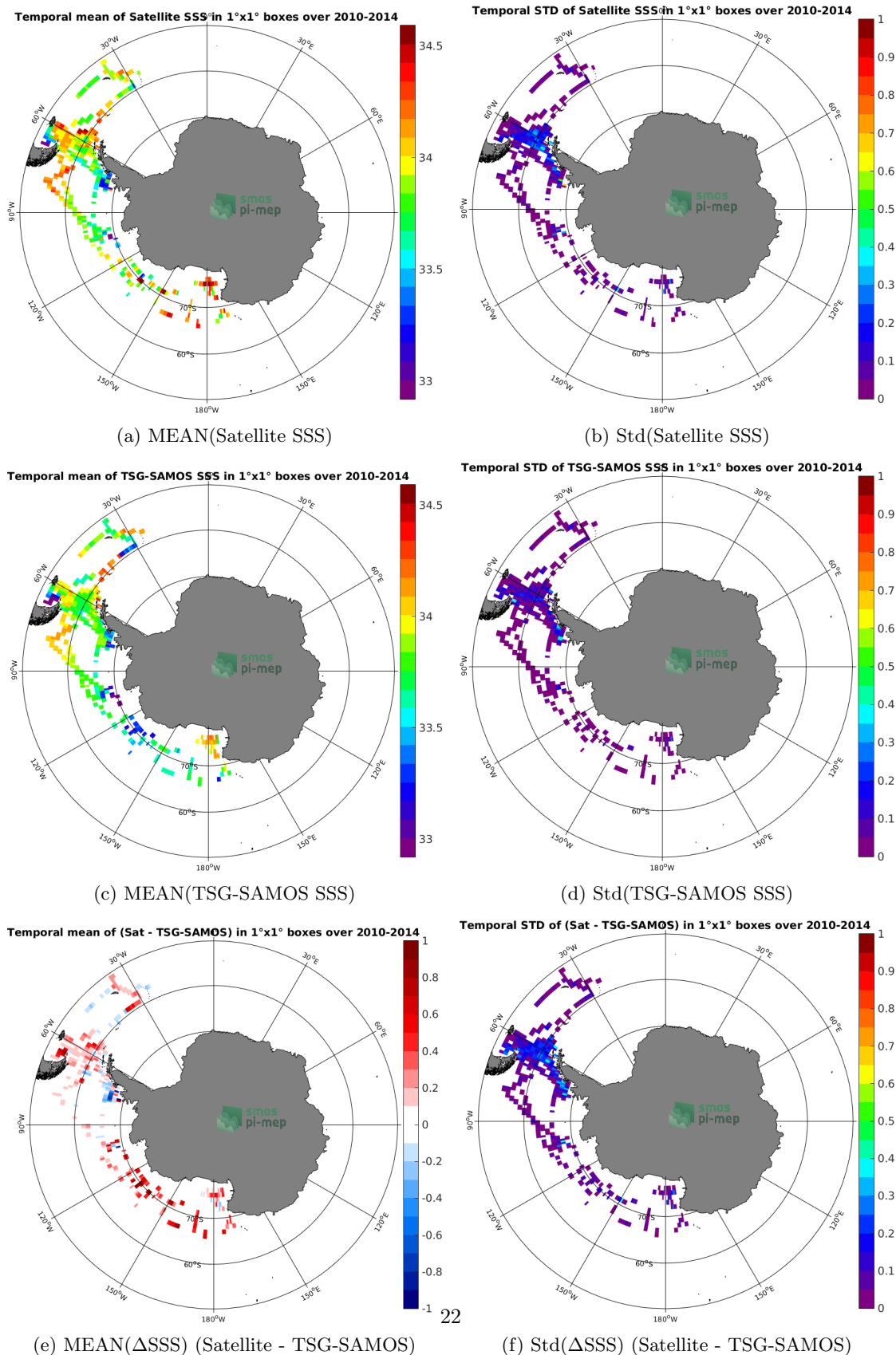
Figure 6: Temporal mean (left) and Std (right) of SSS from CCI L4 Merged-OI v1.8 - 30-day running (ESA) (top), TSG-SAMOS (middle), and of \Delta SSS (Satellite - TSG-SAMOS). Only match-up pairs are used to generate these maps.
