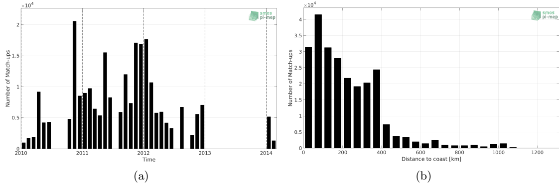
Figure 1: Number of match-ups between TSG-SAMOS and CCI L4 Merged-OI v1.8 - 30-day running (ESA) SSS as a function of time (a) and as function of the distance to coast (b) over the Southern Ocean Pi-MEP region and for the full satellite product period.
