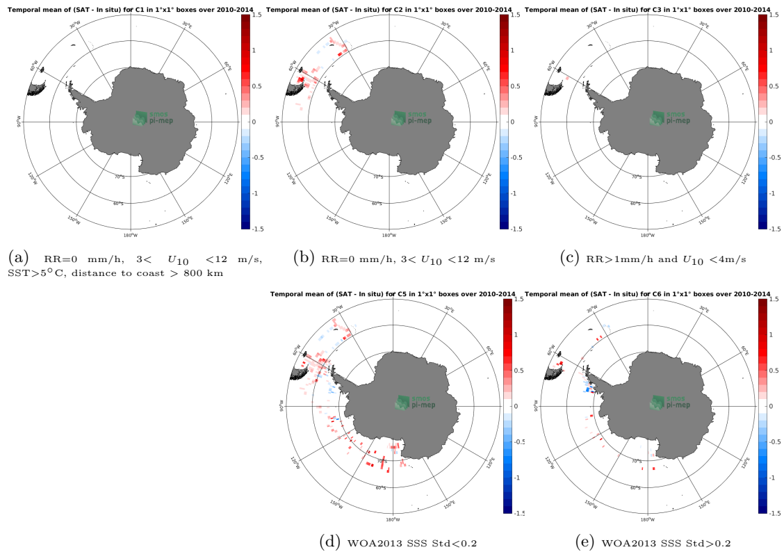
Figure 12: Temporal mean gridded over spatial boxes of size 1^{\circ}\times 1^{\circ} of \Delta\text{SSS} (CCI L4 Merged-OI v1.8 - 30-day running (ESA) - TSG-SAMOS) for 5 different subdatasets corresponding to:RR=0 mm/h, 3 < U_{10} < 12 m/s, SST >5^{\circ}\text{C} , distance to coast > 800 km (a), RR=0 mm/h, 3 < U_{10} < 12 m/s (b), RR >1 mm/h and U_{10} < 4 m/s (c), WOA2013 SSS Std <0.2 (d), WOA2013 SSS Std >0.2 (e).
