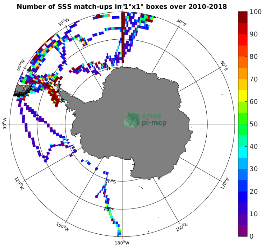
Figure 4: Number of SSS match-ups between TSG-POLARSTERN SSS and the CCI L4 Merged-OI v1.8 - 30-day running (ESA) SSS product for the Southern Ocean Pi-MEP region over 1^\circ \times 1^\circ boxes and for the full satellite product period.
