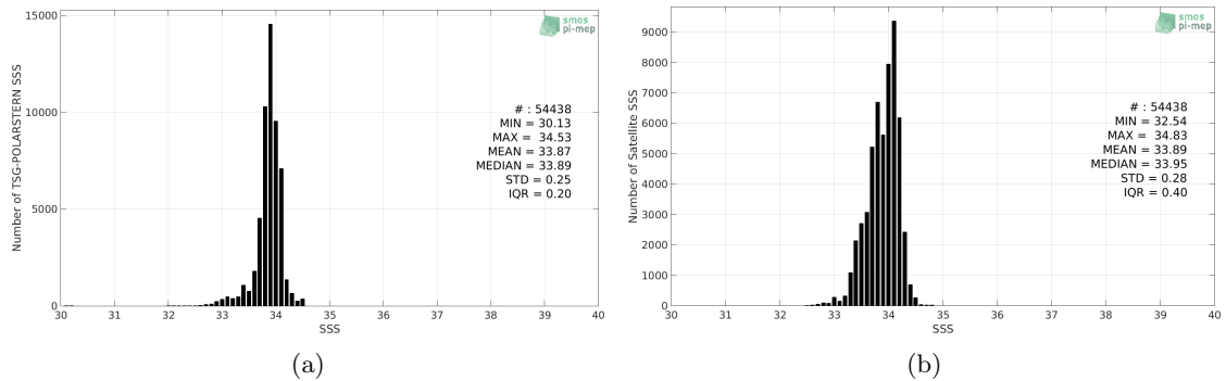
Figure 2: Histograms of SSS from TSG-POLARSTERN (a) and CCI L4 Merged-OI v1.8 - 30-day running (ESA) (b) considering all match-up pairs per bins of 0.1 over the Southern Ocean Pi-MEP region and for the full satellite product period.
