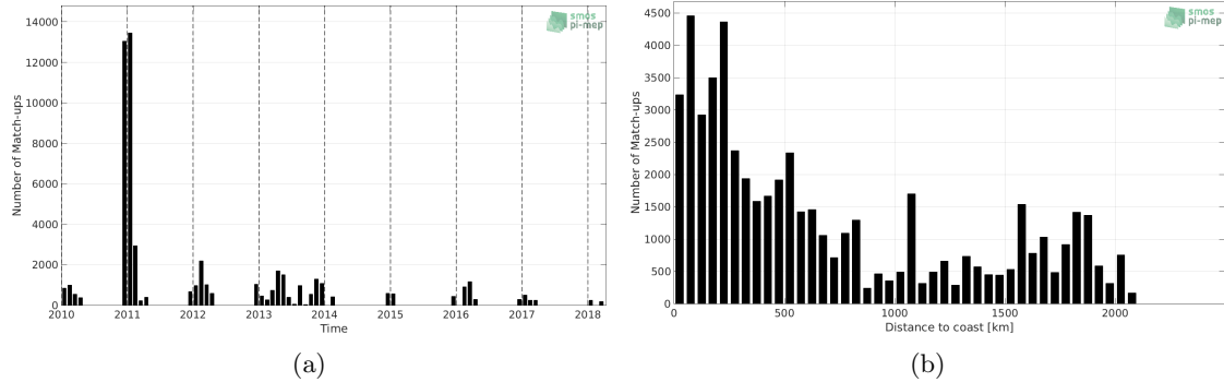
Figure 1: Number of match-ups between TSG-POLARSTERN and CCI L4 Merged-OI v1.8 - 30-day running (ESA) SSS as a function of time (a) and as function of the distance to coast (b) over the Southern Ocean Pi-MEP region and for the full satellite product period.
