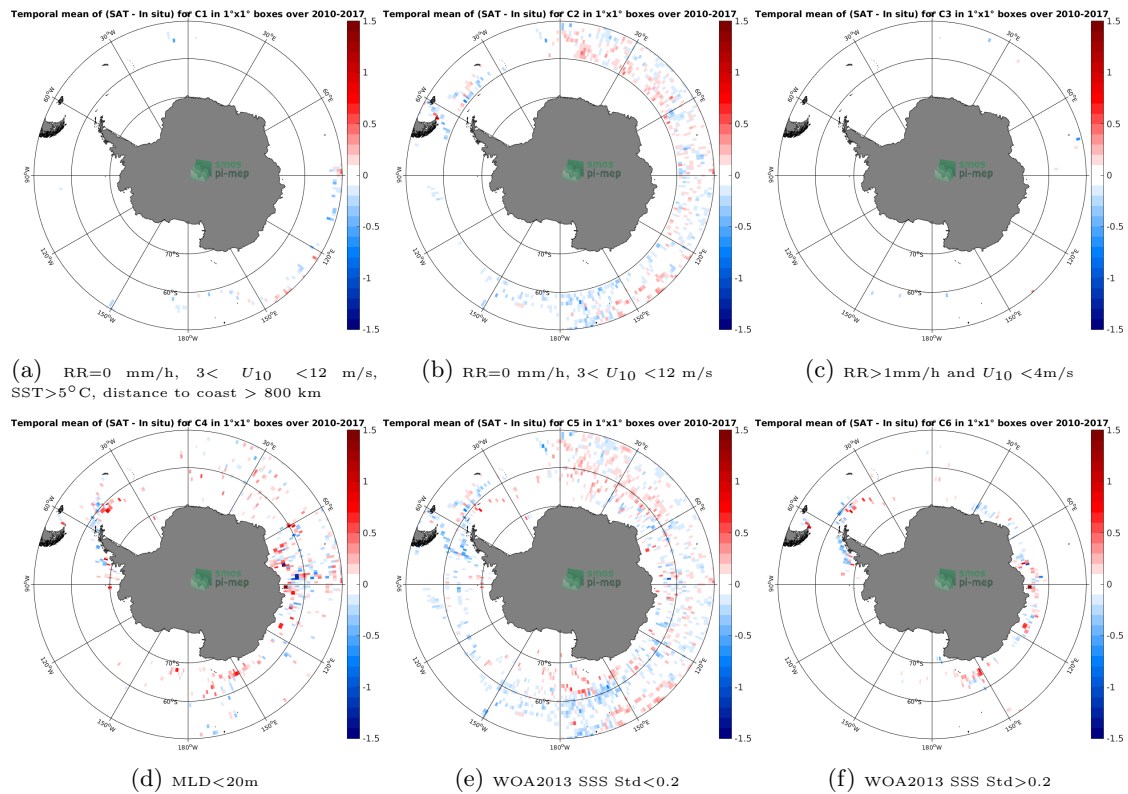
Figure 12: Temporal mean gridded over spatial boxes of size 1^{\circ}\times 1^{\circ} of \Delta\text{SSS} (CCI L4 Merged-OI v1.8 - 30-day running (ESA) - Sea mammals) for 6 different subdatasets corresponding to: RR=0 mm/h, 3 < U_{10} < 12 m/s, SST > 5^{\circ}\text{C} , distance to coast > 800 km (a), RR=0 mm/h, 3 < U_{10} < 12 m/s (b), RR > 1\text{mm/h} and U_{10} < 4\text{m/s} (c), MLD < 20\text{m} (d), WOA2013 SSS Std < 0.2 (e), WOA2013 SSS Std > 0.2 (f).
