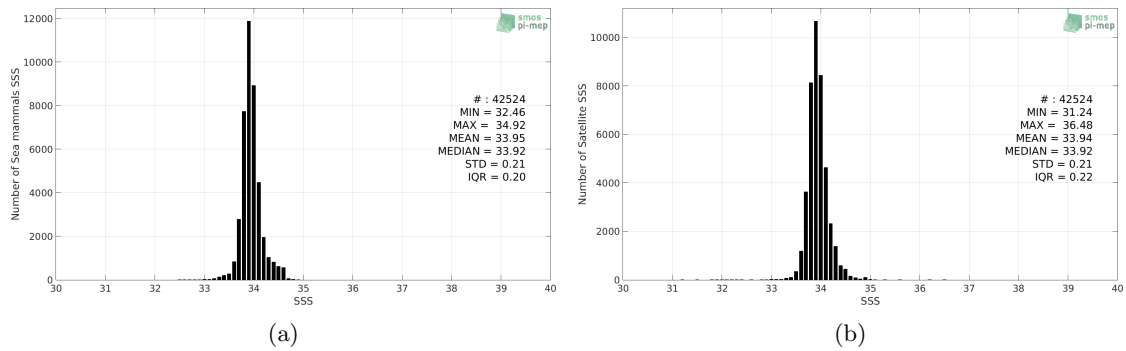
Figure 2: Histograms of SSS from Sea mammals (a) and CCI L4 Merged-OI v1.8 - 30-day running (ESA) (b) considering all match-up pairs per bins of 0.1 over the Southern Ocean Pi-MEP region and for the full satellite product period.
