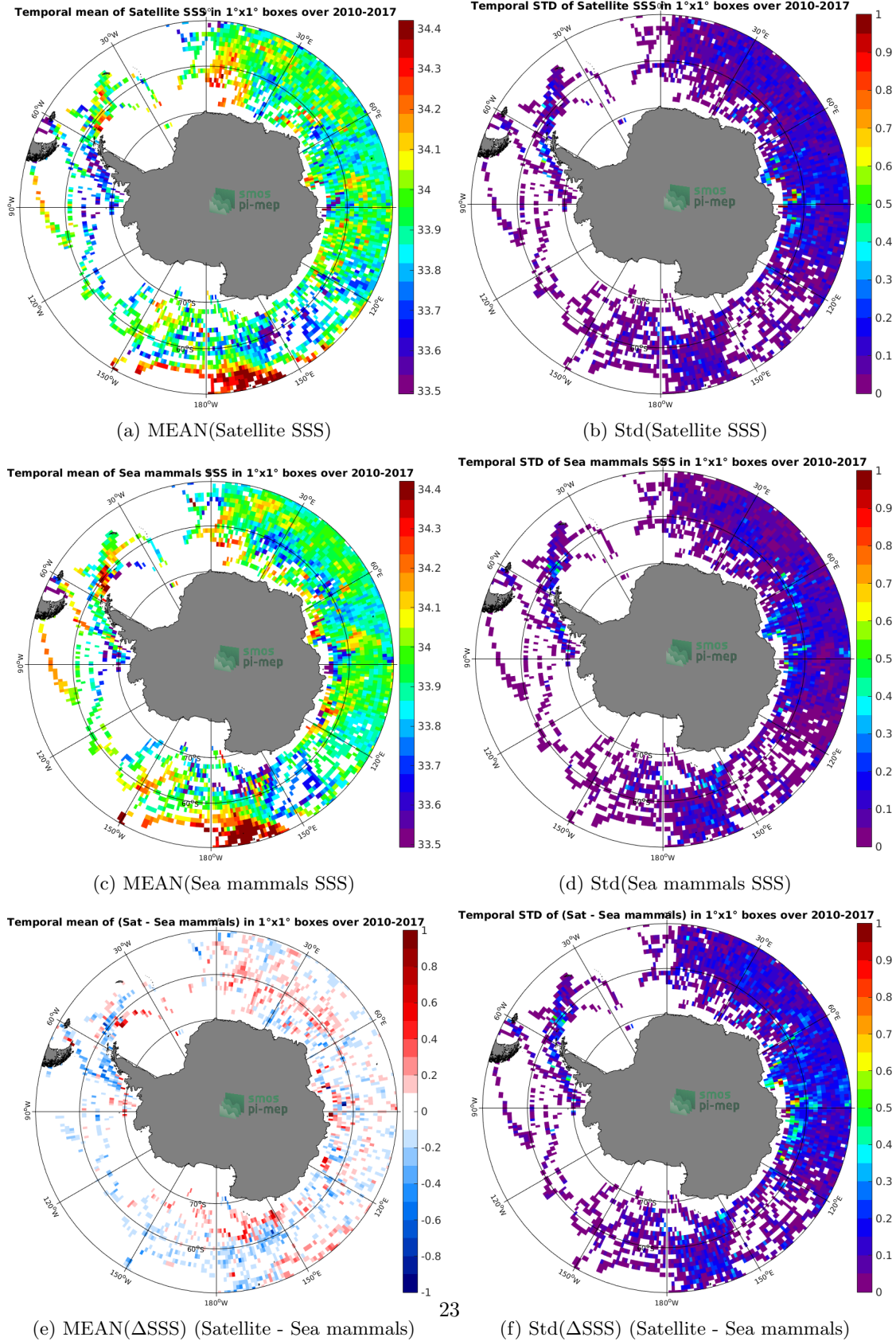
Figure 6: Temporal mean (left) and Std (right) of SSS from CCI L4 Merged-OI v1.8 - 30-day running (ESA) (top), Sea mammals (middle), and of \Delta SSS (Satellite - Sea mammals). Only match-up pairs are used to generate these maps.
