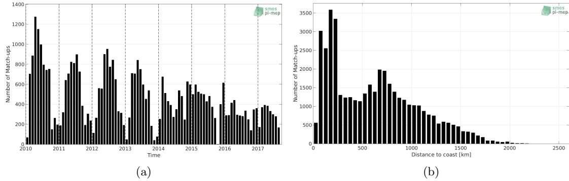
Figure 1: Number of match-ups between Sea mammals and CCI L4 Merged-OI v1.8 - 30-day running (ESA) SSS as a function of time (a) and as function of the distance to coast (b) over the Southern Ocean Pi-MEP region and for the full satellite product period.
