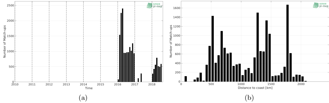
Figure 1: Number of match-ups between Surface drifters and CCI L4 Merged-OI v1.8 - 30-day running (ESA) SSS as a function of time (a) and as function of the distance to coast (b) over the Southern Ocean Pi-MEP region and for the full satellite product period.
