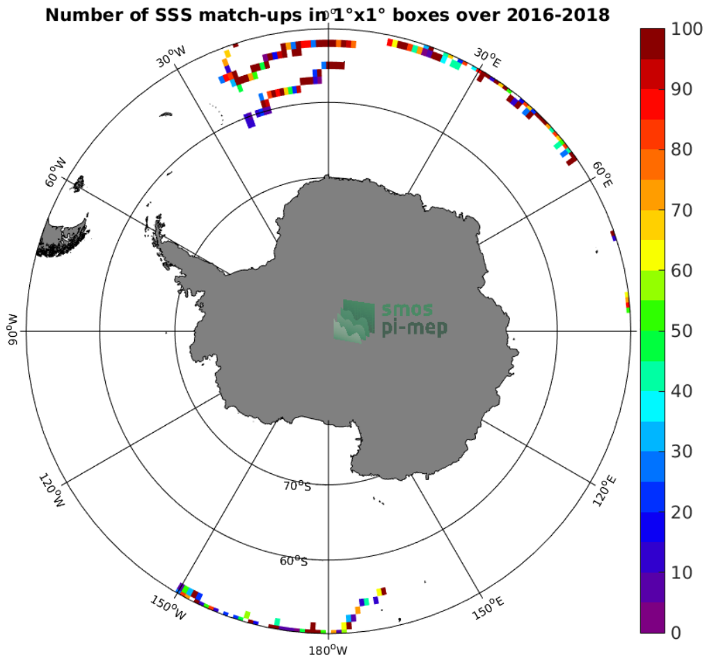
Figure 3: Number of SSS match-ups between Surface drifters SSS and the CCI L4 Merged-OI v1.8 - 30-day running (ESA) SSS product for the Southern Ocean Pi-MEP region over 1°x1° boxes and for the full satellite product period.
