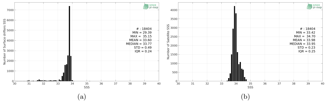
Figure 2: Histograms of SSS from Surface drifters (a) and CCI L4 Merged-OI v1.8 - 30-day running (ESA) (b) considering all match-up pairs per bins of 0.1 over the Southern Ocean Pi-MEP region and for the full satellite product period.
