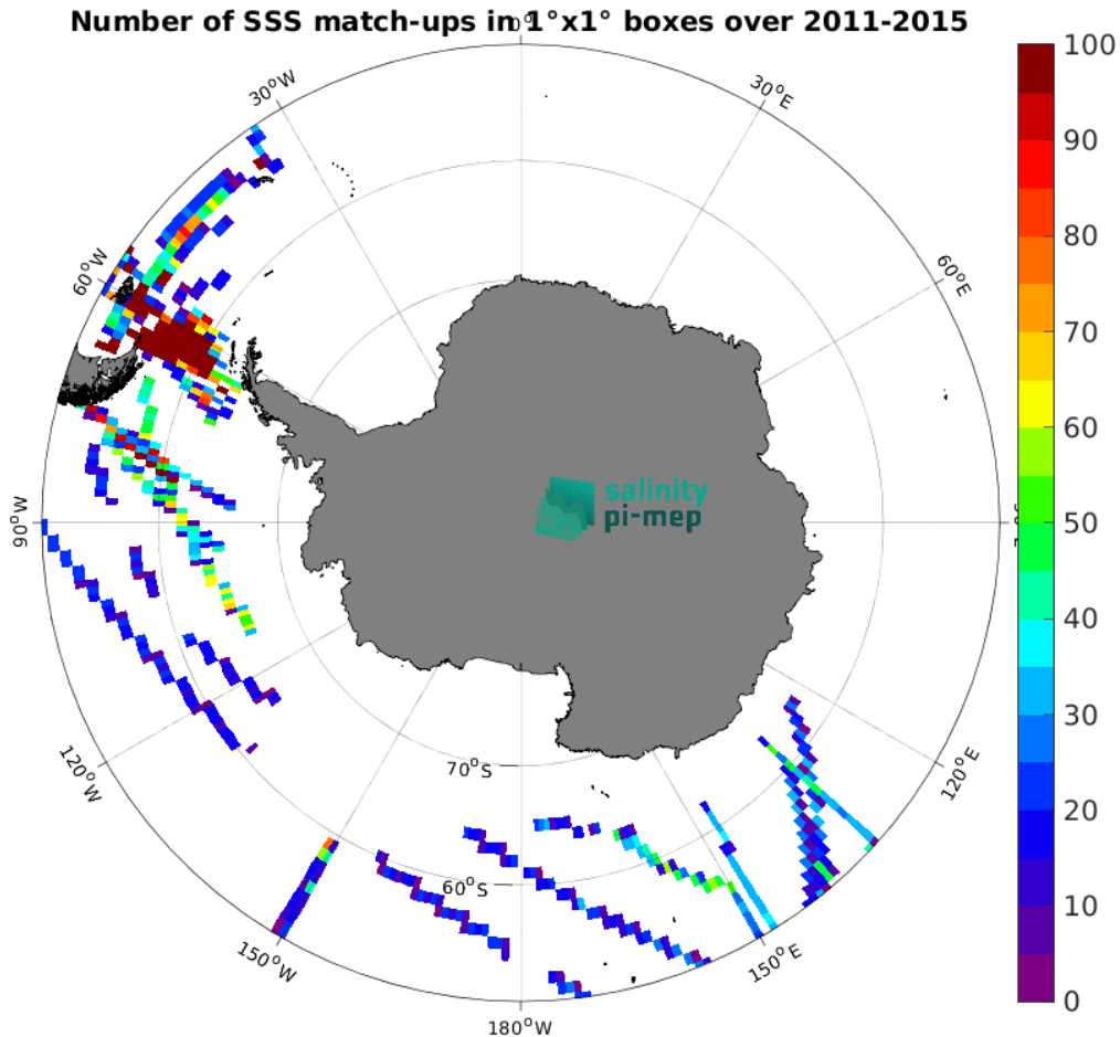
Figure 5: Number of SSS match-ups between TSG (SAMOS) SSS and the Aquarius SSS L4 OI v5 - Weekly (IPRC) SSS product for the Southern Ocean Pi-MEP region over 1^\circ \times 1^\circ boxes and for the full satellite product period.
