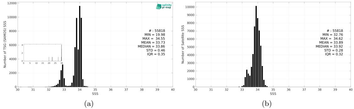
Figure 3: Histograms of SSS from TSG (SAMOS) (a) and Aquarius SSS L4 OI v5 - Weekly (IPRC) (b) considering all match-up pairs per bins of 0.1 over the Southern Ocean Pi-MEP region and for the full satellite product period.
