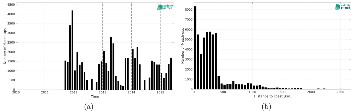
Figure 2: Number of match-ups between TSG (SAMOS) and Aquarius SSS L4 OI v5 - Weekly (IPRC) SSS as a function of time (a) and as function of the distance to coast (b) over the Southern Ocean Pi-MEP region and for the full satellite product period.
