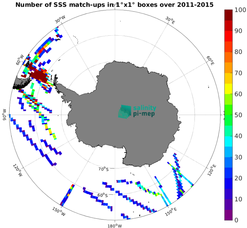
Figure 4: Number of SSS match-ups between TSG (SAMOS) SSS and the Aquarius SSS L4 OI v5 - Weekly (IPRC) SSS product for the Southern Ocean Pi-MEP region over 1^\circ \times 1^\circ boxes and for the full satellite product period.
