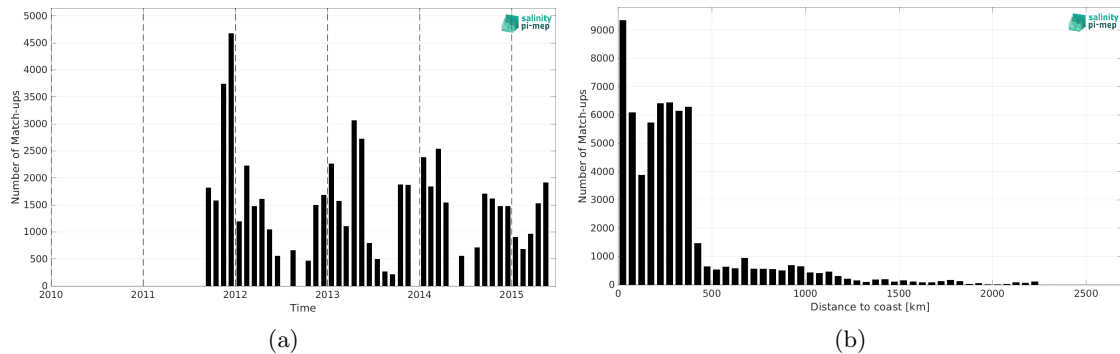
Figure 1: Number of match-ups between TSG (SAMOS) and Aquarius SSS L4 OI v5 - Weekly (IPRC) SSS as a function of time (a) and as function of the distance to coast (b) over the Southern Ocean Pi-MEP region and for the full satellite product period.
