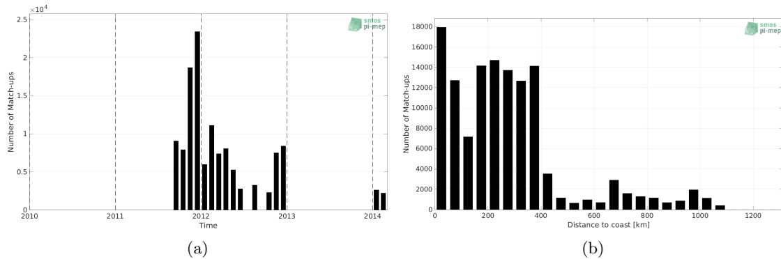
Figure 1: Number of match-ups between TSG (SAMOS) and Aquarius SSS L4 OI v5 - Weekly (IPRC) SSS as a function of time (a) and as function of the distance to coast (b) over the Southern Ocean Pi-MEP region and for the full satellite product period.
