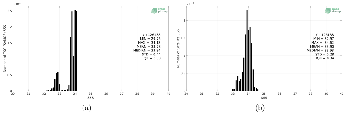
Figure 2: Histograms of SSS from TSG (SAMOS) (a) and Aquarius SSS L4 OI v5 - Weekly (IPRC) (b) considering all match-up pairs per bins of 0.1 over the Southern Ocean Pi-MEP region and for the full satellite product period.
