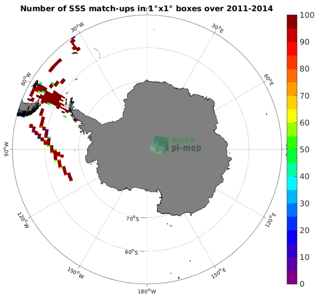
Figure 4: Number of SSS match-ups between TSG (SAMOS) SSS and the Aquarius SSS L4 OI v5 - Weekly (IPRC) SSS product for the Southern Ocean Pi-MEP region over 1^\circ \times 1^\circ boxes and for the full satellite product period.
