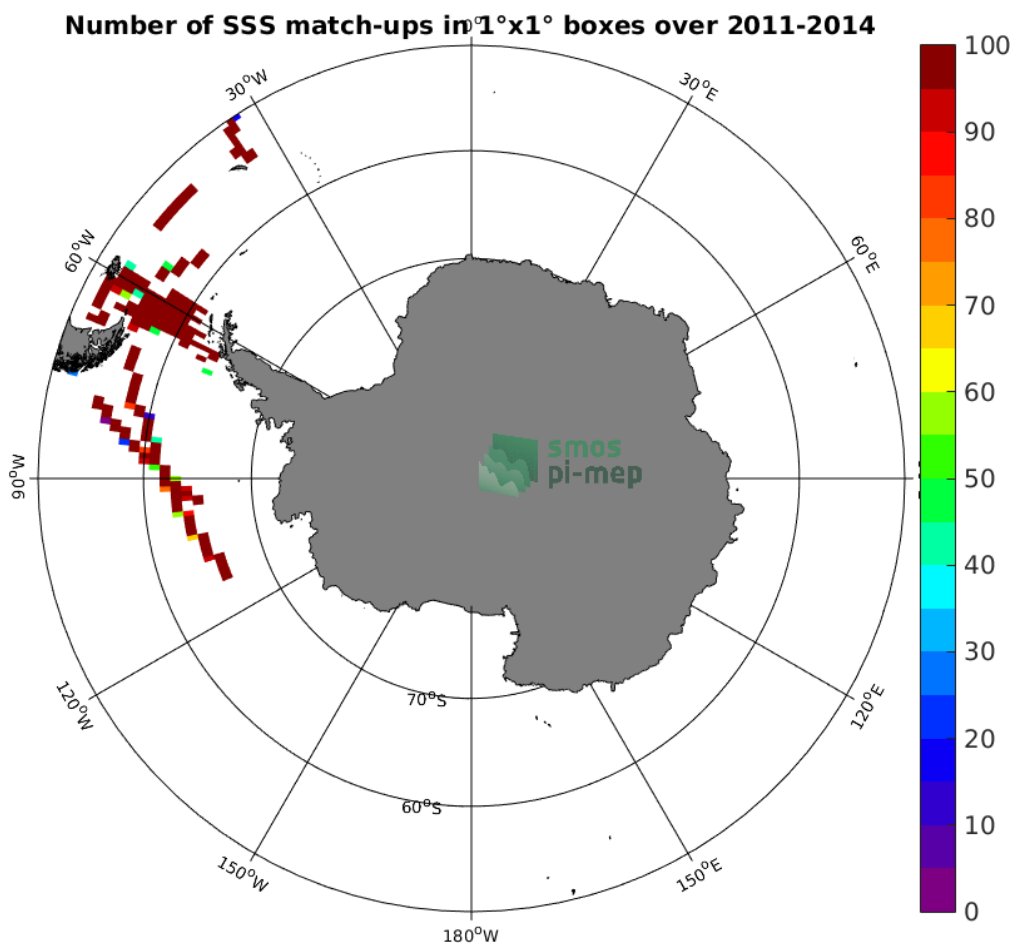
Figure 4: Number of SSS match-ups between TSG-SAMOS SSS and the Aquarius-L4-IPRC-V5-WEEKLY SSS product for the Southern Ocean Pi-MEP region over 1°x1° boxes and for the full satellite product period.
