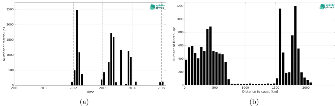
Figure 2: Number of match-ups between TSG (Polarstern) and Aquarius SSS L4 OI v5 - Weekly (IPRC) SSS as a function of time (a) and as function of the distance to coast (b) over the Southern Ocean Pi-MEP region and for the full satellite product period.
