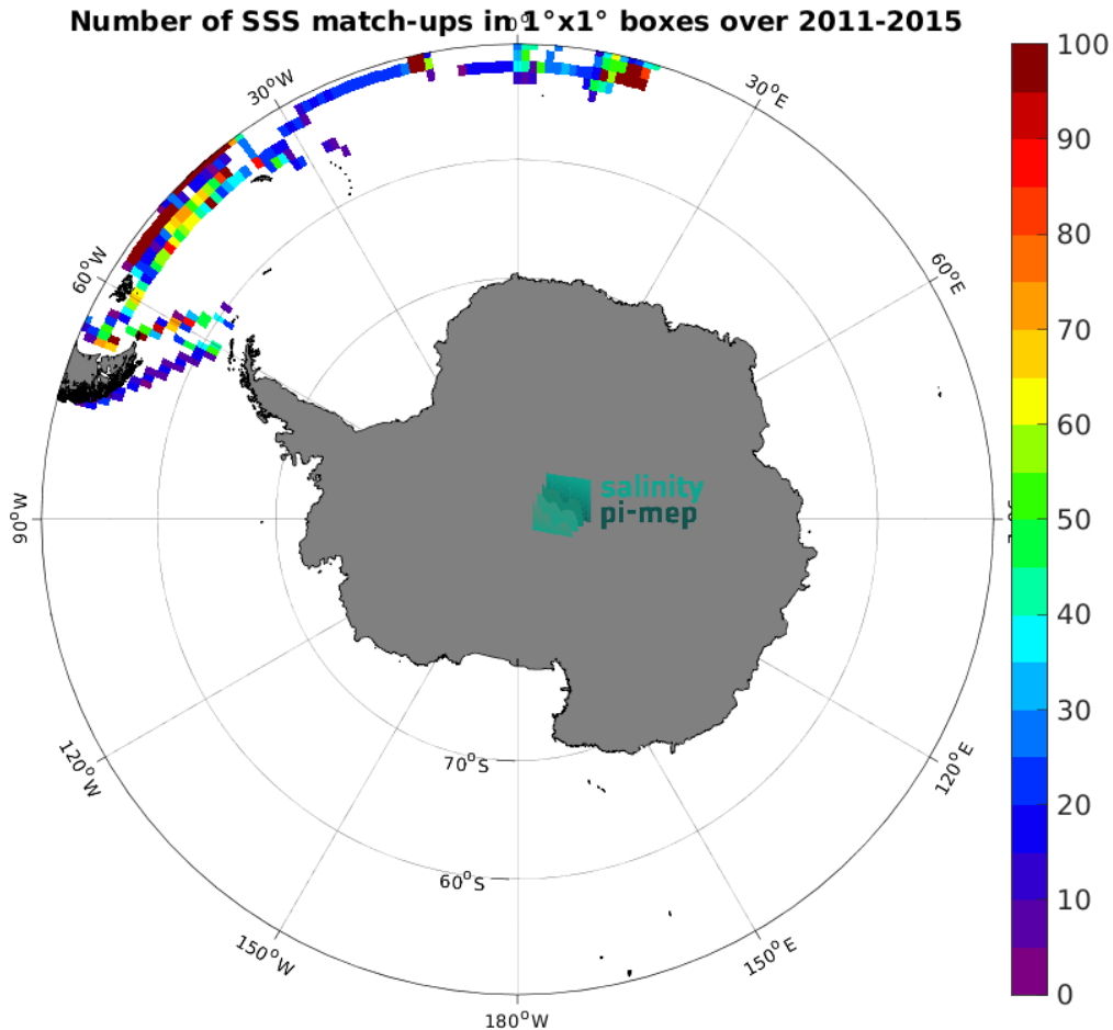
Figure 5: Number of SSS match-ups between TSG (Polarstern) SSS and the Aquarius SSS L4 OI v5 - Weekly (IPRC) SSS product for the Southern Ocean Pi-MEP region over 1^\circ \times 1^\circ boxes and for the full satellite product period.
