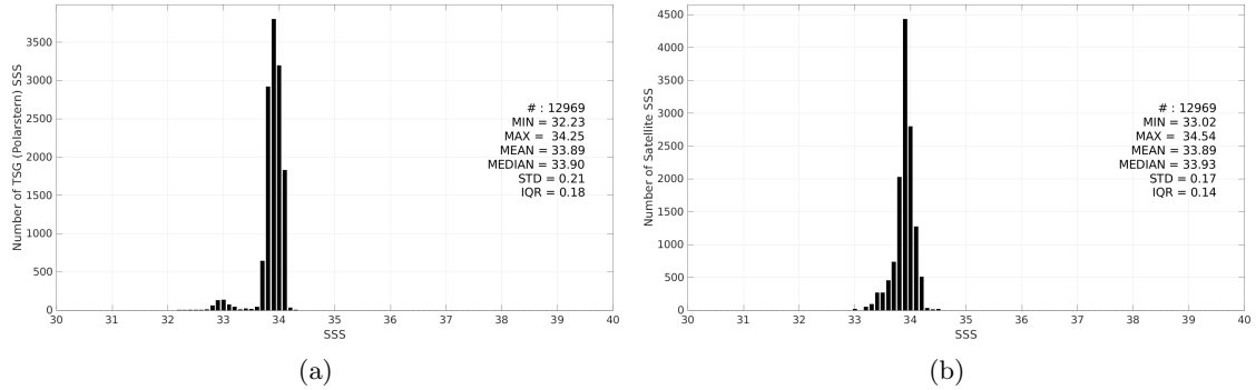
Figure 3: Histograms of SSS from TSG (Polarstern) (a) and Aquarius SSS L4 OI v5 - Weekly (IPRC) (b) considering all match-up pairs per bins of 0.1 over the Southern Ocean Pi-MEP region and for the full satellite product period.
