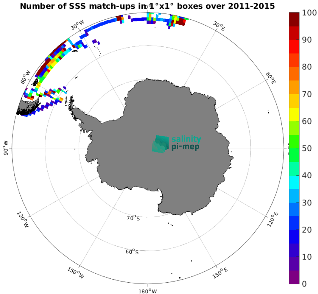
Figure 4: Number of SSS match-ups between TSG (Polarstern) SSS and the Aquarius SSS L4 OI v5 - Weekly (IPRC) SSS product for the Southern Ocean Pi-MEP region over 1^\circ \times 1^\circ boxes and for the full satellite product period.
