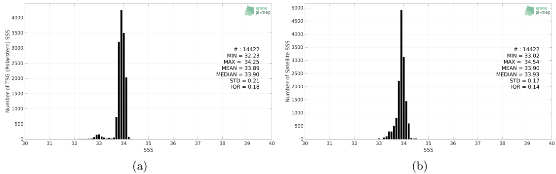
Figure 2: Histograms of SSS from TSG (Polarstern) (a) and Aquarius SSS L4 OI v5 - Weekly (IPRC) (b) considering all match-up pairs per bins of 0.1 over the Southern Ocean Pi-MEP region and for the full satellite product period.
