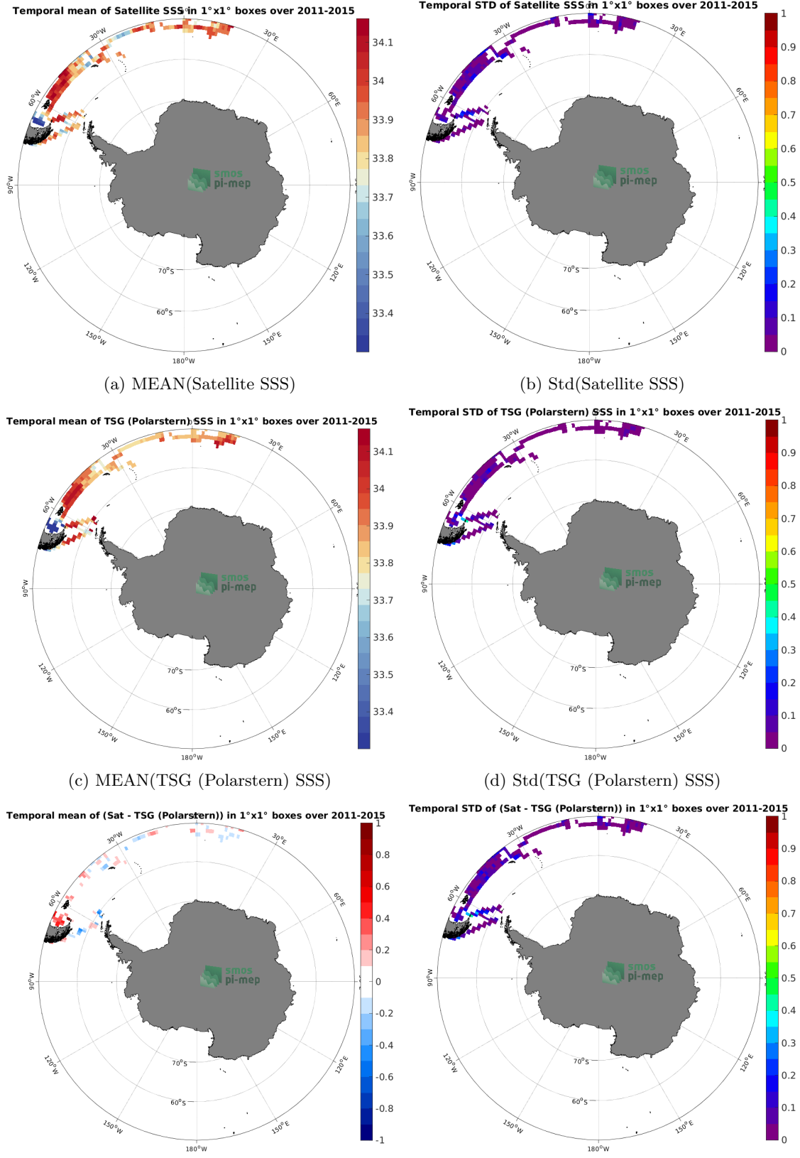
Figure 6: Temporal mean (left) and Std (right) of SSS from Aquarius SSS L4 OI v5 - Weekly (IPRC) (top), TSG (Polarstern) (middle), and of \Delta SSS (Satellite - TSG (Polarstern)). Only match-up pairs are used to generate these maps.
