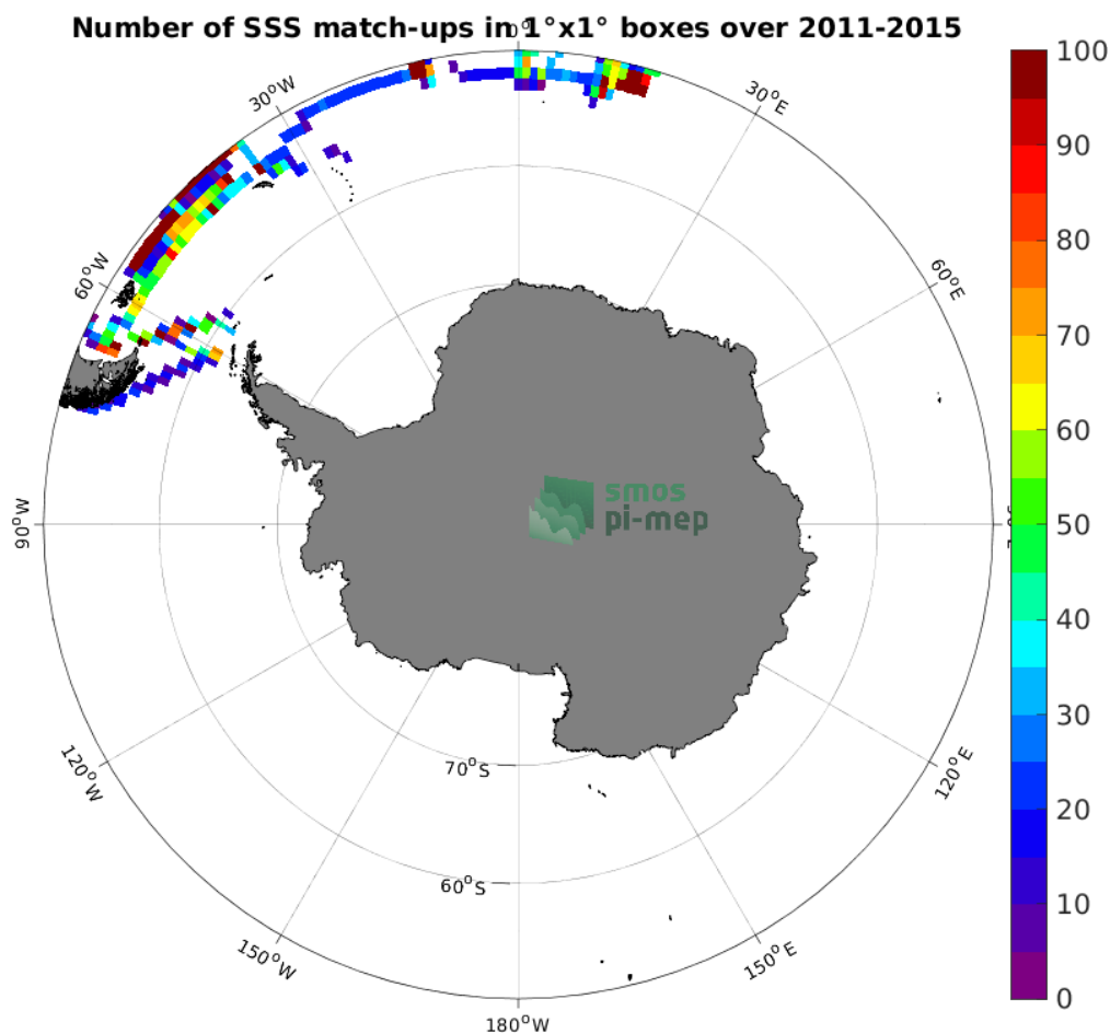
Figure 4: Number of SSS match-ups between TSG (Polarstern) SSS and the Aquarius SSS L4 OI v5 - Weekly (IPRC) SSS product for the Southern Ocean Pi-MEP region over 1^\circ \times 1^\circ boxes and for the full satellite product period.
