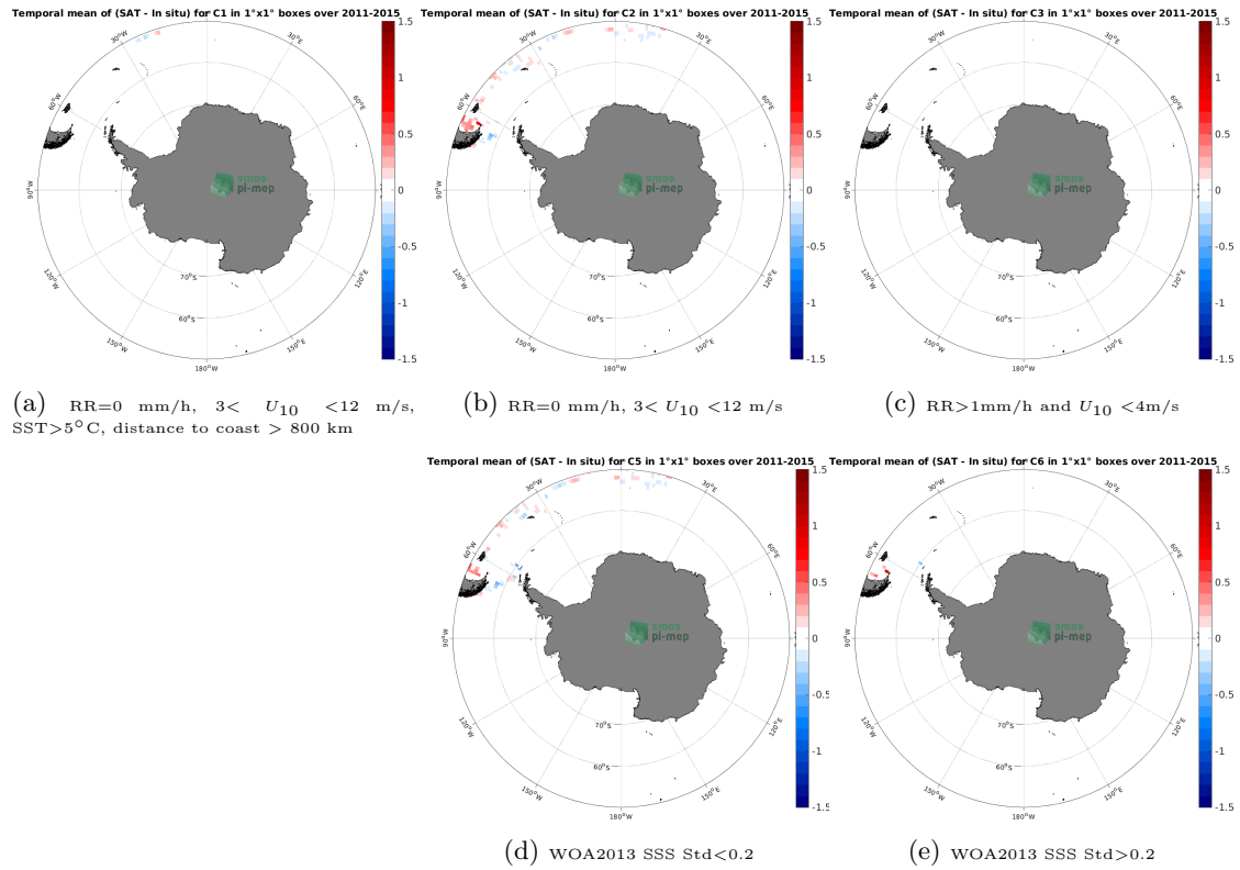
Figure 12: Temporal mean gridded over spatial boxes of size 1^{\circ}\times 1^{\circ} of \Delta\text{SSS} (Aquarius SSS L4 OI v5 - Weekly (IPRC) - TSG (Polarstern)) for 5 different subdatasets corresponding to:RR=0 mm/h, 3 < U_{10} < 12 m/s, SST >5^{\circ}\text{C} , distance to coast > 800 km (a), RR=0 mm/h, 3 < U_{10} < 12 m/s (b), RR >1 mm/h and U_{10} < 4 m/s (c), WOA2013 SSS Std <0.2 (d), WOA2013 SSS Std >0.2 (e).
