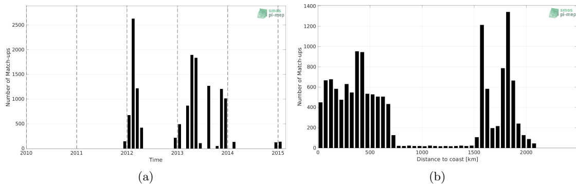
Figure 1: Number of match-ups between TSG (Polarstern) and Aquarius SSS L4 OI v5 - Weekly (IPRC) SSS as a function of time (a) and as function of the distance to coast (b) over the Southern Ocean Pi-MEP region and for the full satellite product period.
