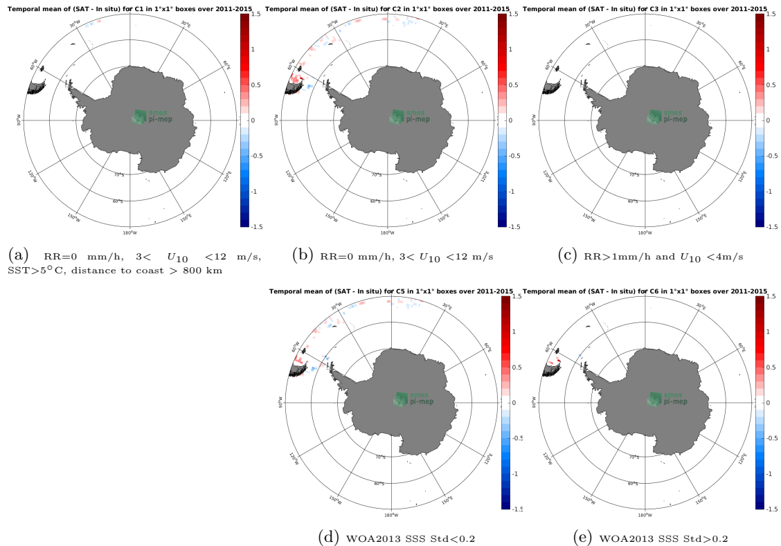
Figure 12: Temporal mean gridded over spatial boxes of size 1^\circ \times 1^\circ of \Delta SSS (Aquarius-L4-IPRC-V5-WEEKLY - TSG-POLARSTERN) for 5 different subdatasets corresponding to:RR=0 mm/h, 3 < U_{10} < 12 m/s, SST >5^\circ C, distance to coast > 800 km (a), RR=0 mm/h, 3 < U_{10} < 12 m/s (b), RR >1 mm/h and U_{10} < 4 m/s (c), WOA2013 SSS Std <0.2 (d), WOA2013 SSS Std >0.2 (e).
