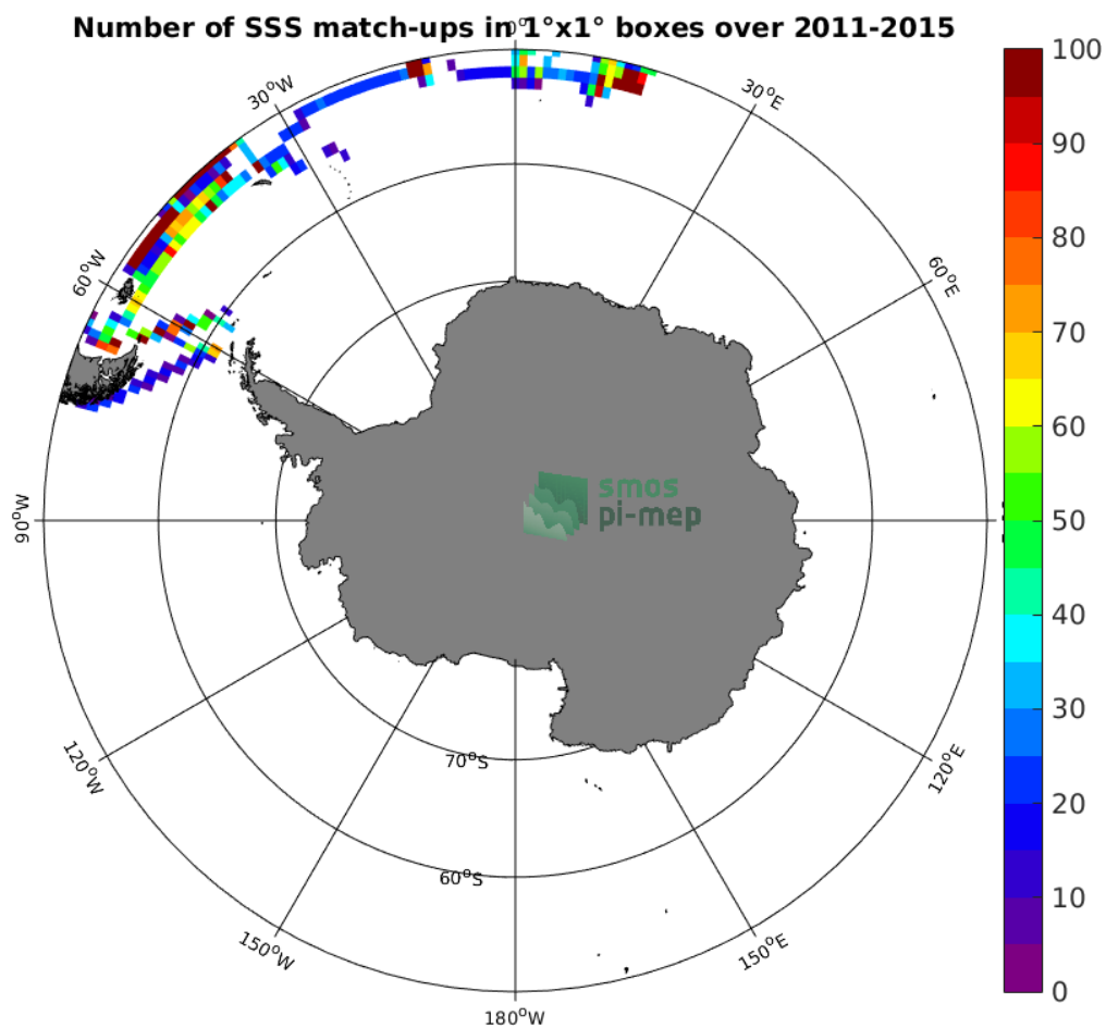
Figure 4: Number of SSS match-ups between TSG-POLARSTERN SSS and the Aquarius-L4-IPRC-V5-WEEKLY SSS product for the Southern Ocean Pi-MEP region over 1^\circ \times 1^\circ boxes and for the full satellite product period.
