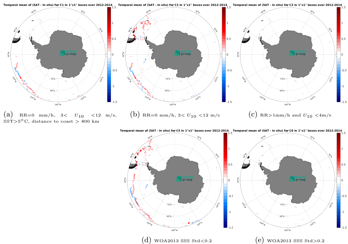
Figure 14: Temporal mean gridded over spatial boxes of size 1^\circ \times 1^\circ of \Delta SSS (Aquarius SSS L4 OI v5 - Weekly (IPRC) - TSG (GOSUD-Sailing-ship)) for 5 different subdatasets corresponding to:RR=0 mm/h, 3 < U_{10} < 12 m/s, SST >5^\circ C, distance to coast > 800 km (a), RR=0 mm/h, 3 < U_{10} < 12 m/s (b), RR >1 mm/h and U_{10} < 4 m/s (c), WOA2013 SSS Std <0.2 (d), WOA2013 SSS Std >0.2 (e).
