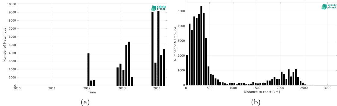
Figure 2: Number of match-ups between TSG (GOSUD-Sailing-ship) and Aquarius SSS L4 OI v5 - Weekly (IPRC) SSS as a function of time (a) and as function of the distance to coast (b) over the Southern Ocean Pi-MEP region and for the full satellite product period.
