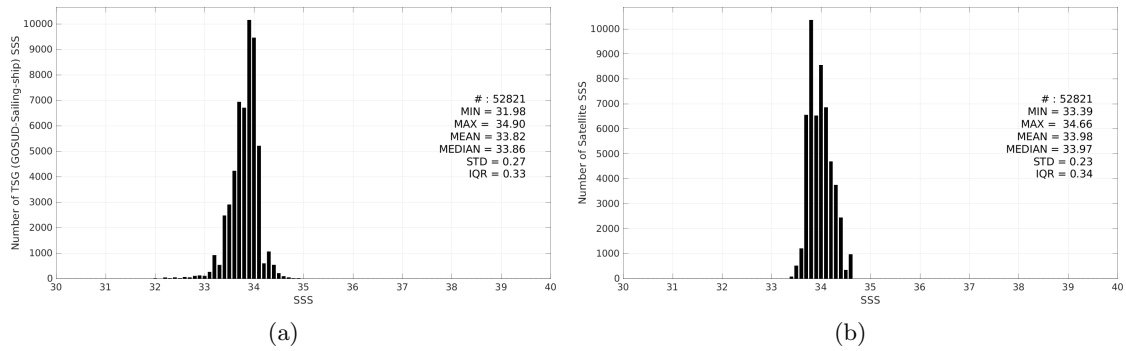
Figure 3: Histograms of SSS from TSG (GOSUD-Sailing-ship) (a) and Aquarius SSS L4 OI v5 - Weekly (IPRC) (b) considering all match-up pairs per bins of 0.1 over the Southern Ocean Pi-MEP region and for the full satellite product period.
