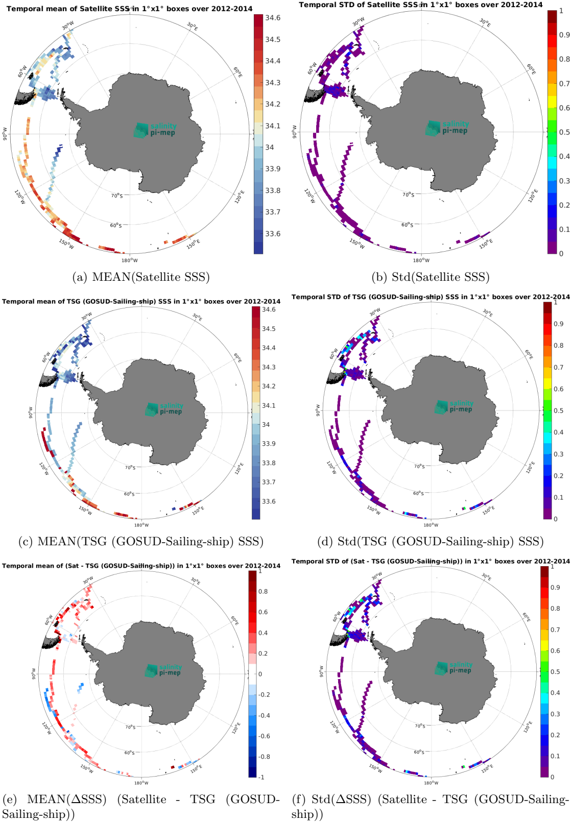
Figure 7: Temporal mean (left) and Std (right) of SSS from Aquarius SSS L4 OI v5 - Weekly (IPRC) (top), TSG (GOSUD-Sailing-ship) (middle), and of \Delta SSS (Satellite - TSG (GOSUD-Sailing-ship)). Only match-up pairs are used to generate these maps.
