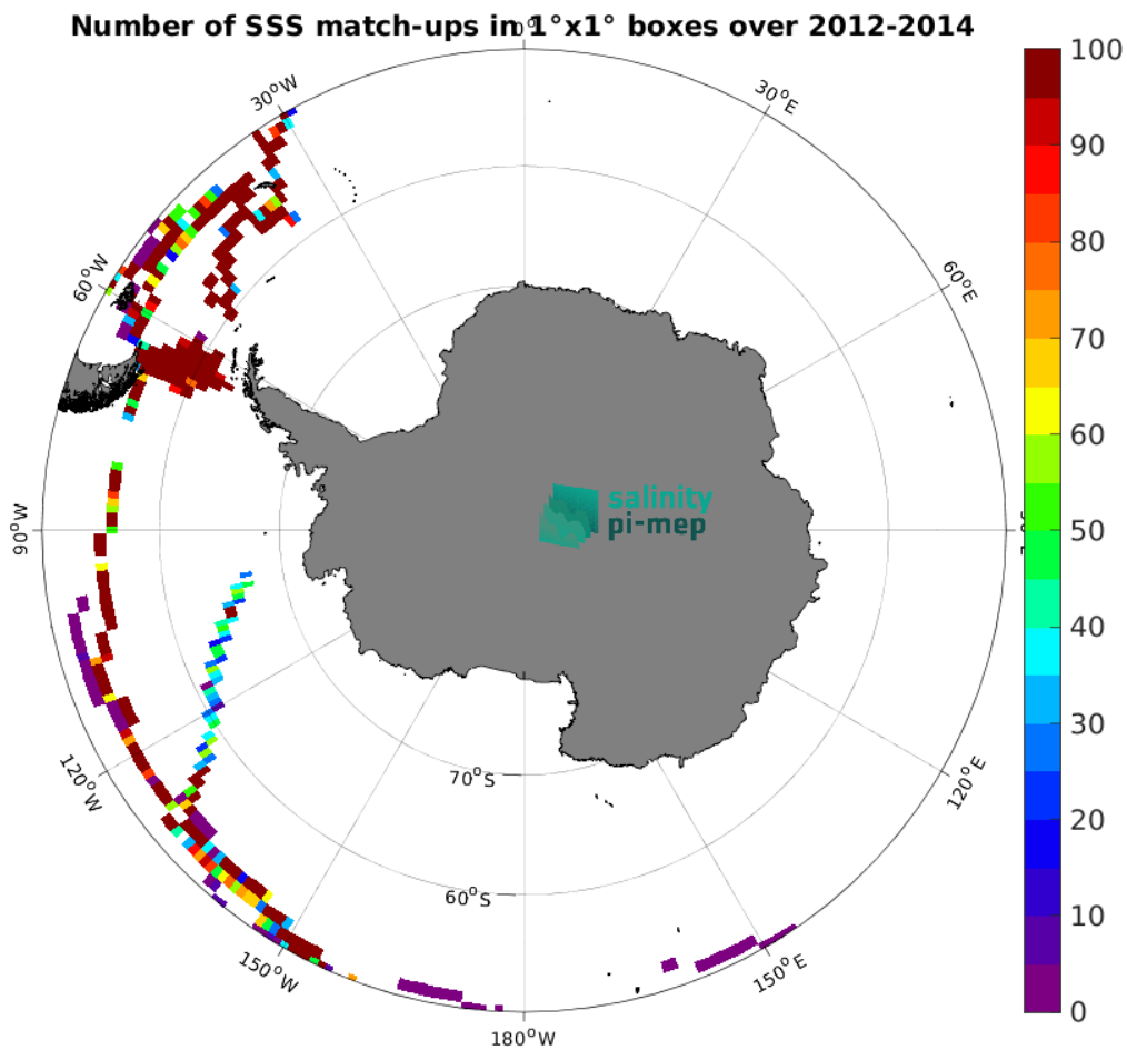
Figure 5: Number of SSS match-ups between TSG (GOSUD-Sailing-ship) SSS and the Aquarius SSS L4 OI v5 - Weekly (IPRC) SSS product for the Southern Ocean Pi-MEP region over 1^\circ \times 1^\circ boxes and for the full satellite product period.
