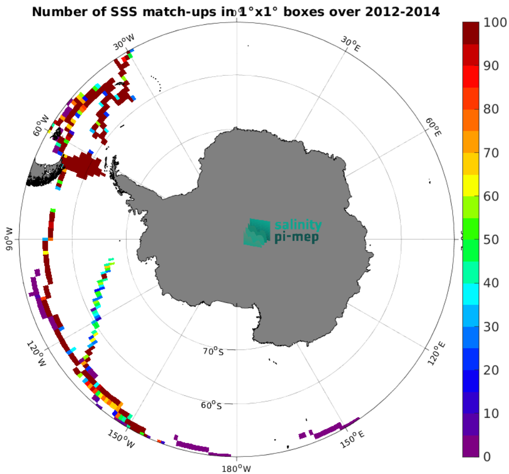
Figure 4: Number of SSS match-ups between TSG (GOSUD-Sailing-ship) SSS and the Aquarius SSS L4 OI v5 - Weekly (IPRC) SSS product for the Southern Ocean Pi-MEP region over 1^\circ \times 1^\circ boxes and for the full satellite product period.
