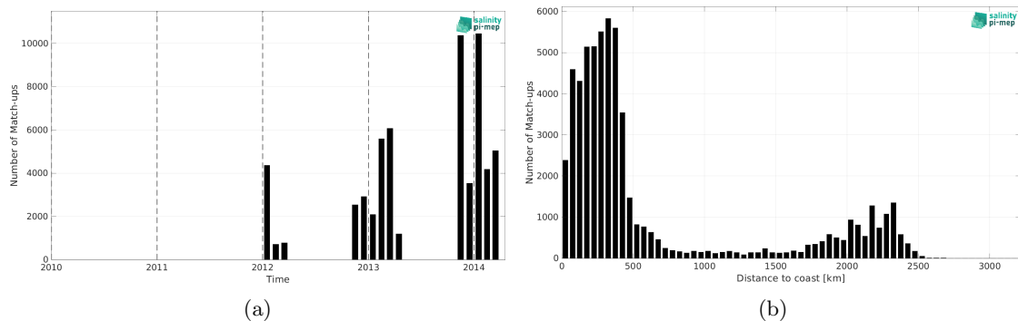
Figure 1: Number of match-ups between TSG (GOSUD-Sailing-ship) and Aquarius SSS L4 OI v5 - Weekly (IPRC) SSS as a function of time (a) and as function of the distance to coast (b) over the Southern Ocean Pi-MEP region and for the full satellite product period.
