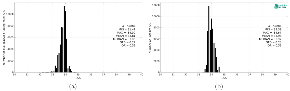
Figure 2: Histograms of SSS from TSG (GOSUD-Sailing-ship) (a) and Aquarius SSS L4 OI v5 - Weekly (IPRC) (b) considering all match-up pairs per bins of 0.1 over the Southern Ocean Pi-MEP region and for the full satellite product period.
