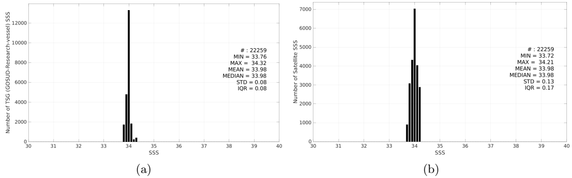
Figure 3: Histograms of SSS from TSG (GOSUD-Research-vessel) (a) and Aquarius SSS L4 OI v5 - Weekly (IPRC) (b) considering all match-up pairs per bins of 0.1 over the Southern Ocean Pi-MEP region and for the full satellite product period.
