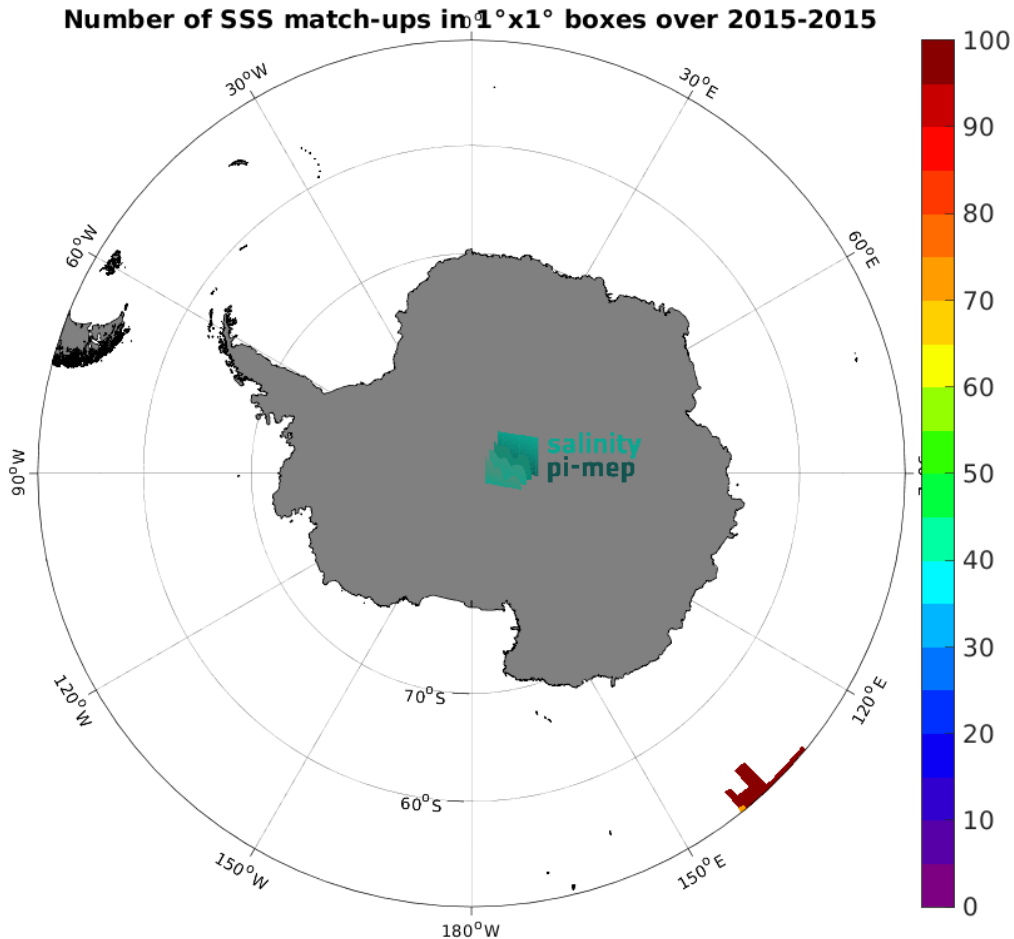
Figure 5: Number of SSS match-ups between TSG (GOSUD-Research-vessel) SSS and the Aquarius SSS L4 OI v5 - Weekly (IPRC) SSS product for the Southern Ocean Pi-MEP region over 1^\circ \times 1^\circ boxes and for the full satellite product period.
