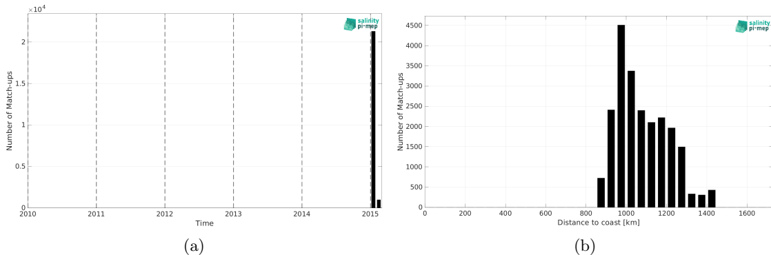
Figure 2: Number of match-ups between TSG (GOSUD-Research-vessel) and Aquarius SSS L4 OI v5 - Weekly (IPRC) SSS as a function of time (a) and as function of the distance to coast (b) over the Southern Ocean Pi-MEP region and for the full satellite product period.
