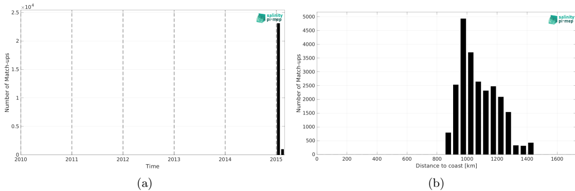
Figure 1: Number of match-ups between TSG (GOSUD-Research-vessel) and Aquarius SSS L4 OI v5 - Weekly (IPRC) SSS as a function of time (a) and as function of the distance to coast (b) over the Southern Ocean Pi-MEP region and for the full satellite product period.
