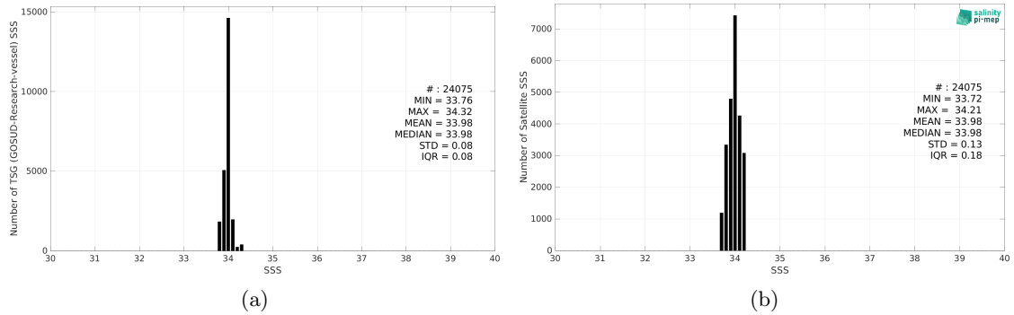
Figure 2: Histograms of SSS from TSG (GOSUD-Research-vessel) (a) and Aquarius SSS L4 OI v5 - Weekly (IPRC) (b) considering all match-up pairs per bins of 0.1 over the Southern Ocean Pi-MEP region and for the full satellite product period.
