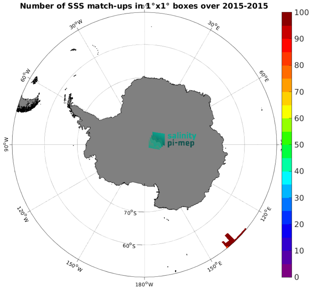
Figure 4: Number of SSS match-ups between TSG (GOSUD-Research-vessel) SSS and the Aquarius SSS L4 OI v5 - Weekly (IPRC) SSS product for the Southern Ocean Pi-MEP region over 1^\circ \times 1^\circ boxes and for the full satellite product period.
