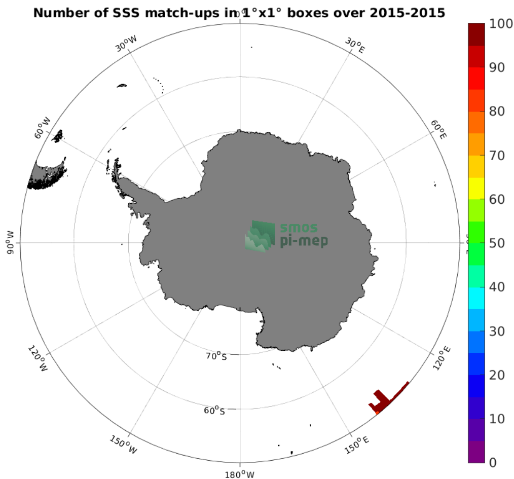
Figure 4: Number of SSS match-ups between TSG (GOSUD-Research-vessel) SSS and the Aquarius SSS L4 OI v5 - Weekly (IPRC) SSS product for the Southern Ocean Pi-MEP region over 1^\circ \times 1^\circ boxes and for the full satellite product period.
