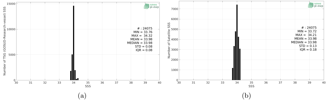
Figure 2: Histograms of SSS from TSG (GOSUD-Research-vessel) (a) and Aquarius SSS L4 OI v5 - Weekly (IPRC) (b) considering all match-up pairs per bins of 0.1 over the Southern Ocean Pi-MEP region and for the full satellite product period.
