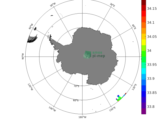
(c) MEAN(TSG (GOSUD-Research-vessel) SSS)
