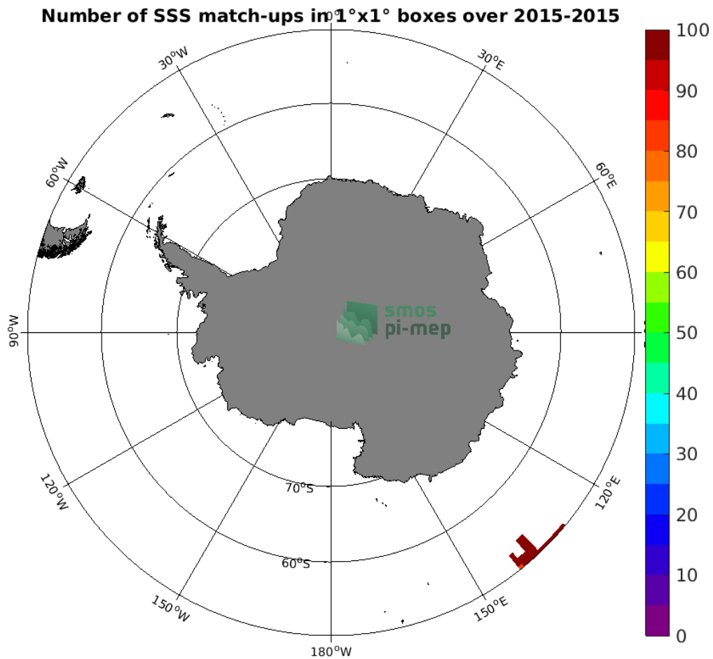
Figure 4: Number of SSS match-ups between TSG (GOSUD-Research-vessel) SSS and the Aquarius SSS L4 OI v5 - Weekly (IPRC) SSS product for the Southern Ocean Pi-MEP region over 1°x1° boxes and for the full satellite product period.
