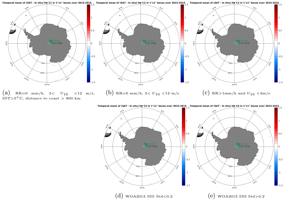
Figure 12: Temporal mean gridded over spatial boxes of size 1°x1° of \Delta SSS (Aquarius-L4-IPRC-V5-WEEKLY - TSG-GOSUD-Research-vessel) for 5 different subdatasets corresponding to:RR=0 mm/h, 3 < U_{10} < 12 m/s, SST>5°C, distance to coast > 800 km (a), RR=0 mm/h, 3 < U_{10} < 12 m/s (b), RR>1mm/h and U_{10} < 4 m/s (c), WOA2013 SSS Std<0.2 (d), WOA2013 SSS Std>0.2 (e).
