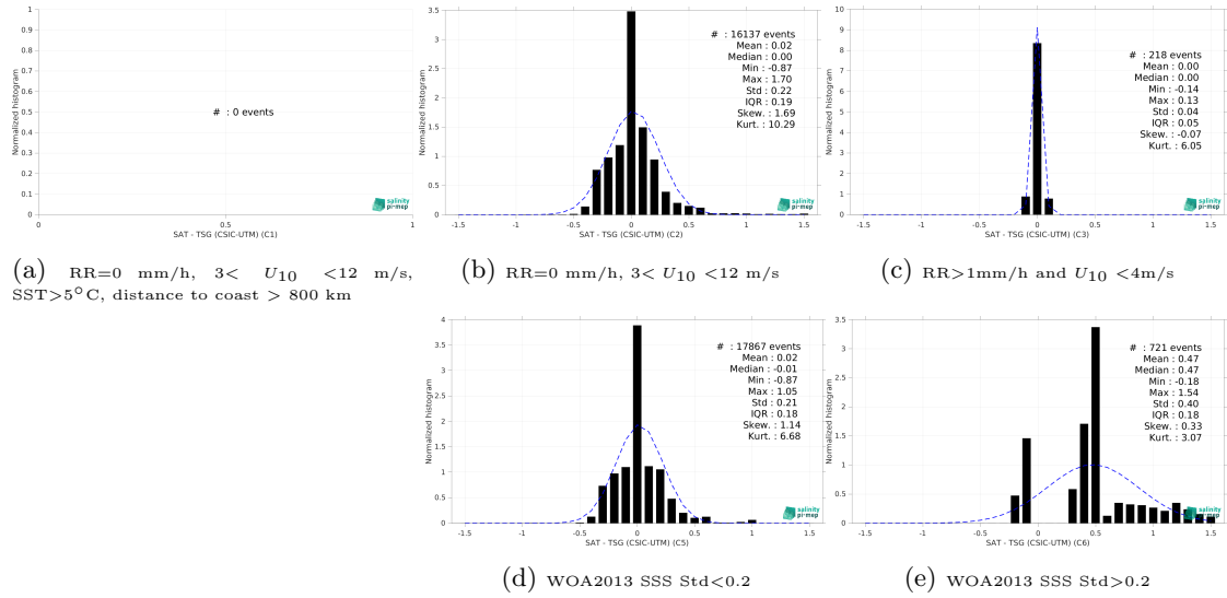
Figure 15: Normalized histogram of \Delta SSS (Aquarius SSS L4 OI v5 - Weekly (IPRC) - TSG (CSIC-UTM)) for 5 different subdatasets corresponding to: RR=0 mm/h, 3 < U_{10} < 12 m/s, SST > 5°C, distance to coast > 800 km (a), RR=0 mm/h, 3 < U_{10} < 12 m/s (b), RR > 1mm/h and U_{10} < 4 m/s (c), WOA2013 SSS Std < 0.2 (d), WOA2013 SSS Std > 0.2 (e).
