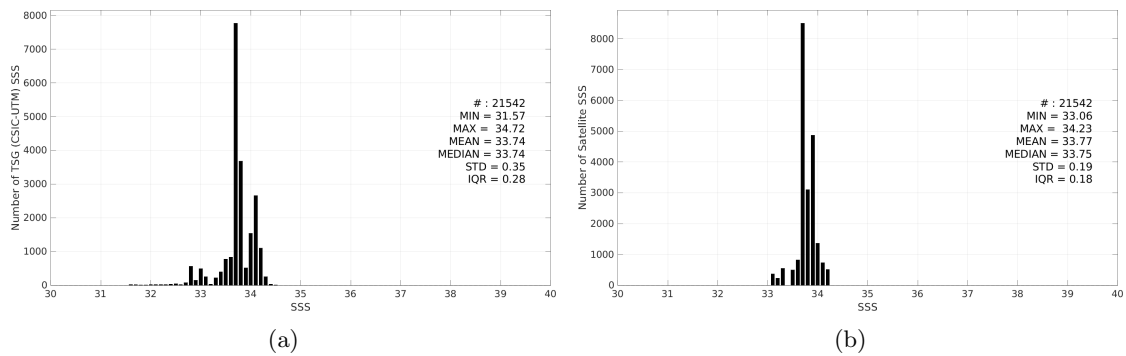
Figure 3: Histograms of SSS from TSG (CSIC-UTM) (a) and Aquarius SSS L4 OI v5 - Weekly (IPRC) (b) considering all match-up pairs per bins of 0.1 over the Southern Ocean Pi-MEP region and for the full satellite product period.
