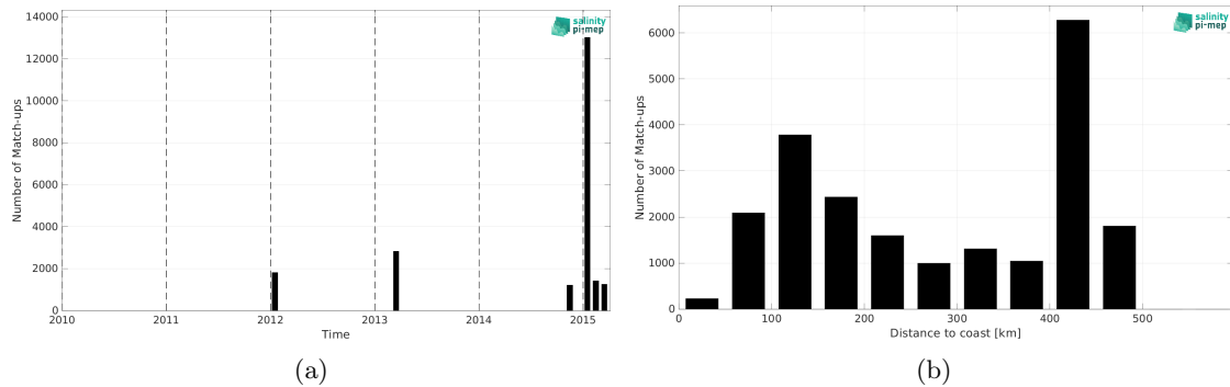
Figure 2: Number of match-ups between TSG (CSIC-UTM) and Aquarius SSS L4 OI v5 - Weekly (IPRC) SSS as a function of time (a) and as function of the distance to coast (b) over the Southern Ocean Pi-MEP region and for the full satellite product period.
