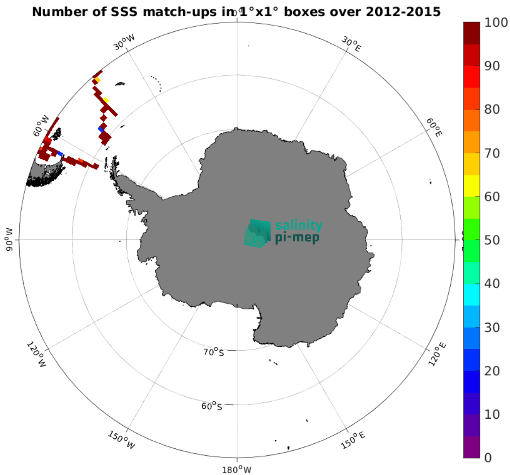
Figure 5: Number of SSS match-ups between TSG (CSIC-UTM) SSS and the Aquarius SSS L4 OI v5 - Weekly (IPRC) SSS product for the Southern Ocean Pi-MEP region over 1^{\circ} \times 1^{\circ} boxes and for the full satellite product period.
