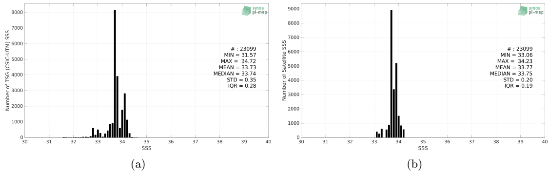
Figure 2: Histograms of SSS from TSG (CSIC-UTM) (a) and Aquarius SSS L4 OI v5 - Weekly (IPRC) (b) considering all match-up pairs per bins of 0.1 over the Southern Ocean Pi-MEP region and for the full satellite product period.
