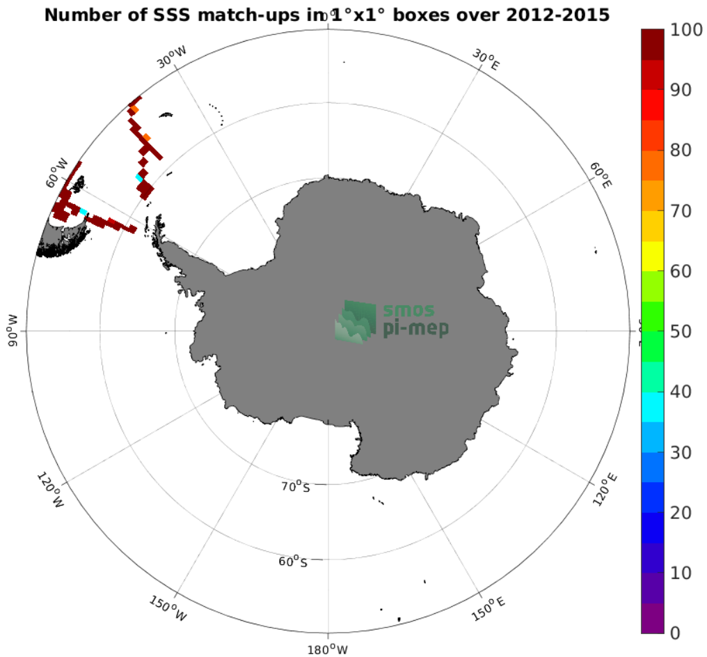
Figure 4: Number of SSS match-ups between TSG (CSIC-UTM) SSS and the Aquarius SSS L4 OI v5 - Weekly (IPRC) SSS product for the Southern Ocean Pi-MEP region over 1^\circ \times 1^\circ boxes and for the full satellite product period.
