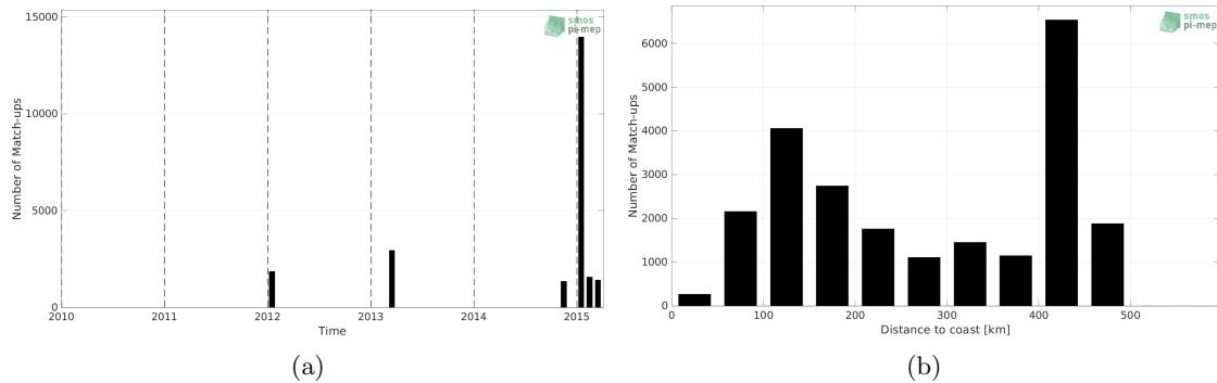
Figure 1: Number of match-ups between TSG (CSIC-UTM) and Aquarius SSS L4 OI v5 - Weekly (IPRC) SSS as a function of time (a) and as function of the distance to coast (b) over the Southern Ocean Pi-MEP region and for the full satellite product period.
