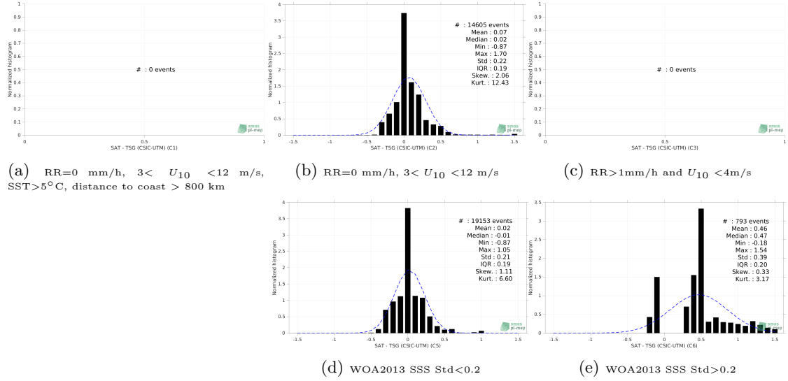
Figure 13: Normalized histogram of \Delta SSS (Aquarius SSS L4 OI v5 - Weekly (IPRC) - TSG (CSIC-UTM)) for 5 different subdatasets corresponding to: RR=0 mm/h, 3 < U_{10} < 12 m/s, SST > 5°C, distance to coast > 800 km (a), RR=0 mm/h, 3 < U_{10} < 12 m/s (b), RR > 1mm/h and U_{10} < 4 m/s (c), WOA2013 SSS Std < 0.2 (d), WOA2013 SSS Std > 0.2 (e).
