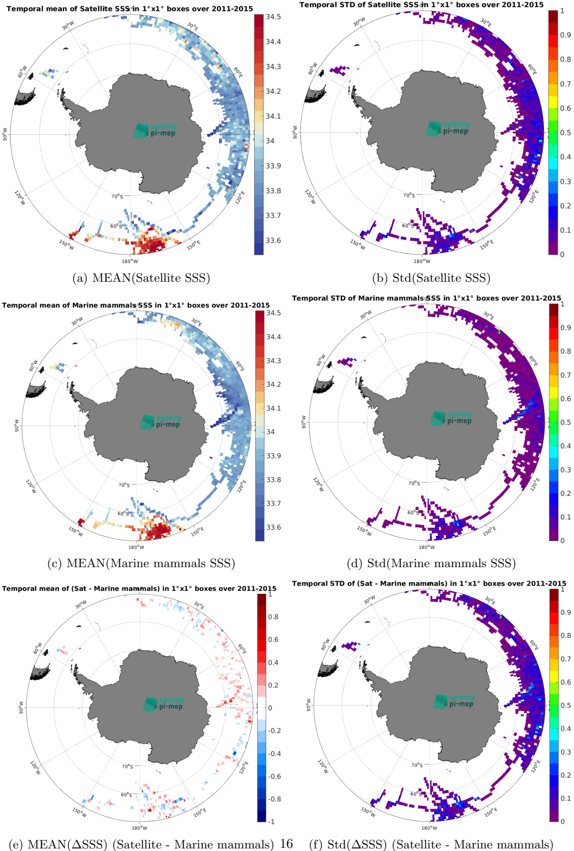
Figure 7: Temporal mean (left) and Std (right) of SSS from Aquarius SSS L4 OI v5 - Weekly (IPRC) (top), Marine mammals (middle), and of \Delta SSS (Satellite - Marine mammals). Only match-up pairs are used to generate these maps.
