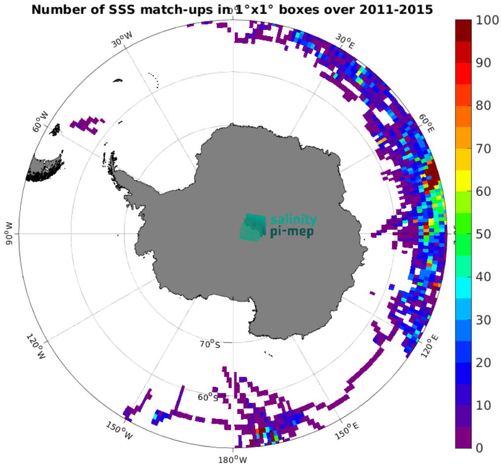
Figure 5: Number of SSS match-ups between Marine mammals SSS and the Aquarius SSS L4 OI v5 - Weekly (IPRC) SSS product for the Southern Ocean Pi-MEP region over 1^\circ \times 1^\circ boxes and for the full satellite product period.
