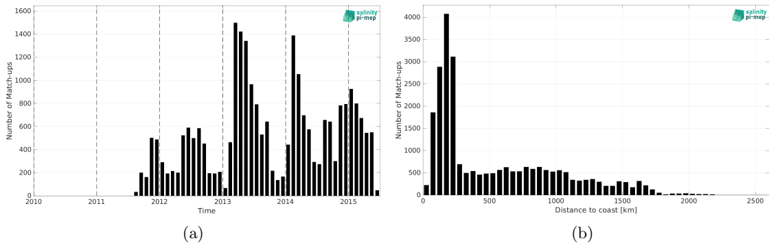
Figure 2: Number of match-ups between Marine mammals and Aquarius SSS L4 OI v5 - Weekly (IPRC) SSS as a function of time (a) and as function of the distance to coast (b) over the Southern Ocean Pi-MEP region and for the full satellite product period.
