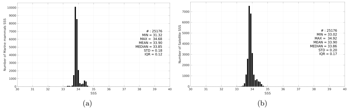
Figure 3: Histograms of SSS from Marine mammals (a) and Aquarius SSS L4 OI v5 - Weekly (IPRC) (b) considering all match-up pairs per bins of 0.1 over the Southern Ocean Pi-MEP region and for the full satellite product period.
