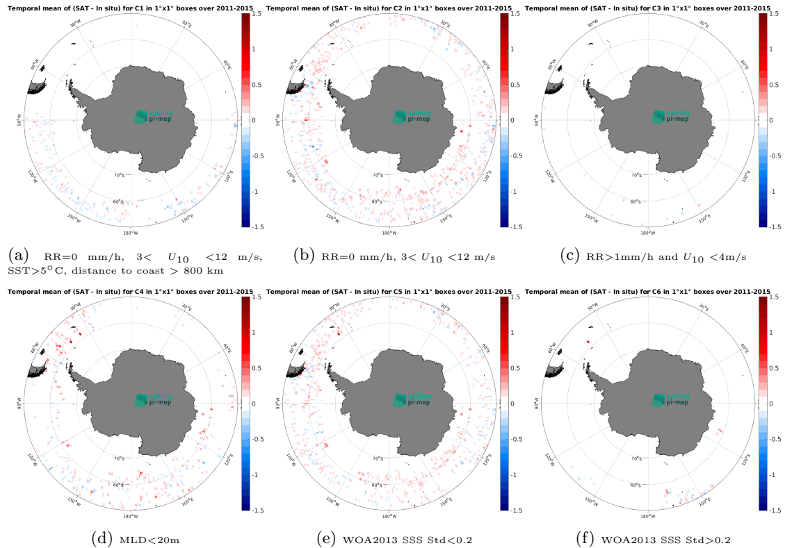
Figure 14: Temporal mean gridded over spatial boxes of size 1^\circ \times 1^\circ of \Delta SSS (Aquarius SSS L4 OI v5 - Weekly (IPRC) - Argo) for 6 different subdatasets corresponding to:RR=0 mm/h, 3 < U_{10} < 12 m/s, SST>5°C, distance to coast > 800 km (a), RR=0 mm/h, 3 < U_{10} < 12 m/s (b), RR>1mm/h and U_{10} < 4 m/s (c),MLD<20m (d),WOA2013 SSS Std<0.2 (e),WOA2013 SSS Std>0.2 (f).
