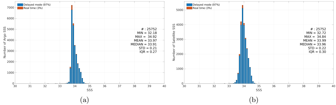
Figure 3: Histograms of SSS from Argo (a) and Aquarius SSS L4 OI v5 - Weekly (IPRC) (b) considering all match-up pairs per bins of 0.1 over the Southern Ocean Pi-MEP region and for the full satellite product period.
