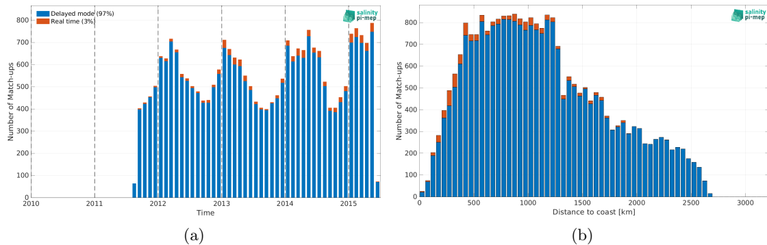
Figure 2: Number of match-ups between Argo and Aquarius SSS L4 OI v5 - Weekly (IPRC) SSS as a function of time (a) and as function of the distance to coast (b) over the Southern Ocean Pi-MEP region and for the full satellite product period.
