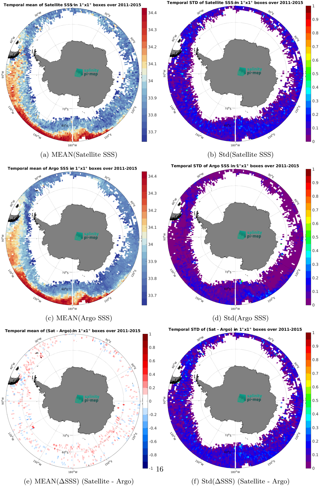
Figure 7: Temporal mean (left) and Std (right) of SSS from Aquarius SSS L4 OI v5 - Weekly (IPRC) (top), Argo (middle), and of \Delta SSS (Satellite - Argo). Only match-up pairs are used to generate these maps.
