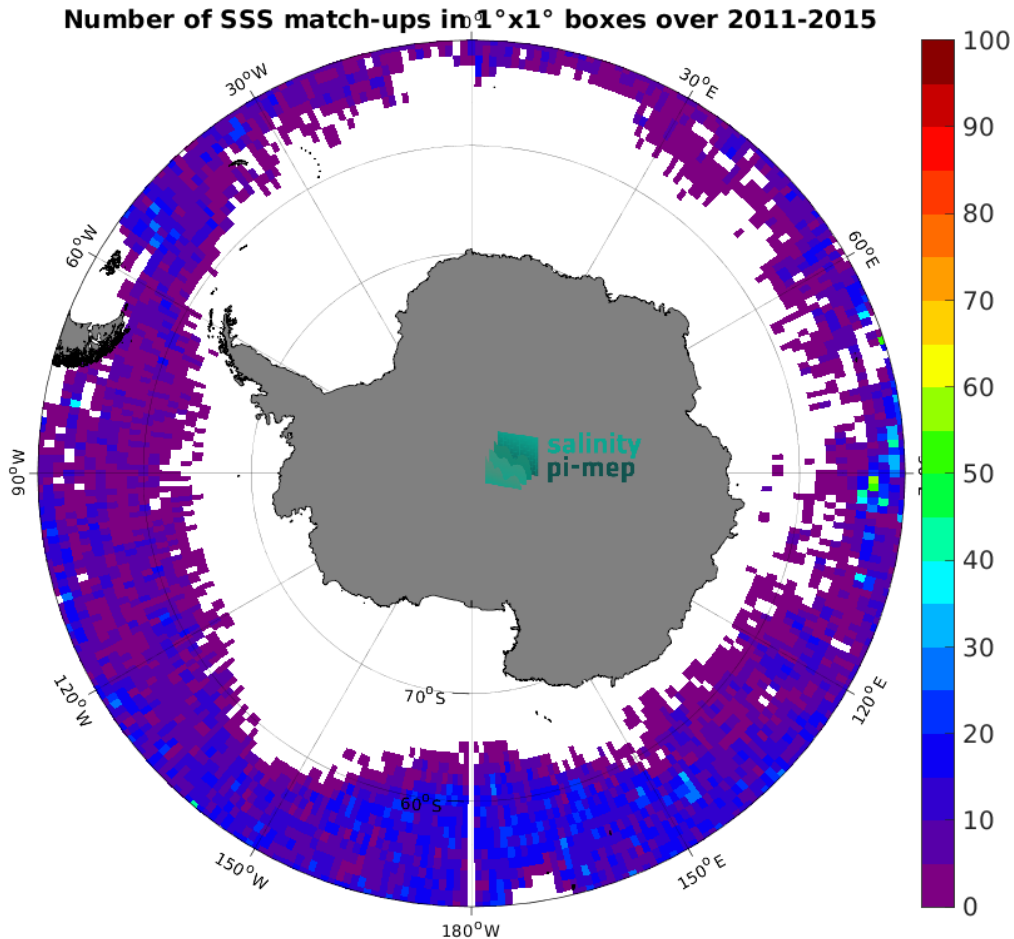
Figure 5: Number of SSS match-ups between Argo SSS and the Aquarius SSS L4 OI v5 - Weekly (IPRC) SSS product for the Southern Ocean Pi-MEP region over 1^\circ \times 1^\circ boxes and for the full satellite product period.
