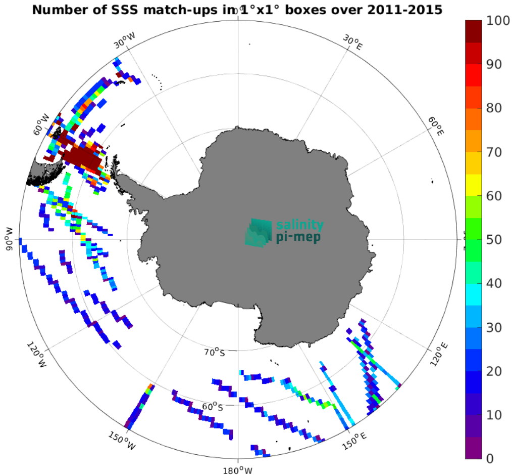
Figure 5: Number of SSS match-ups between TSG (SAMOS) SSS and the Aquarius SSS L4 OI v5 - Monthly (IPRC) SSS product for the Southern Ocean Pi-MEP region over 1^\circ \times 1^\circ boxes and for the full satellite product period.
