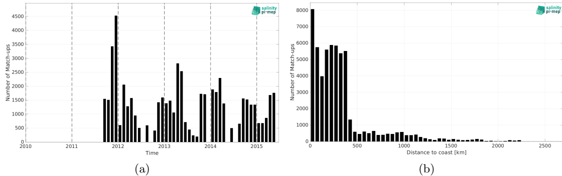
Figure 2: Number of match-ups between TSG (SAMOS) and Aquarius SSS L4 OI v5 - Monthly (IPRC) SSS as a function of time (a) and as function of the distance to coast (b) over the Southern Ocean Pi-MEP region and for the full satellite product period.
