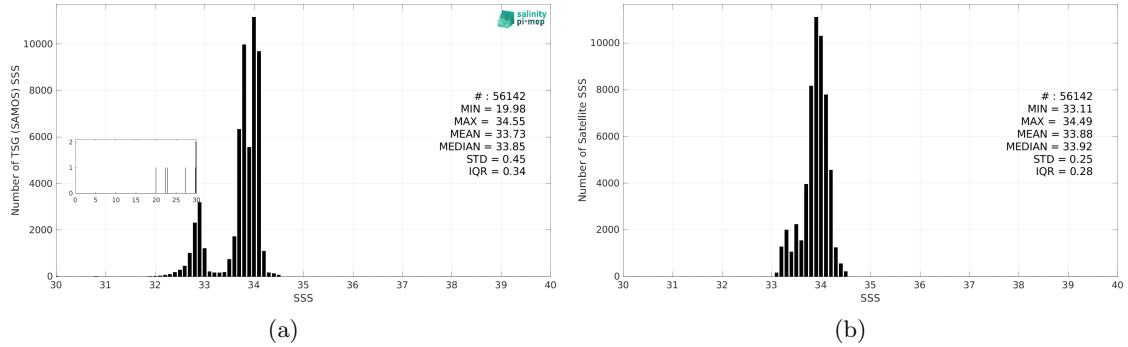
Figure 3: Histograms of SSS from TSG (SAMOS) (a) and Aquarius SSS L4 OI v5 - Monthly (IPRC) (b) considering all match-up pairs per bins of 0.1 over the Southern Ocean Pi-MEP region and for the full satellite product period.
