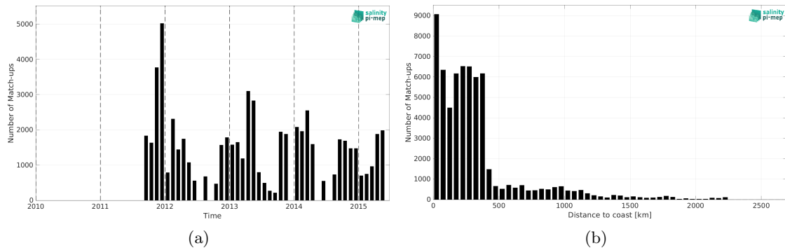
Figure 1: Number of match-ups between TSG (SAMOS) and Aquarius SSS L4 OI v5 - Monthly (IPRC) SSS as a function of time (a) and as function of the distance to coast (b) over the Southern Ocean Pi-MEP region and for the full satellite product period.
