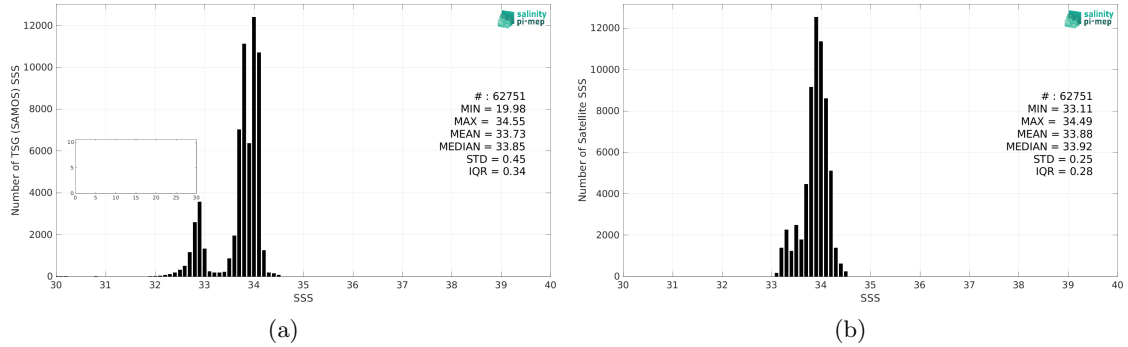
Figure 2: Histograms of SSS from TSG (SAMOS) (a) and Aquarius SSS L4 OI v5 - Monthly (IPRC) (b) considering all match-up pairs per bins of 0.1 over the Southern Ocean Pi-MEP region and for the full satellite product period.
