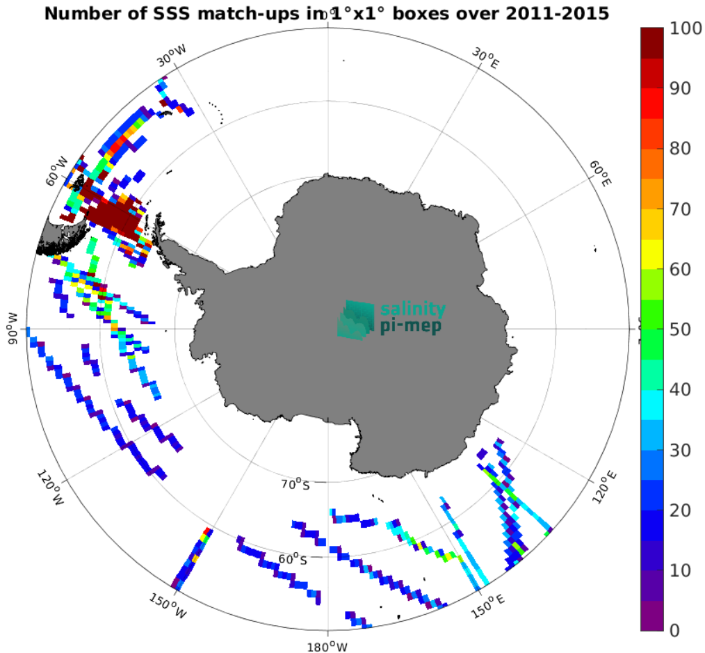
Figure 4: Number of SSS match-ups between TSG (SAMOS) SSS and the Aquarius SSS L4 OI v5 - Monthly (IPRC) SSS product for the Southern Ocean Pi-MEP region over 1^\circ \times 1^\circ boxes and for the full satellite product period.
